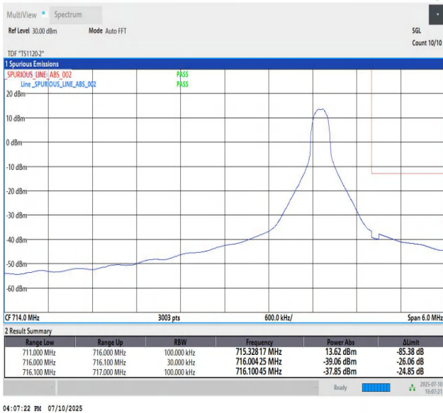
Band85_5MHz_QPSK_134157_1_High
