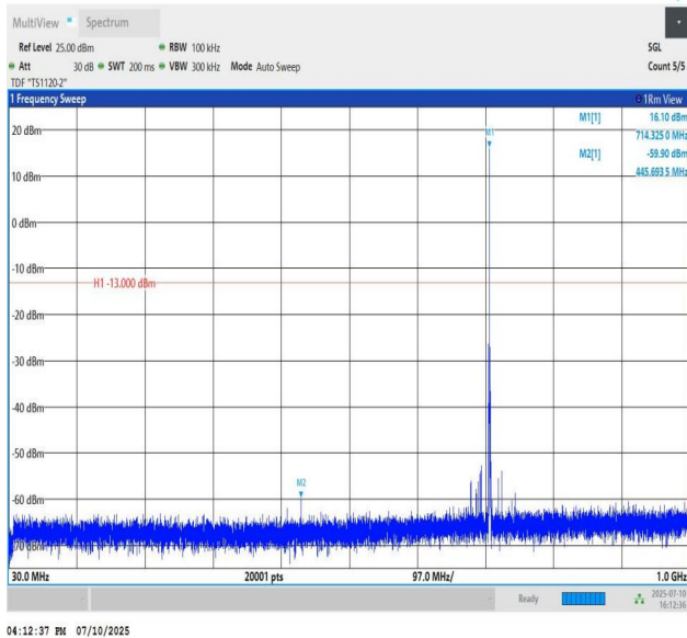
Band85-10MHz-QPSK-134132-PASS
