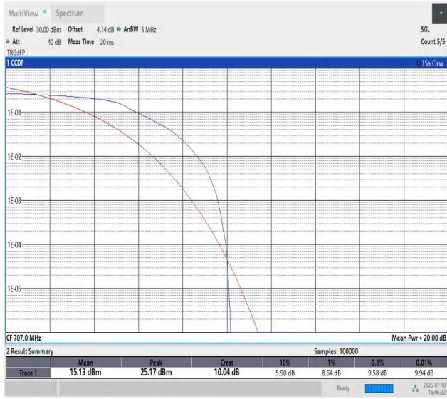
Band85-5MHz-16QAM-134092-PASS
