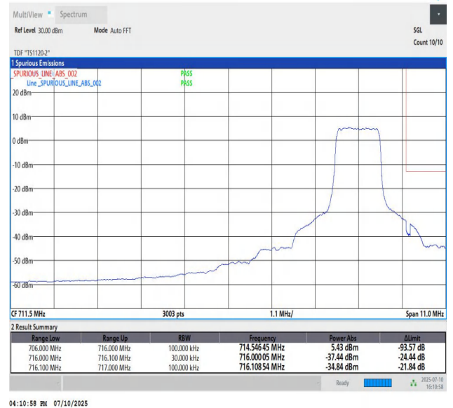
Band85_10MHz_QPSK_134132_6_High
