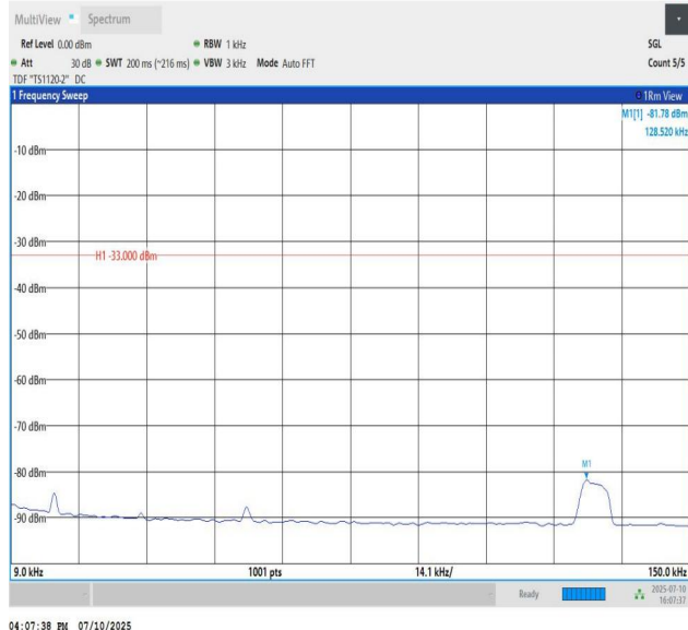
Band85-5MHz-QPSK-134027-PASS
