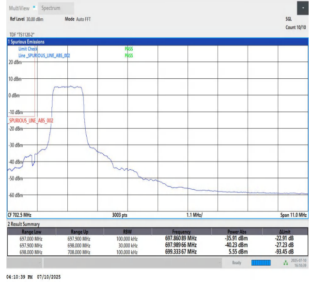
Band85_10MHz_QPSK_134052_6_Low
