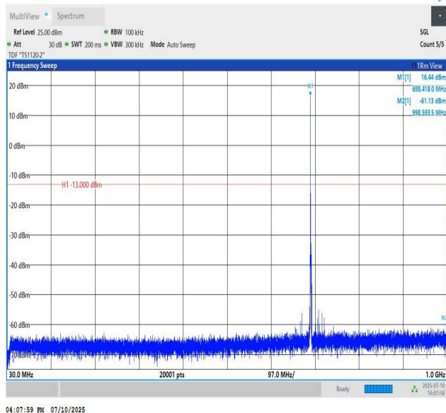
Band85-5MHz-QPSK-134027-PASS
