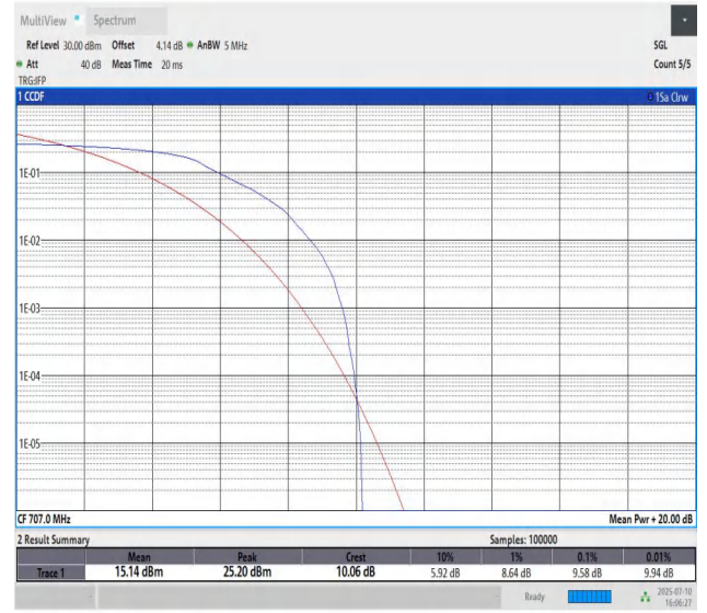
Band85-5MHz-QPSK-134092-PASS
