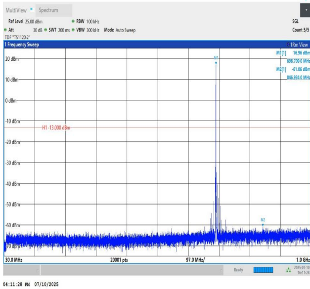
Band85-10MHz-QPSK-134052-PASS
