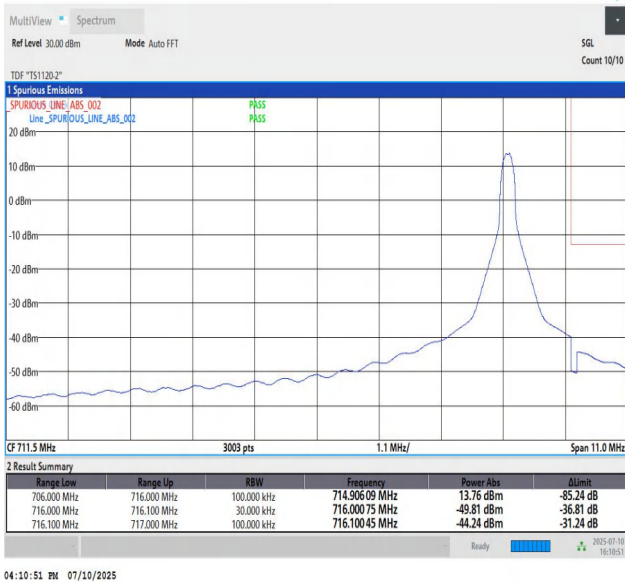
Band85_10MHz_QPSK_134132_1_High
