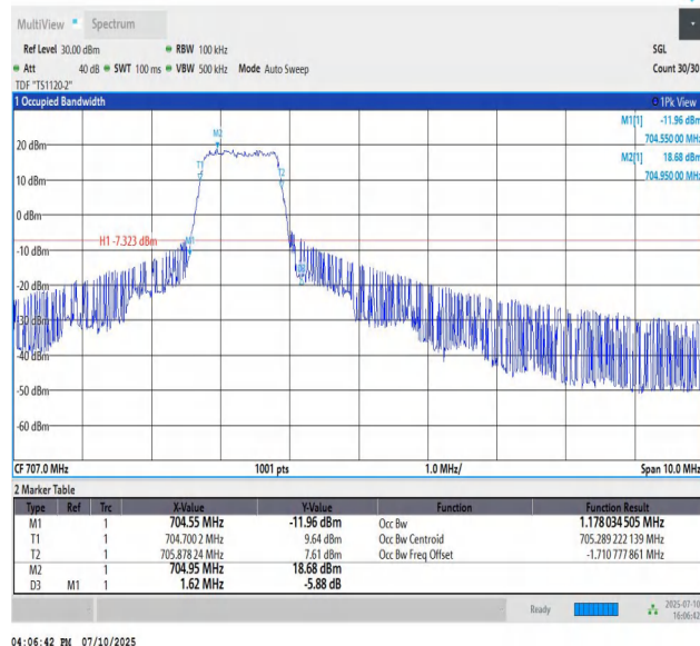
Band85-5MHz-QPSK-134092-PASS
