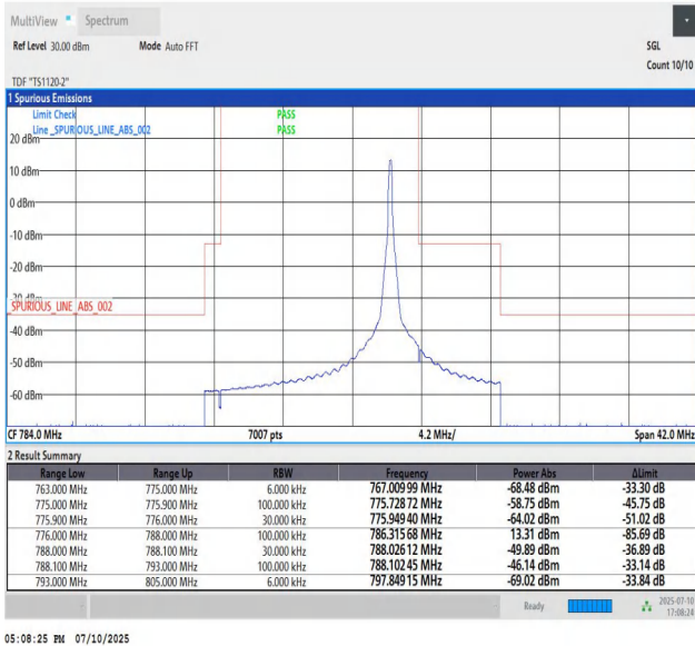
Band13_5MHz_QPSK_23255_1_High
