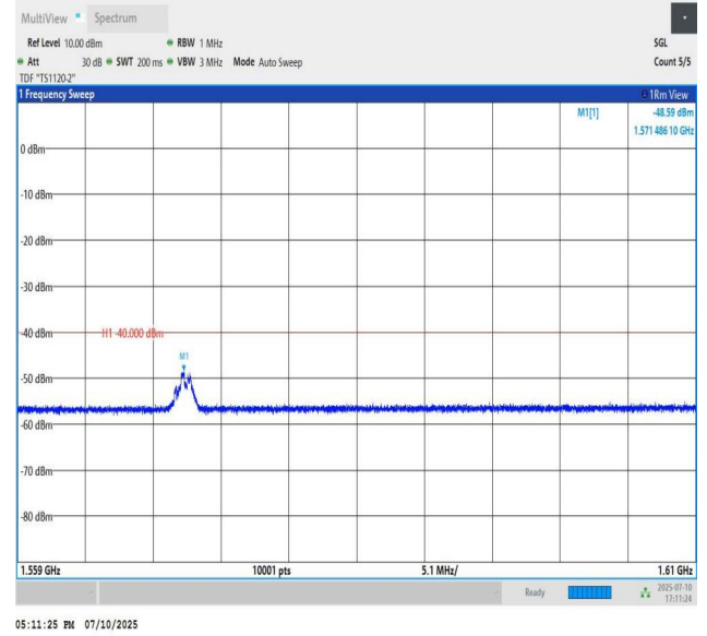
Band13-5MHz-QPSK-23255-PASS
