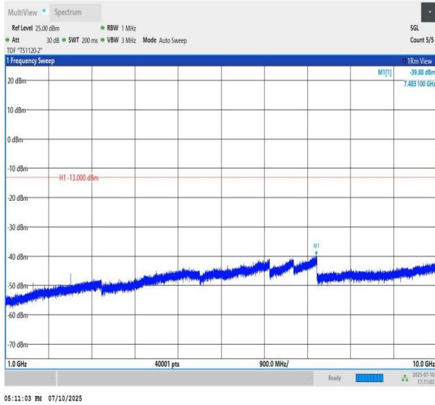
Band13-5MHz-QPSK-23255-PASS
