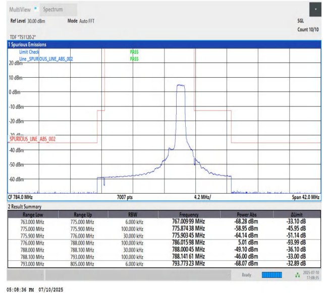
Band13_5MHz_QPSK_23255_6_High
