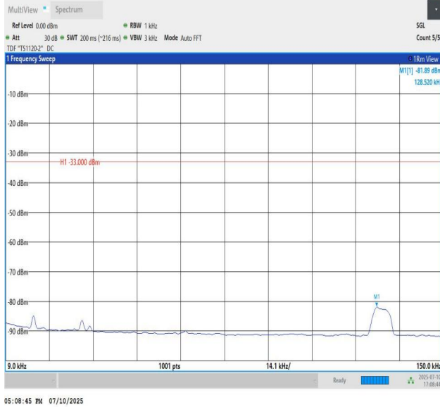
Band13-5MHz-QPSK-23205-PASS
