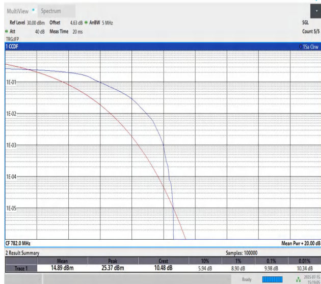
Band13-5MHz-16QAM-23230-PASS
