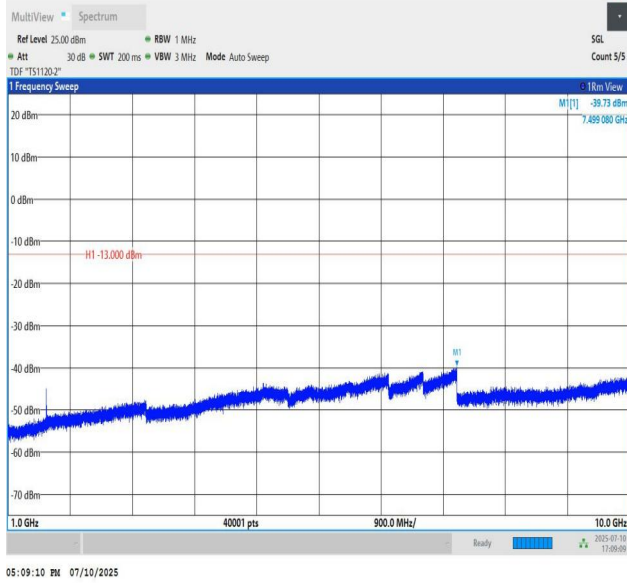
Band13-5MHz-QPSK-23205-PASS
