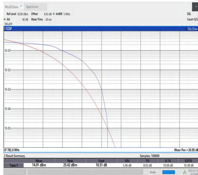
Band13-5MHz-QPSK-23230-PASS
