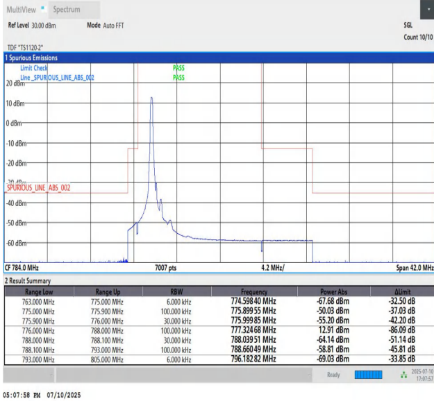
Band13_5MHz_QPSK_23205_1_Low
