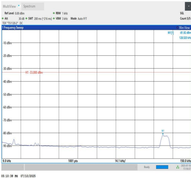
Band13-5MHz-QPSK-23255-PASS
