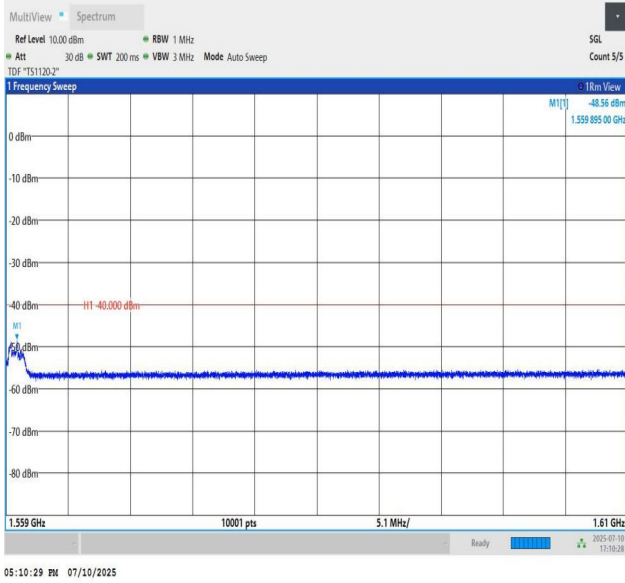
Band13-5MHz-QPSK-23230-PASS
