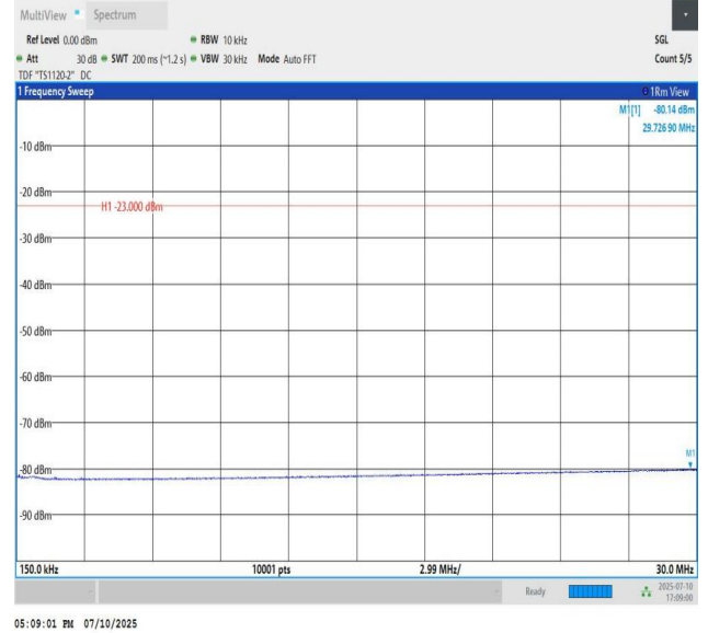
Band13-5MHz-QPSK-23205-PASS
