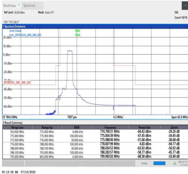
Band13_10MHz_QPSK_23230_6_Low
