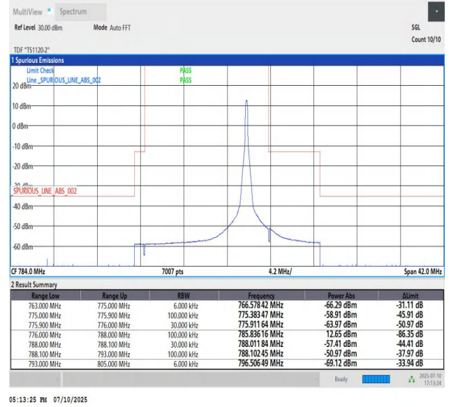
Band13_10MHz_QPSK_23230_1_High
