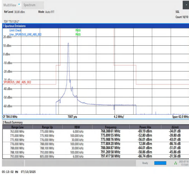
Band13_10MHz_QPSK_23230_1_Low
