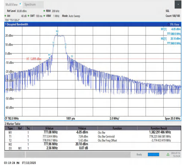
Band13-10MHz-QPSK-23230-PASS
