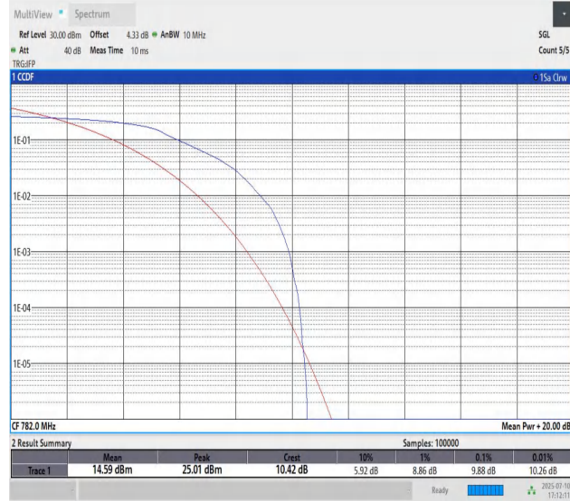
Band13-10MHz-QPSK-23230-PASS
