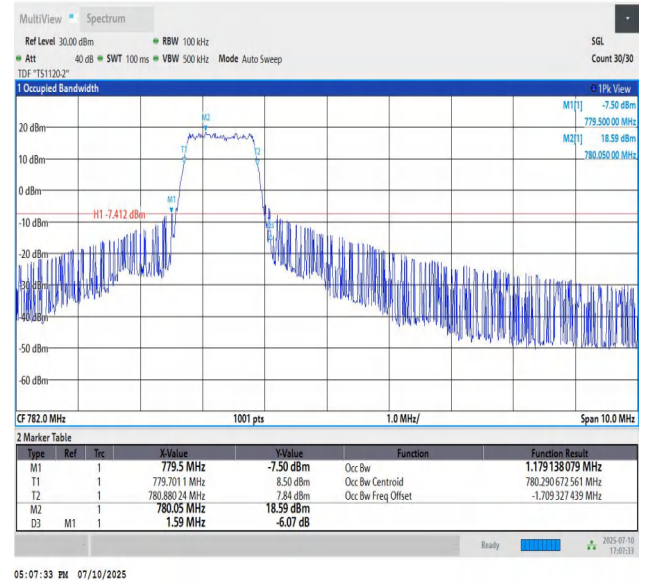
Band13-5MHz-QPSK-23230-PASS
