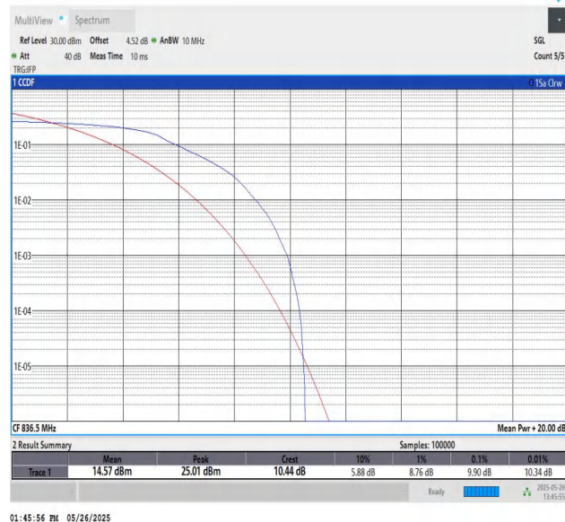
Band5-10MHz-16QAM-20525-PASS
