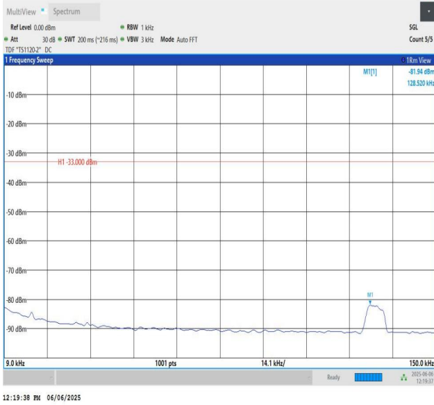
Band5-3MHz-QPSK-20415-PASS
