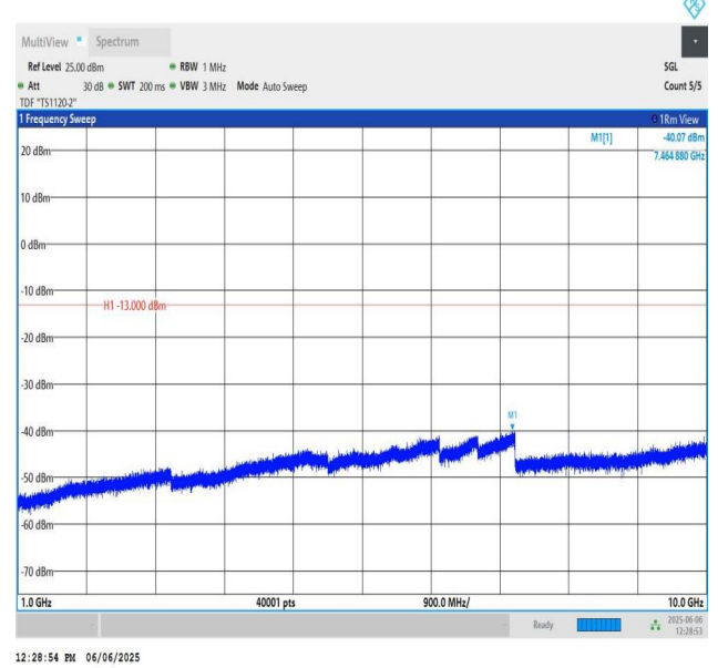
Band5-10MHz-QPSK-20525-PASS
