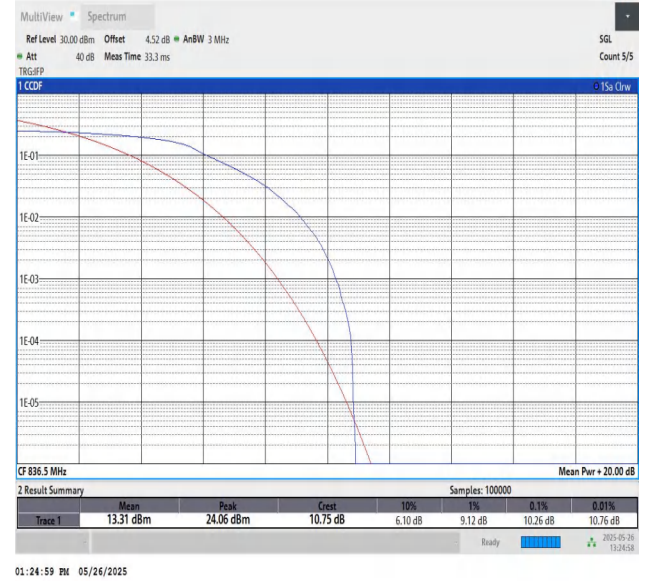
Band5-3MHz-16QAM-20525-PASS
