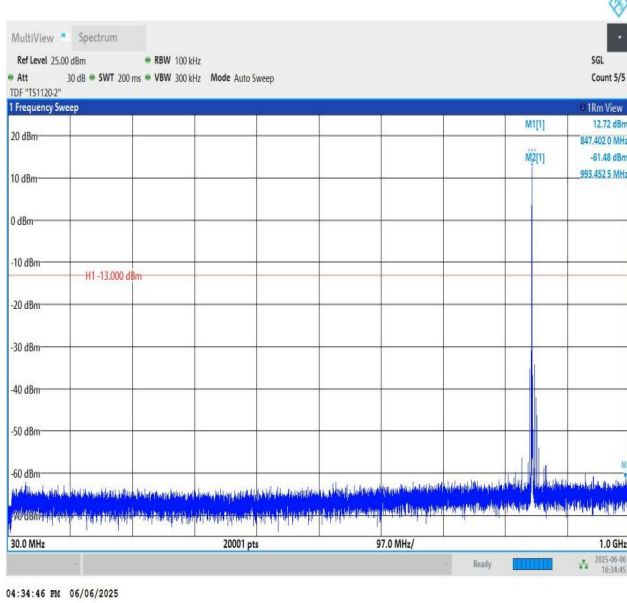
Band5-10MHz-QPSK-20525-PASS
