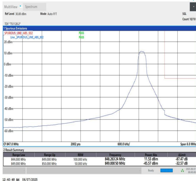
Band5_5MHz_QPSK_20625_1_High
