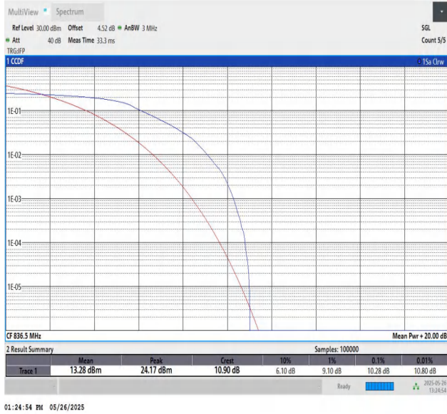
Band5-3MHz-QPSK-20525-PASS
