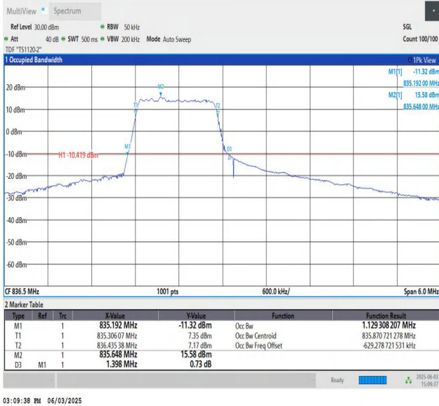
Band5-3MHz-QPSK-20525-PASS
