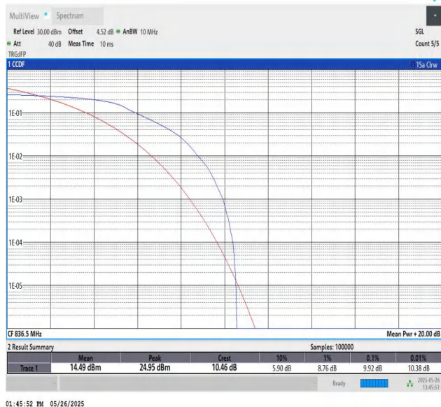
Band5-10MHz-QPSK-20525-PASS
