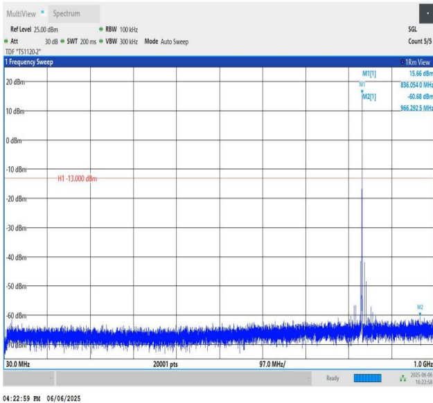
Band5-1.4MHz-QPSK-20525-PASS
