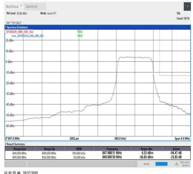
Band5_5MHz_QPSK_20625_6_High
