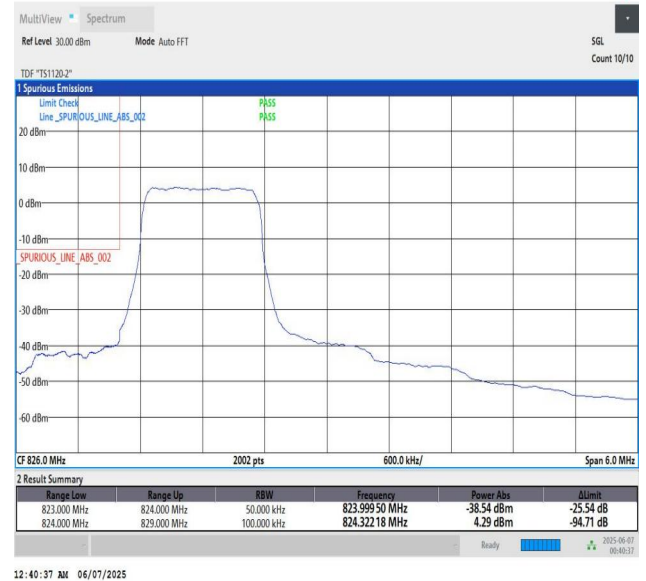
Band5_5MHz_QPSK_20425_6_Low
