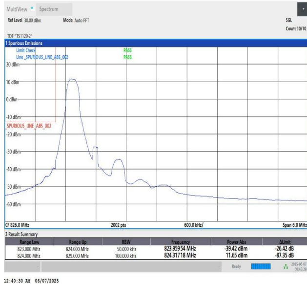
Band5_5MHz_QPSK_20425_1_Low
