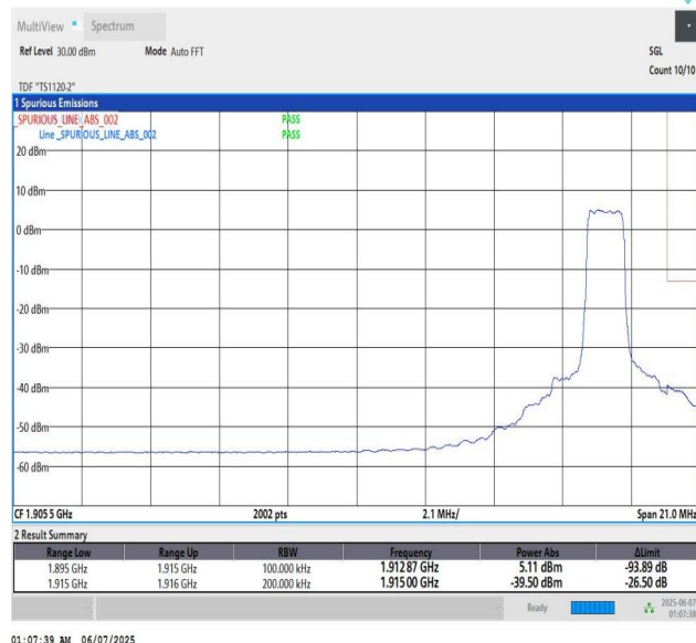
Band25_20MHz_QPSK_26590_6_High
