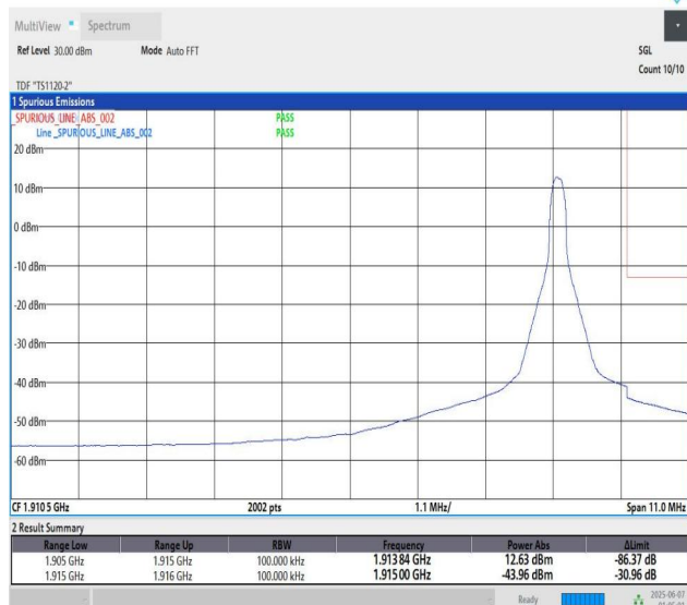
Band25_10MHz_QPSK_26640_1_High
