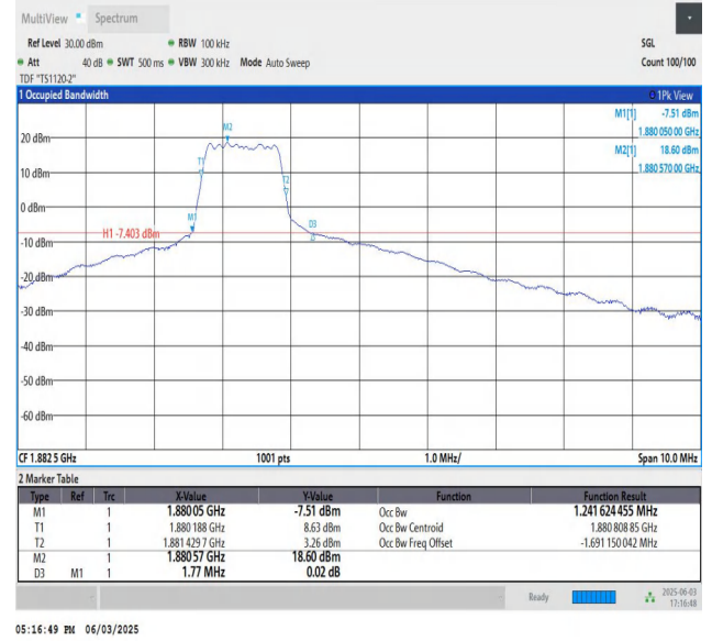
Band25-5MHz-16QAM-26365-PASS
