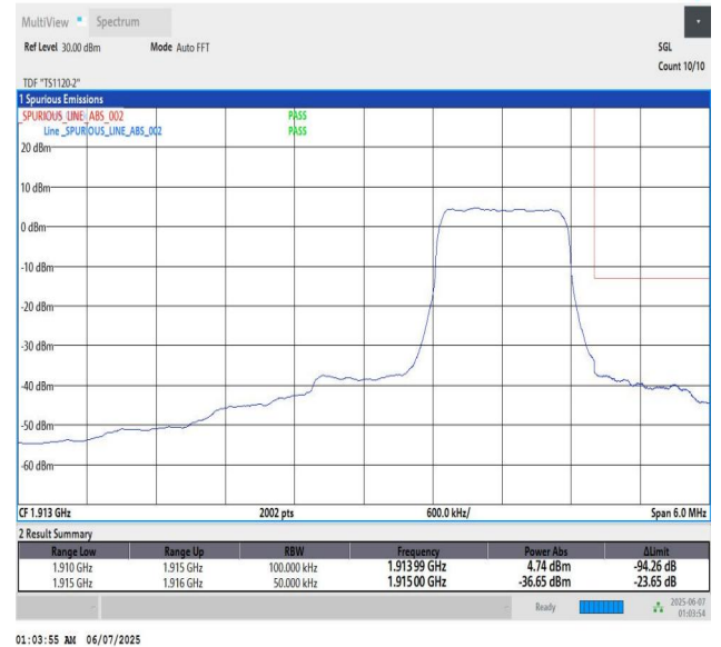
Band25_5MHz_QPSK_26665_6_High
