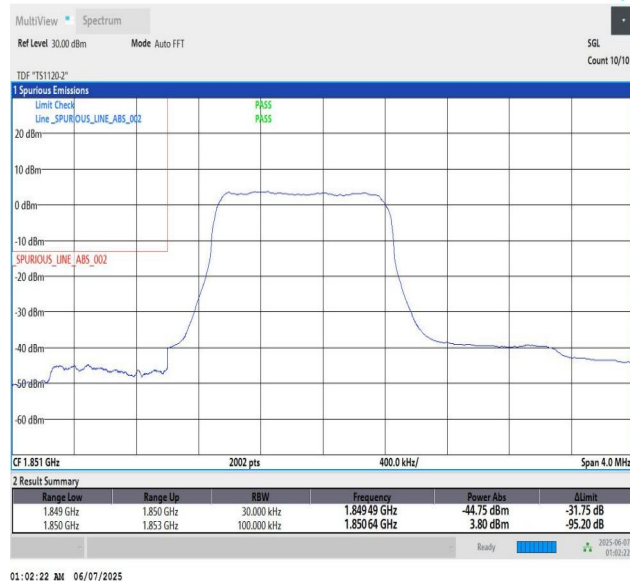
Band25_3MHz_QPSK_26055_6_Low
