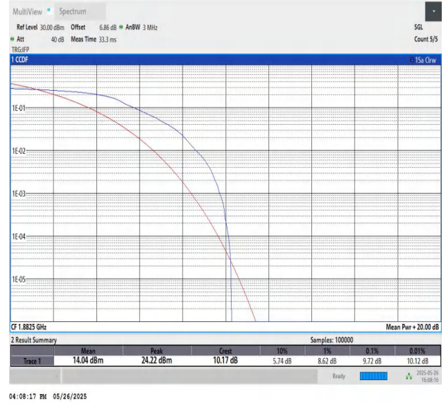
Band25-3MHz-16QAM-26365-PASS
