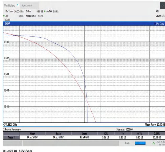
Band25-5MHz-16QAM-26365-PASS
