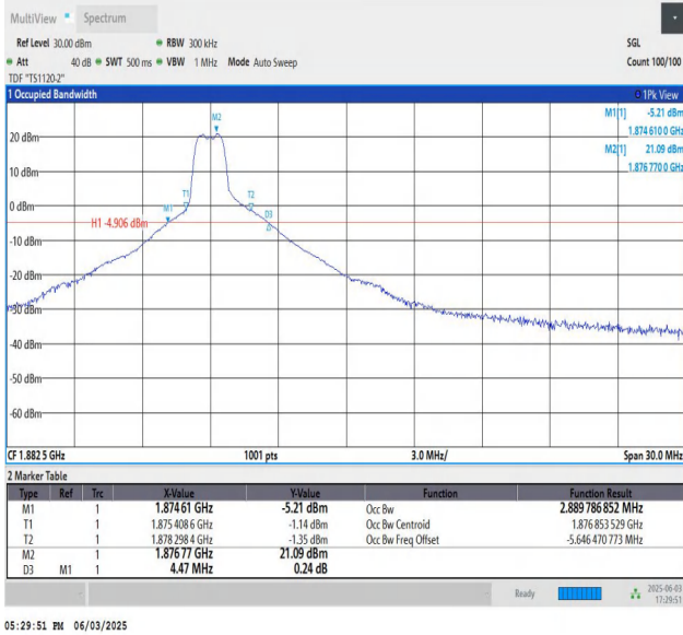
Band25-15MHz-QPSK-26365-PASS
