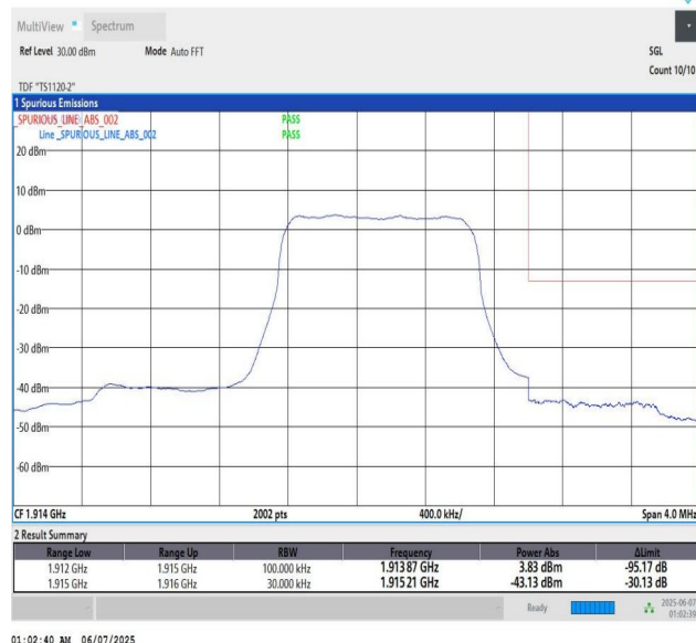
Band25_3MHz_QPSK_26675_6_High
