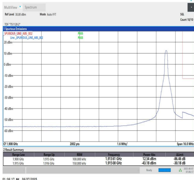
Band25_15MHz_QPSK_26615_1_High
