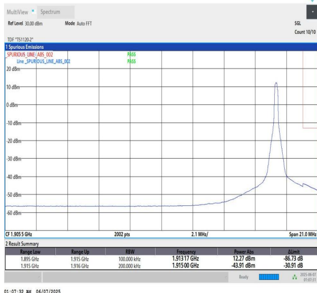
Band25_20MHz_QPSK_26590_1_High
