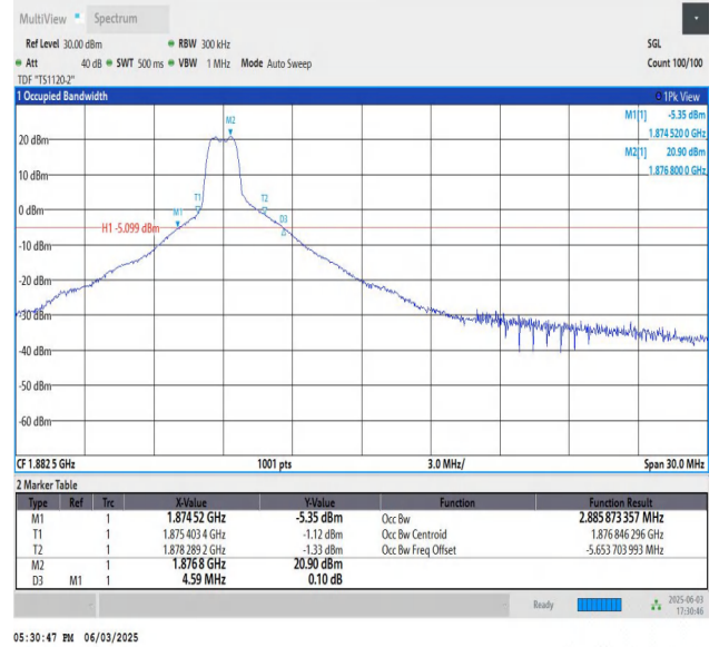
Band25-15MHz-16QAM-26365-PASS
