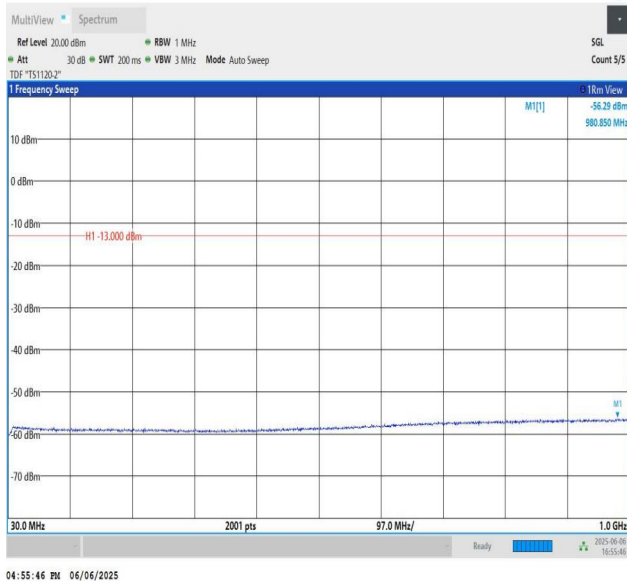
Band25-1.4MHz-QPSK-26047-PASS
