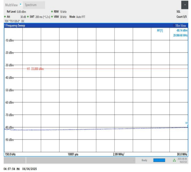
Band25-3MHz-QPSK-26055-PASS
