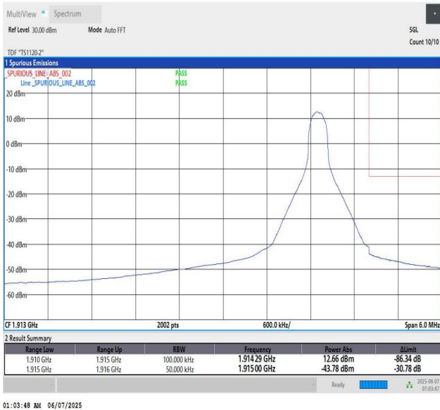
Band25_5MHz_QPSK_26665_1_High
