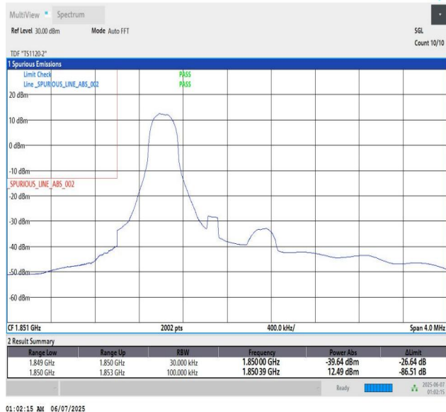
Band25_3MHz_QPSK_26055_1_Low
