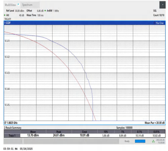
Band25-1.4MHz-16QAM-26365-PASS
