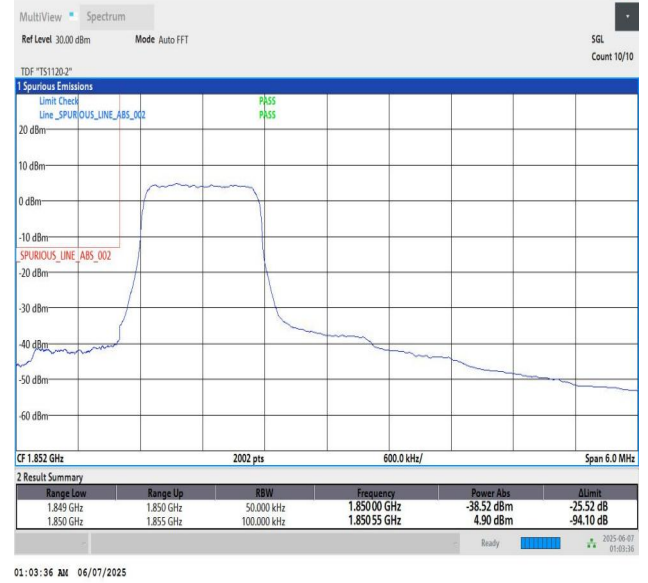
Band25_5MHz_QPSK_26065_6_Low
