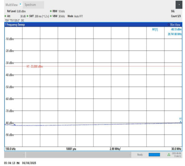
Band25-15MHz-QPSK-26115-PASS
