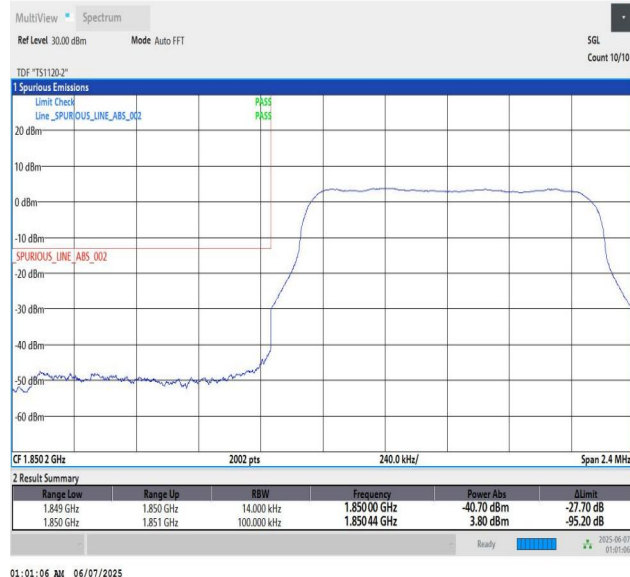
Band25_1.4MHz_QPSK_26047_6_Low
