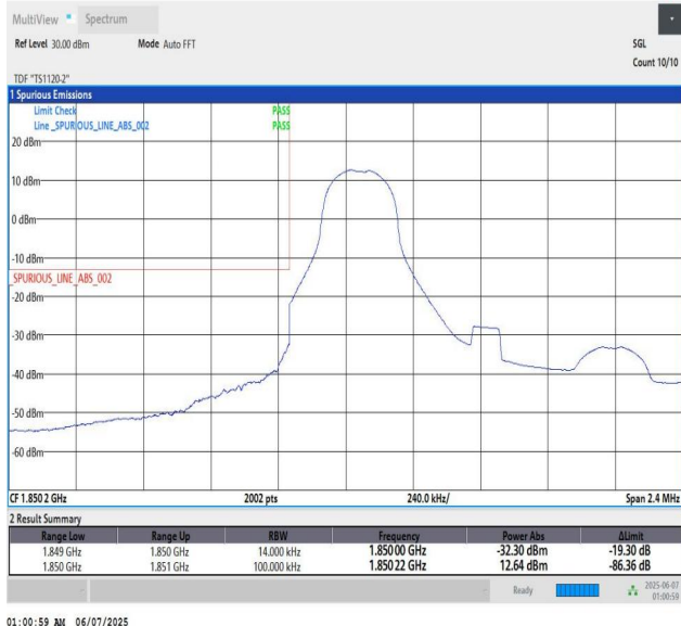
Band25_1.4MHz_QPSK_26047_1_Low
