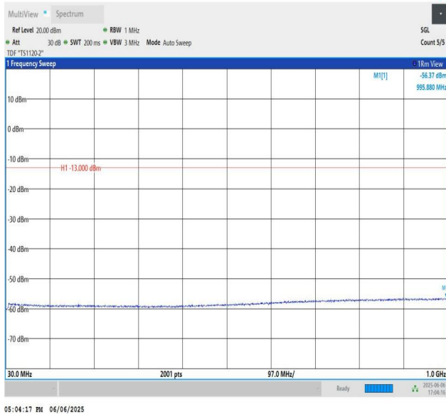
Band25-15MHz-QPSK-26115-PASS
