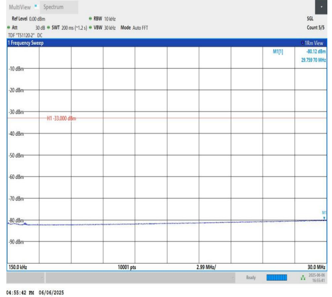
Band25-1.4MHz-QPSK-26047-PASS
