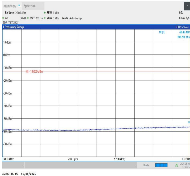
Band25-15MHz-QPSK-26615-PASS
