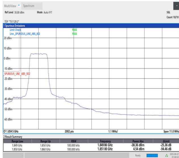
Band25_10MHz_QPSK_26090_6_Low
