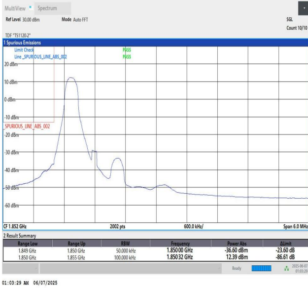
Band25_5MHz_QPSK_26065_1_Low
