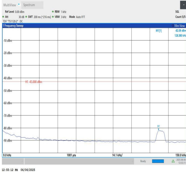
Band25-3MHz-QPSK-26055-PASS
