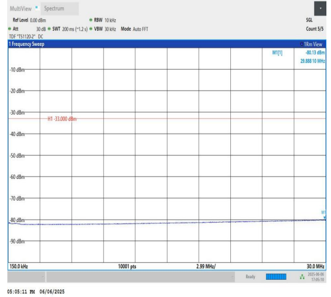
Band25-15MHz-QPSK-26615-PASS
