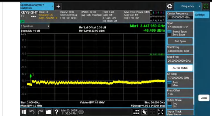
Band66-15MHz-QPSK-132047-1RB#74-3000~20000-PASS
