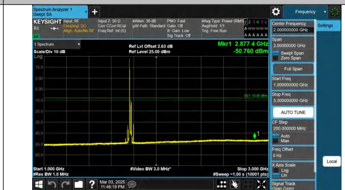
Band66-20MHz-QPSK-132572-1RB#0-1000~3000-PASS
