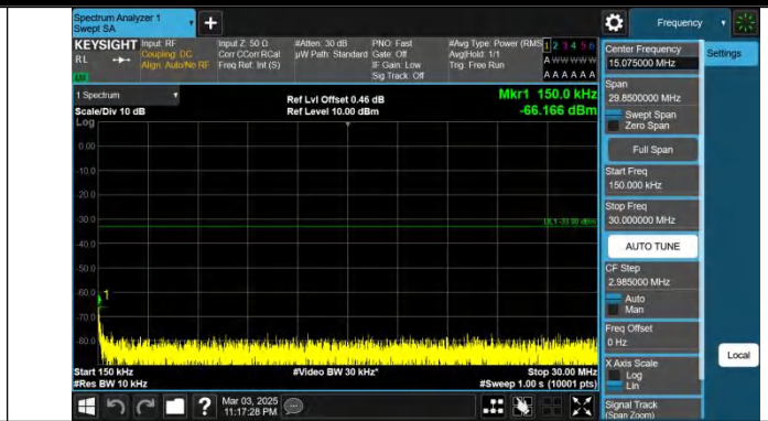
Band66-5MHz-QPSK-132647-1RB#0-0.15~30-PASS
