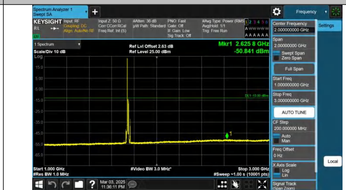
Band66-15MHz-QPSK-132322-1RB#0-1000~3000-PASS
