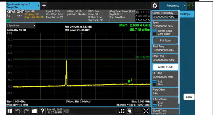
Band66-10MHz-QPSK-132622-1RB#0-1000~3000-PASS
