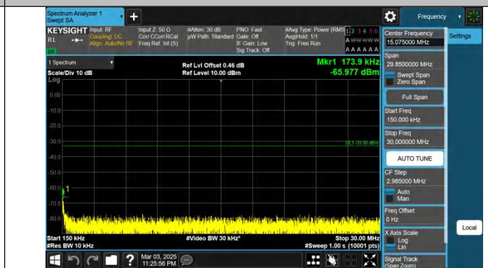
Band66-10MHz-QPSK-132322-1RB#0-0.15~30-PASS
