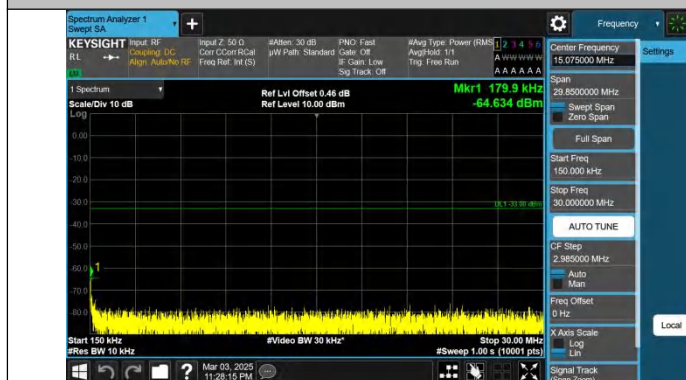
Band66-10MHz-QPSK-132622-1RB#49-0.15~30-PASS
