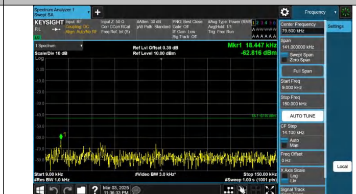
Band66-15MHz-QPSK-132322-1RB#74-0.009~0.15-PASS
