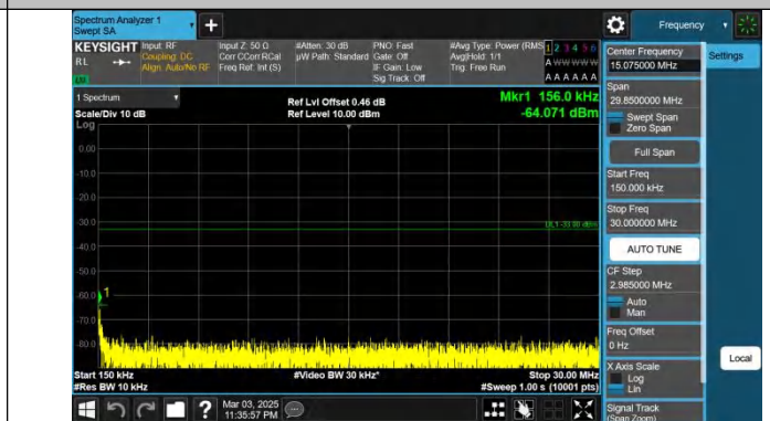
Band66-15MHz-QPSK-132322-1RB#0-0.15~30-PASS
