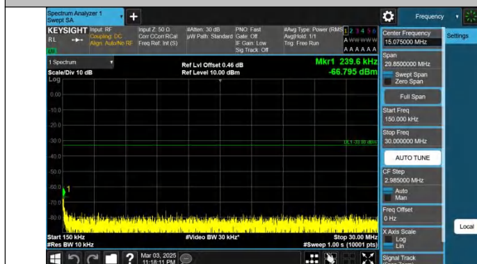
Band66-5MHz-QPSK-132647-1RB#24-0.15~30-PASS
