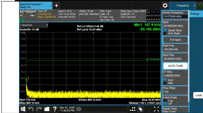
Band66-15MHz-QPSK-132322-1RB#74-0.15~30-PASS
