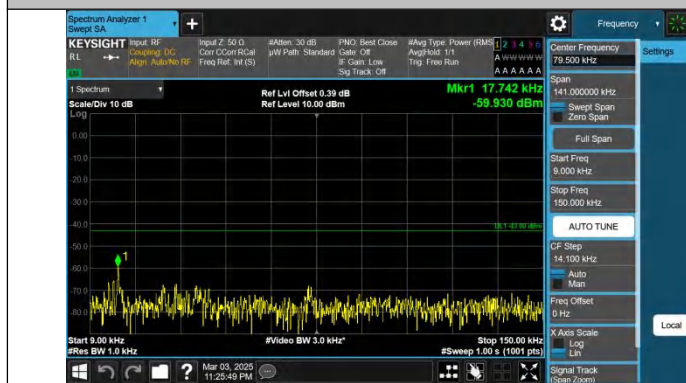
Band66-10MHz-QPSK-132322-1RB#0-0.009~0.15-PASS
