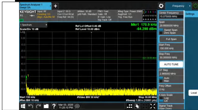
Band66-10MHz-QPSK-132022-1RB#49-0.15~30-PASS
