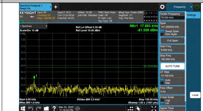
Band66-5MHz-QPSK-132647-1RB#24-0.009~0.15-PASS
