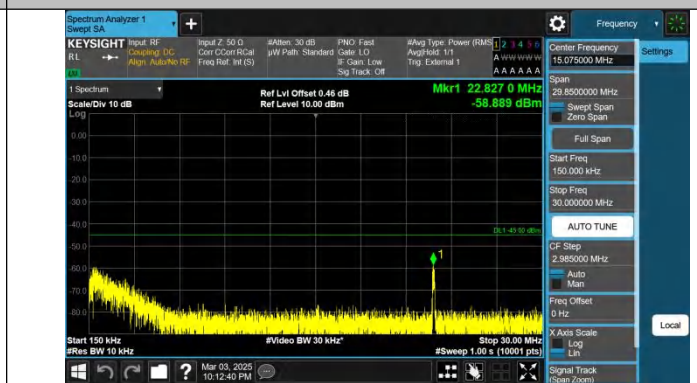
Band41-20MHz-QPSK-40620-1RB#0-0.15~30-PASS
