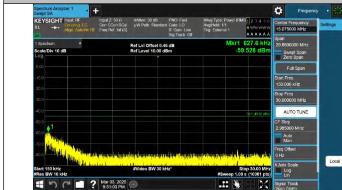
Band41-15MHz-QPSK-40620-1RB#74-0.15~30-PASS
