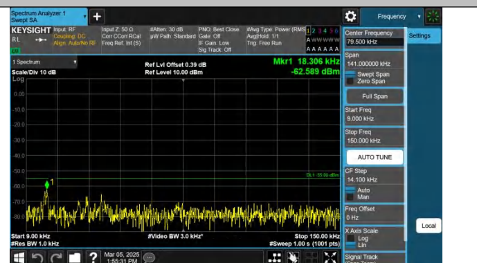
Band41-20MHz-QPSK-39750-1RB#99-0.009~0.15-PASS
