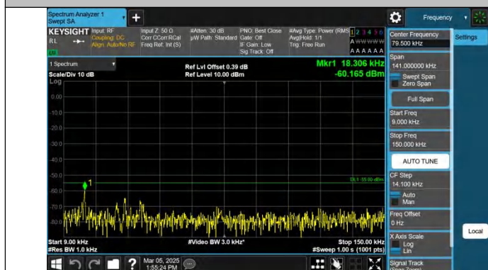
Band41-20MHz-QPSK-39750-1RB#0-0.009~0.15-PASS
