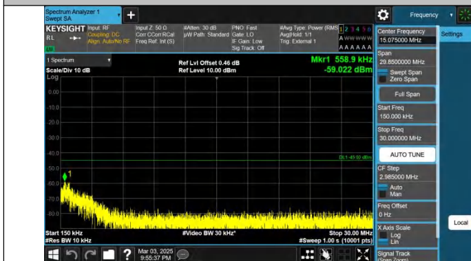
Band41-15MHz-QPSK-41515-1RB#74-0.15~30-PASS
