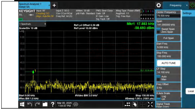
Band41-15MHz-QPSK-41515-1RB#0-0.009~0.15-PASS
