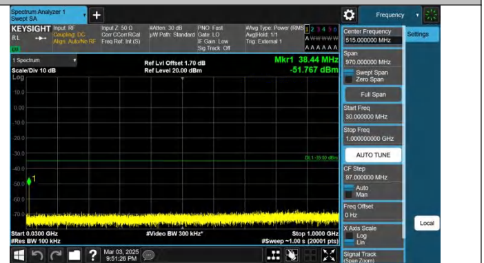
Band41-15MHz-QPSK-40620-1RB#74-30~1000-PASS
