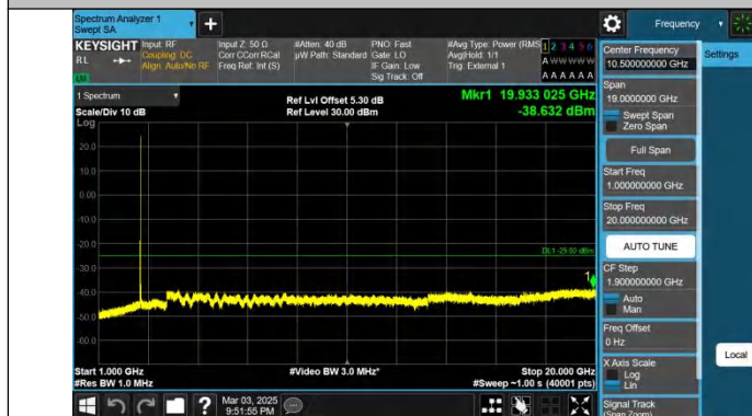
Band41-15MHz-QPSK-40620-1RB#74-1000~20000-PASS
