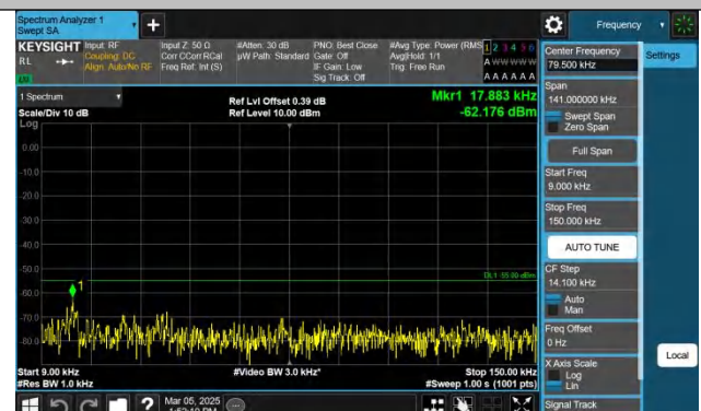
Band41-5MHz-QPSK-40620-1RB#24-0.009~0.15-PASS
