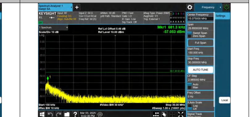
Band41-5MHz-QPSK-41565-1RB#0-0.15~30-PASS
