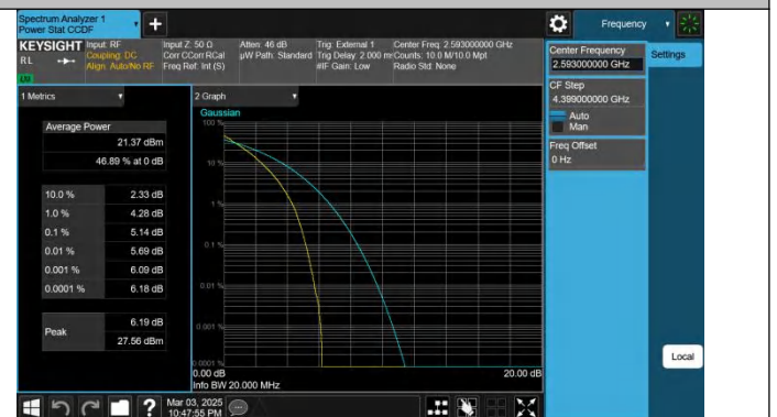
Band41-20MHz-QPSK-40620-100RB#0-PASS
