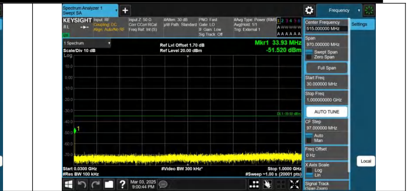
Band41-5MHz-QPSK-40620-1RB#24-30~1000-PASS
