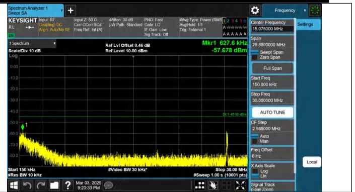
Band41-10MHz-QPSK-40620-1RB#0-0.15~30-PASS
