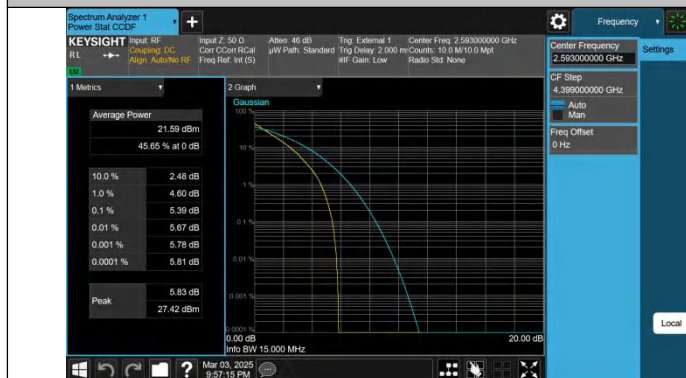
Band41-15MHz-QPSK-40620-75RB#0-PASS
