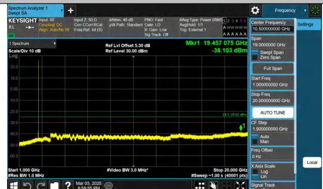
Band41-5MHz-QPSK-40620-1RB#0-1000~20000-PASS
