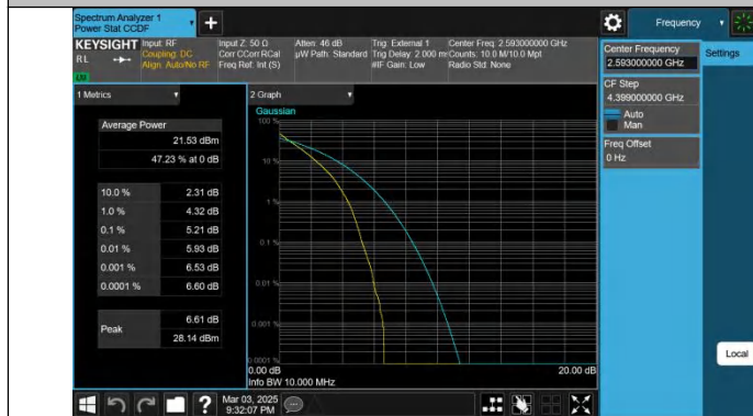
Band41-10MHz-QPSK-40620-50RB#0-PASS
