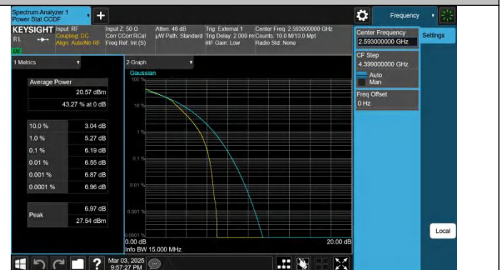
Band41-15MHz-16QAM-40620-75RB#0-PASS
