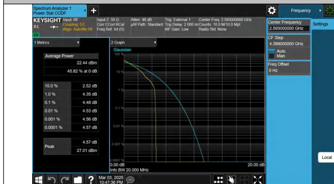
Band41-20MHz-QPSK-40620-1RB#0-PASS
