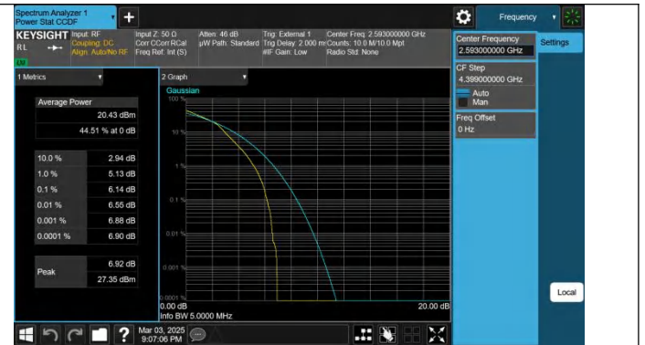
Band41-5MHz-16QAM-40620-25RB#0-PASS
