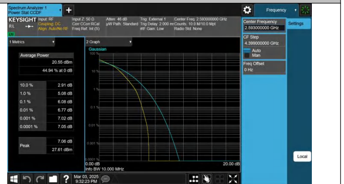
Band41-10MHz-16QAM-40620-50RB#0-PASS
