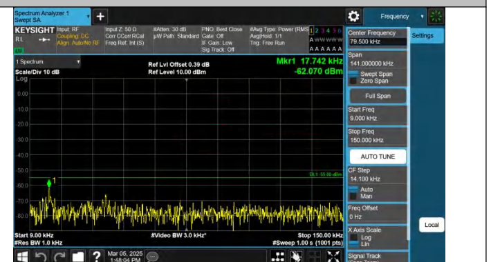
Band38-10MHz-QPSK-38200-1RB#49-0.009~0.15-PASS
