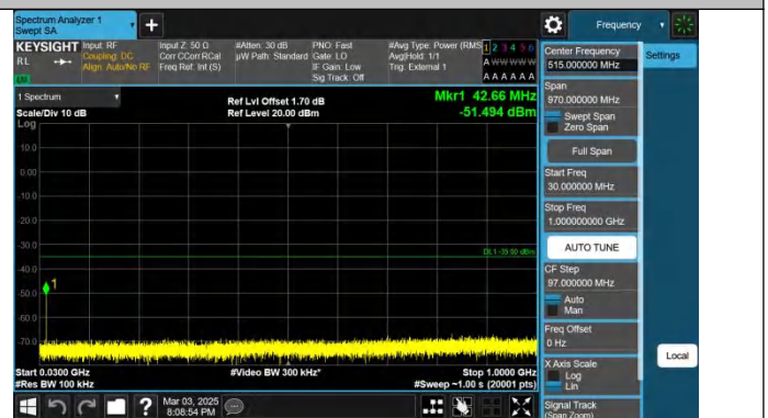
Band38-20MHz-QPSK-38000-1RB#99-30~1000-PASS
