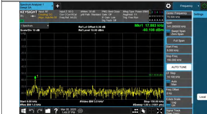
Band38-20MHz-QPSK-37850-1RB#0-0.009~0.15-PASS
