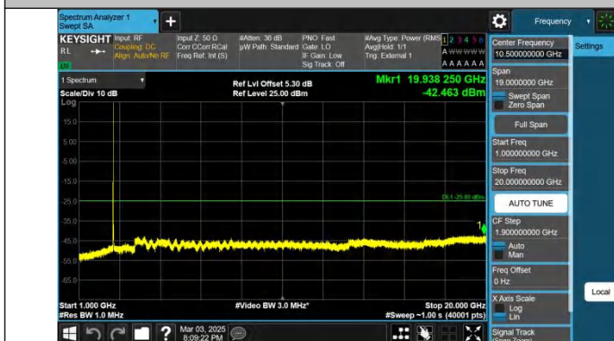
Band38-20MHz-QPSK-38000-1RB#99-1000~20000-PASS
