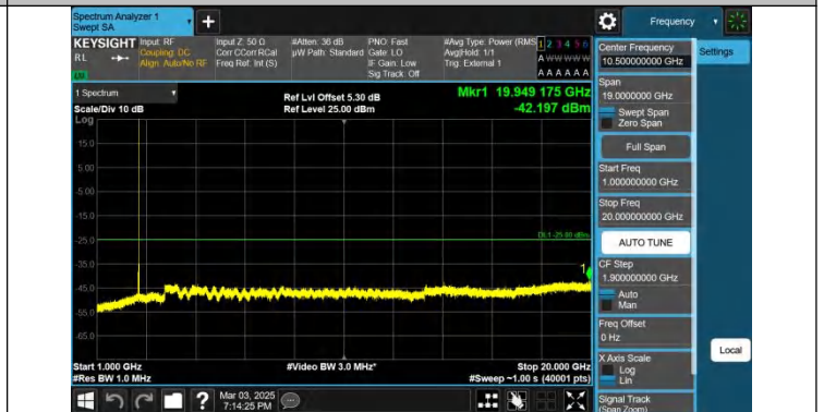
Band38-10MHz-QPSK-38000-1RB#0-1000~20000-PASS
