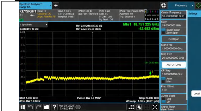
Band38-15MHz-QPSK-38175-1RB#74-1000~20000-PASS
