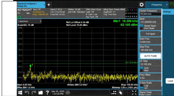
Band38-10MHz-QPSK-38000-1RB#0-0.009~0.15-PASS
