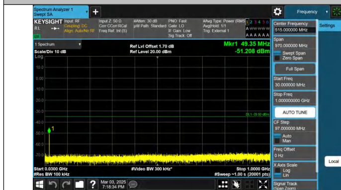
Band38-10MHz-QPSK-38200-1RB#0-30~1000-PASS
