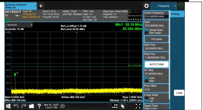
Band38-10MHz-QPSK-38200-1RB#49-30~1000-PASS
