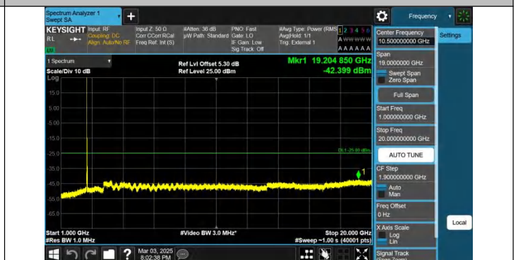
Band38-20MHz-QPSK-37850-1RB#0-1000~20000-PASS
