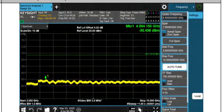
Band26(824-849)-5MHz-QPSK-26815-1RB#24-3000~10000-PASS
