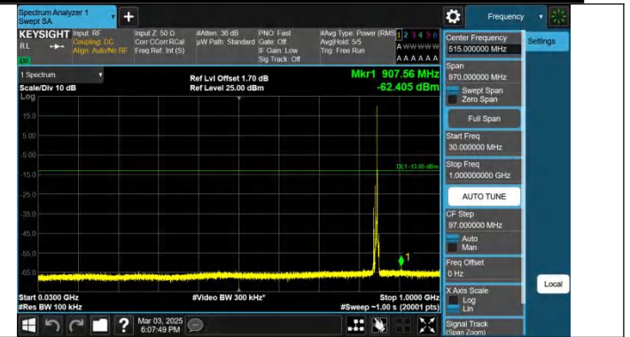
Band26(824-849)-5MHz-QPSK-27015-1RB#24-30~1000-PASS
