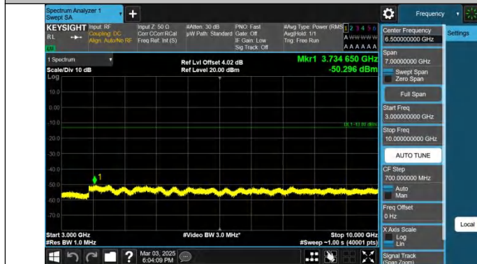
Band26(824-849)-5MHz-QPSK-26815-1RB#0-3000~10000-PASS
