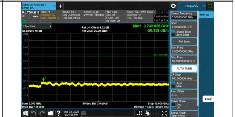
Band26(824-849)-15MHz-QPSK-26865-1RB#74-3000~10000-PAS
