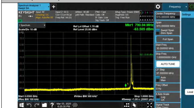
Band26(824-849)-15MHz-QPSK-26915-1RB#0-30~1000-PASS
