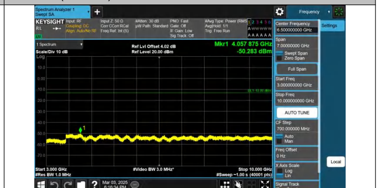
Band26(824-849)-10MHz-QPSK-26915-1RB#49-3000~10000-PASS S
