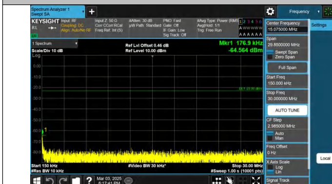
Band26(824-849)-10MHz-QPSK-26990-1RB#49-0.15~30-PASS
