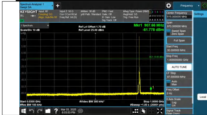
Band26(824-849)-5MHz-QPSK-26815-1RB#0-30~1000-PASS
