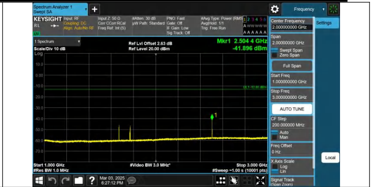
Band26(824-849)-15MHz-QPSK-26965-1RB#0-1000~3000-PASS
