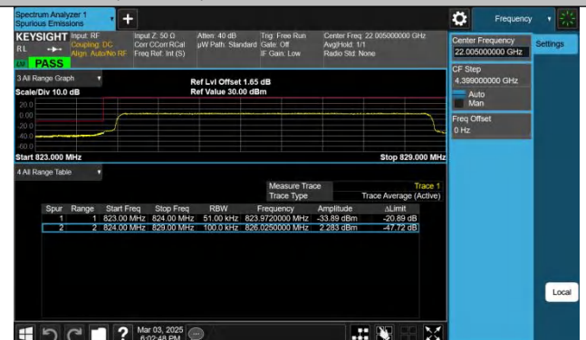
Band26(824-849)-5MHz-QPSK-26815-25RB#0-PASS
