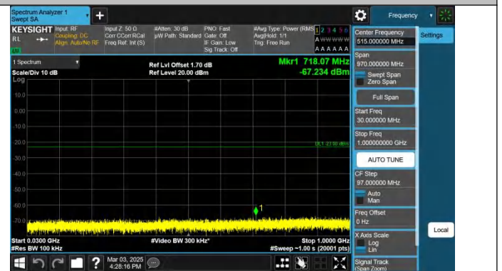
Band25-5MHz-QPSK-26365-1RB#24-30~1000-PASS
