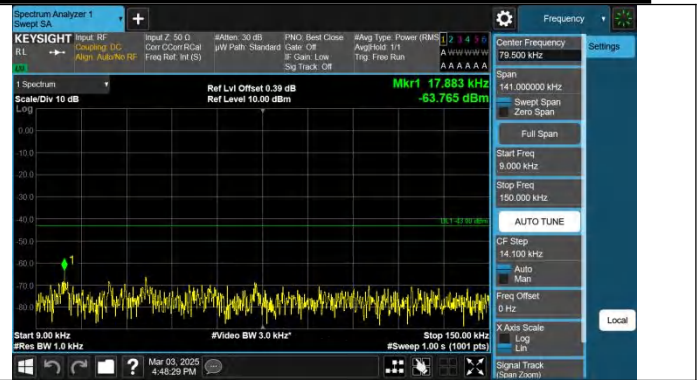
Band25-15MHz-QPSK-26615-1RB#74-0.009~0.15-PASS
