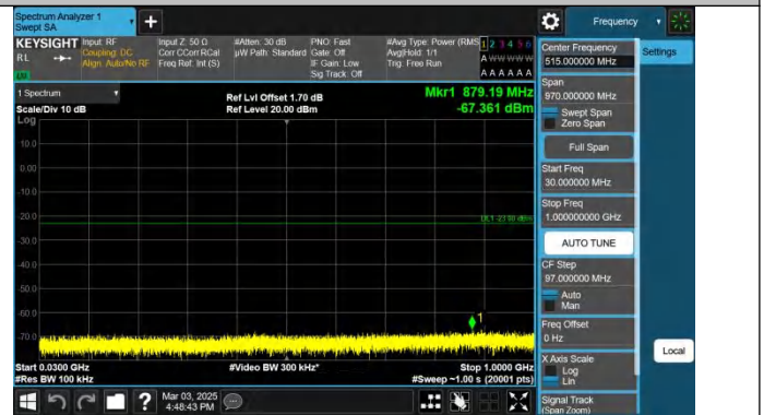
Band25-15MHz-QPSK-26615-1RB#74-30~1000-PASS
