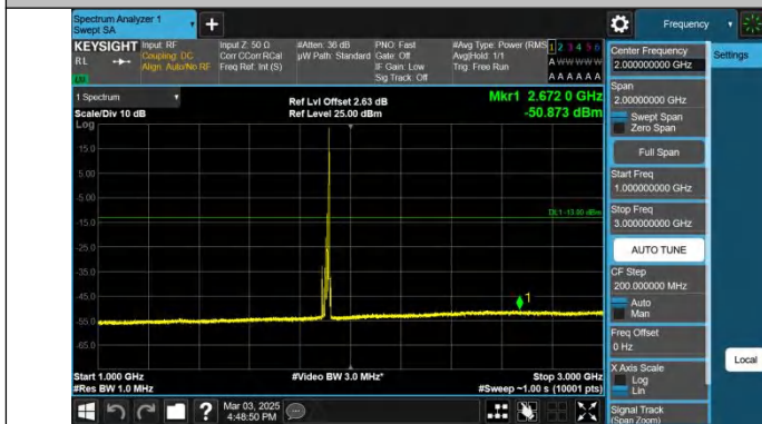
Band25-15MHz-QPSK-26615-1RB#74-1000~3000-PASS
