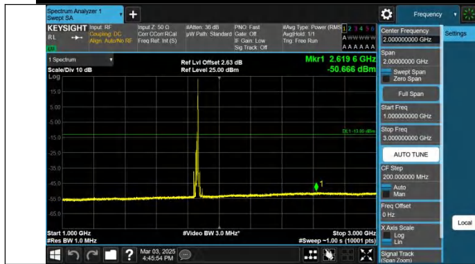
Band25-15MHz-QPSK-26115-1RB#74-1000~3000-PASS
