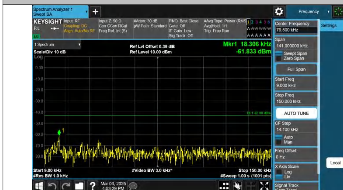
Band25-20MHz-QPSK-26140-1RB#0-0.009~0.15-PASS
