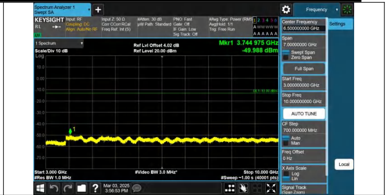
Band13-10MHz-QPSK-23230-1RB#0-3000~10000-PASS
