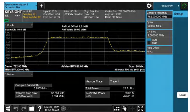
Band13-10MHz-16QAM-23230-50RB#0-PASS
