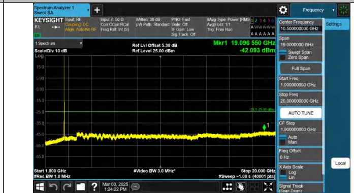
Band7-15MHz-QPSK-21375-1RB#0-1000~20000-PASS
