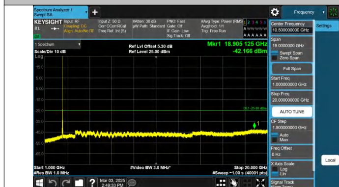
Band7-20MHz-QPSK-20850-1RB#99-1000~20000-PASS
