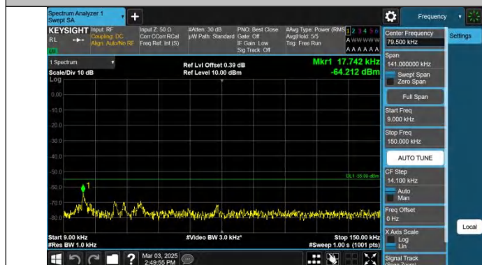
Band7-20MHz-QPSK-21100-1RB#0-0.009~0.15-PASS
