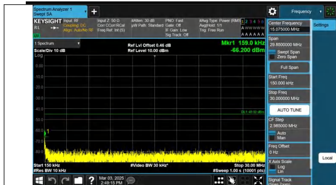
Band7-20MHz-QPSK-20850-1RB#99-0.15~30-PASS
