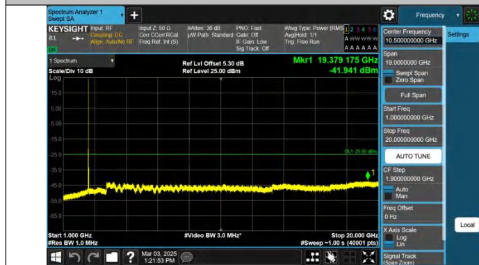
Band7-15MHz-QPSK-20825-1RB#74-1000~20000-PASS
