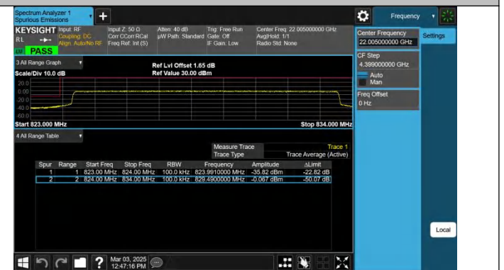
Band5-10MHz-QPSK-20450-50RB#0-PASS
