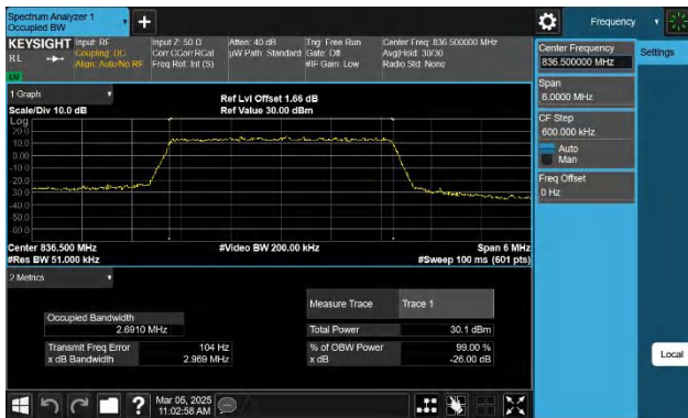
Band5-3MHz-QPSK-20525-15RB#0-PASS
