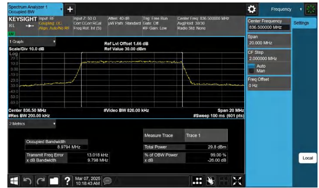
Band5-10MHz-16QAM-20525-50RB#0-PASS
