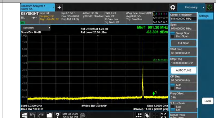
Band5-3MHz-QPSK-20415-1RB#14-30~1000-PASS
