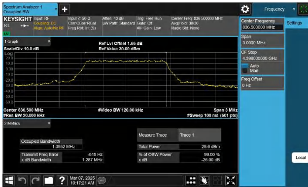
Band5-1.4MHz-QPSK-20525-6RB#0-PASS
