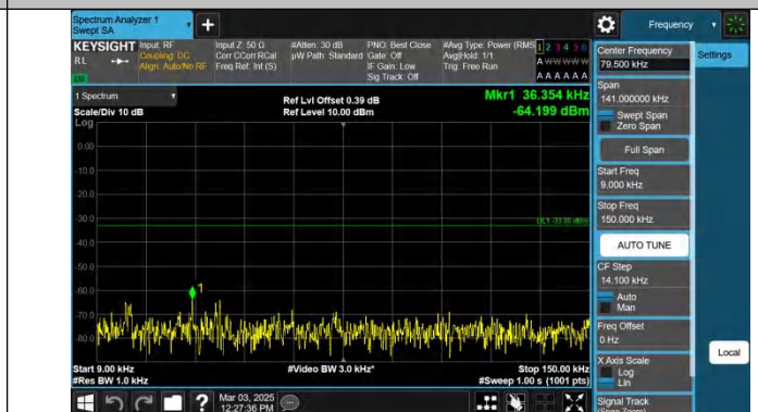
Band5-3MHz-QPSK-20415-1RB#14-0.009~0.15-PASS
