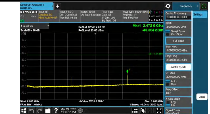
Band5-3MHz-QPSK-20415-1RB#0-1000~3000-PASS
