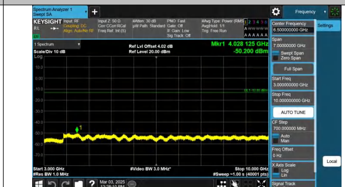
Band5-3MHz-QPSK-20415-1RB#14-3000~10000-PASS
