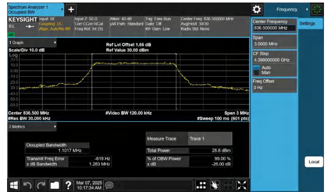
Band5-1.4MHz-16QAM-20525-6RB#0-PASS
