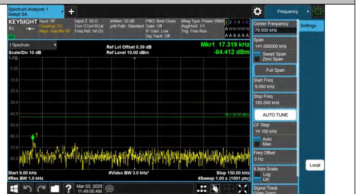
Band4-10MHz-QPSK-20350-1RB#49-0.009~0.15-PASS
