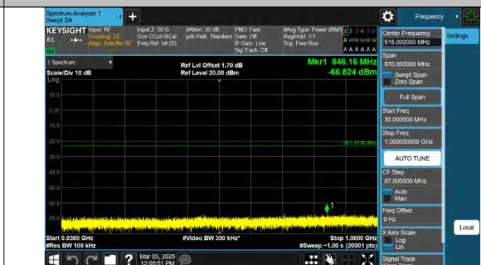
Band4-20MHz-QPSK-20175-1RB#99-30~1000-PASS
