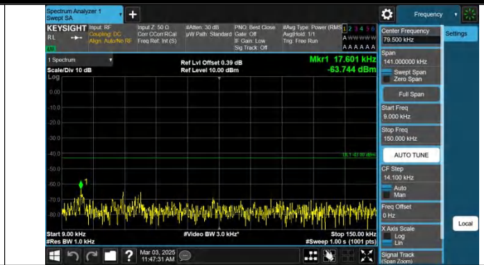
Band4-10MHz-QPSK-20175-1RB#49.0.009~0.15-PASS
