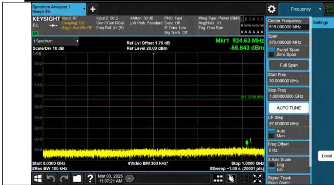
Band4-5MHz-QPSK-20175-1RB#0-30~1000-PASS
