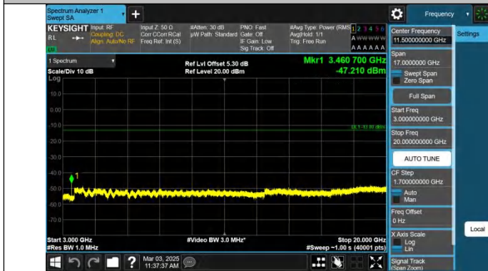
Band4-5MHz-QPSK-20175-1RB#0-3000~20000-PASS
