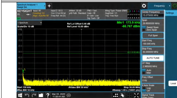
Band4-15MHz-QPSK-20325-1RB#74-0.15~30-PASS
