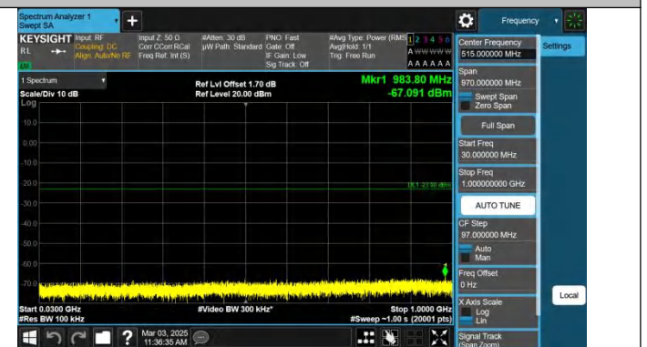
Band4-5MHz-QPSK-19975-1RB#24-30~1000-PASS
