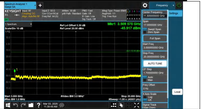
Band4-5MHz-QPSK-20375-1RB#24-3000~20000-PASS
