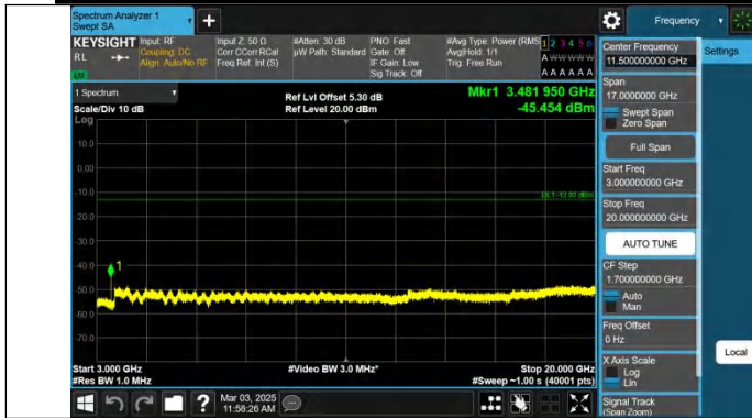
Band4-15MHz-QPSK-20325-1RB#0-3000~20000-PASS
