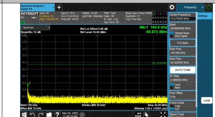
Band4-10MHz-QPSK-20350-1RB#0.0.15~30-PASS
