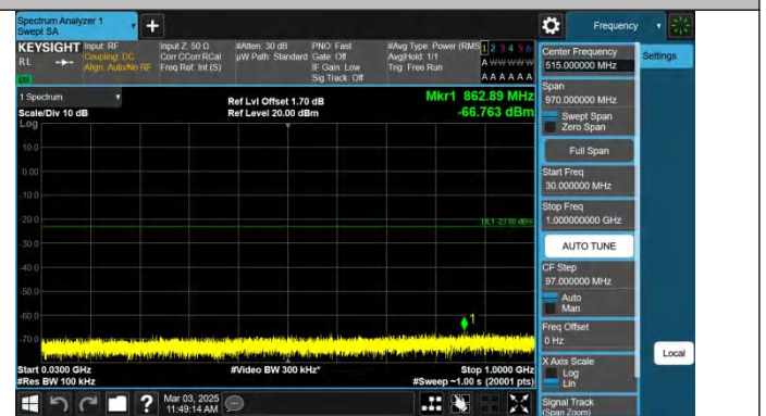
Band4-10MHz-QPSK-20350-1RB#49-30~1000-PASS
