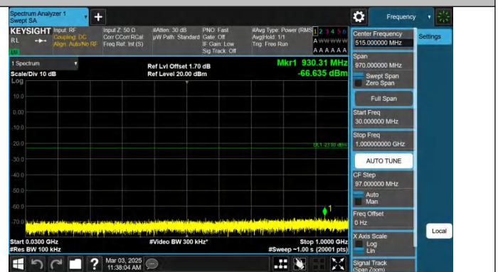
Band4-5MHz-QPSK-20175-1RB#24-30~1000-PASS
