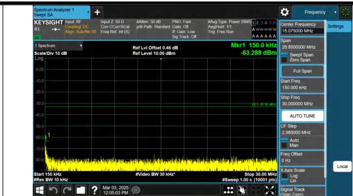
Band4-20MHz-QPSK-20175-1RB#0-0.15~30-PASS
