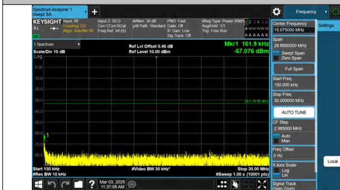
Band4-5MHz-QPSK-20175-1RB#24-0.15~30-PASS
