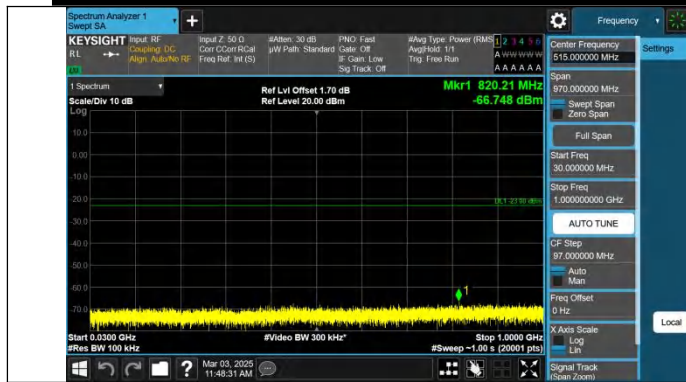
Band4-10MHz-QPSK-20350-1RB#0-30~1000-PASS
