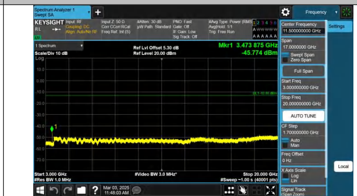
Band4-10MHz-QPSK-20175-1RB#49.3000~20000-PASS
