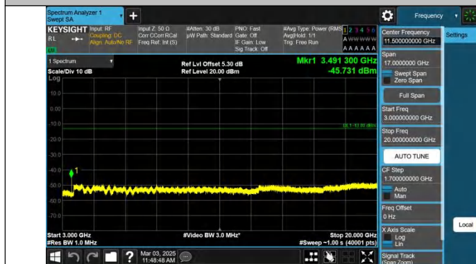
Band4-10MHz-QPSK-20350-1RB#0-3000~20000-PASS
