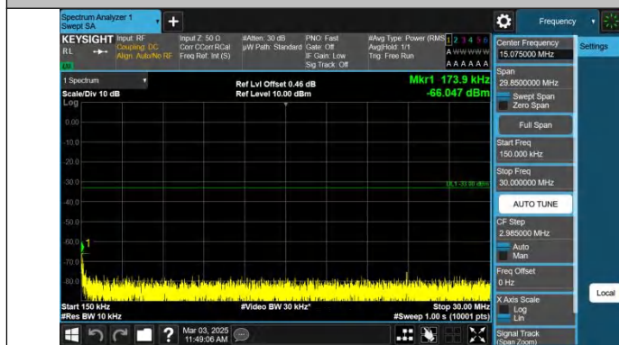
Band4-10MHz-QPSK-20350-1RB#49-0.15~30-PASS
