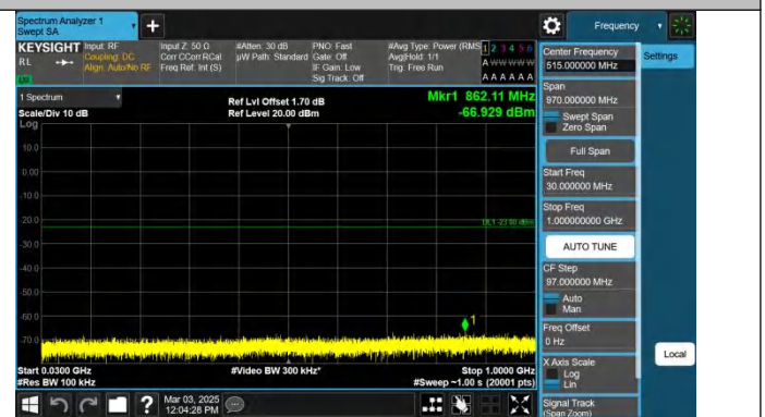
Band4-20MHz-QPSK-20050-1RB#99-30~1000-PASS
