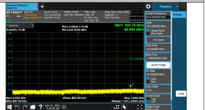
Band4-15MHz-QPSK-20325-1RB#74-30~1000-PASS
