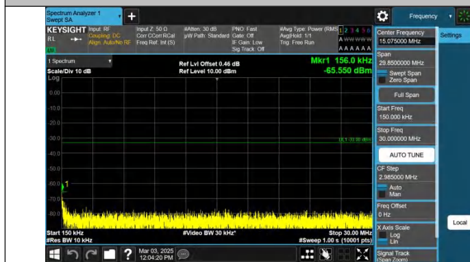
Band4-20MHz-QPSK-20050-1RB#99-0.15~30-PASS
