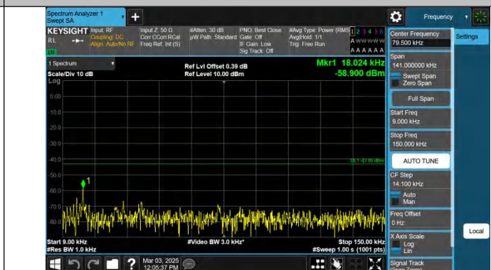
Band4-20MHz-QPSK-20175-1RB#99-0.009~0.15-PASS
