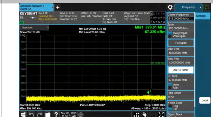
Band2-20MHz-QPSK-18900-1RB#99-30~1000-PASS
