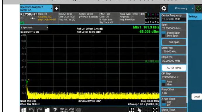
Band2-10MHz-QPSK-19150-1RB#49-0.15~30-PASS
