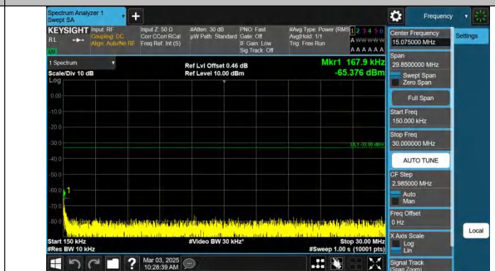
Band2-3MHz-QPSK-19185-1RB#0.15~30-PASS
