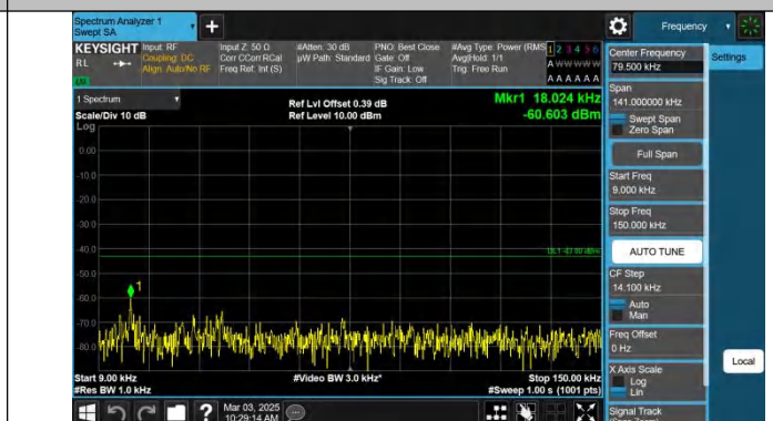
Band2-3MHz-QPSK-19185-1RB#14-0.009~0.15-PASS
