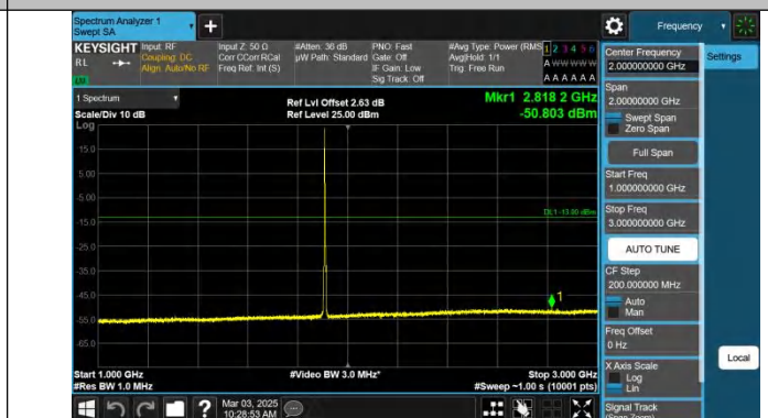
Band2-3MHz-QPSK-19185-1RB#0-1000~3000-PASS
