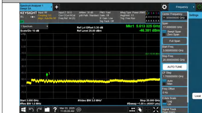
Band2-20MHz-QPSK-18900-1RB#0-3000~20000-PASS
