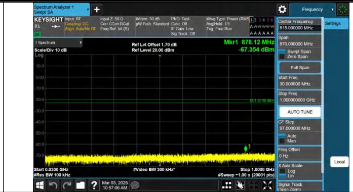
Band2-15MHz-QPSK-18900-1RB#74-30~1000-PASS
