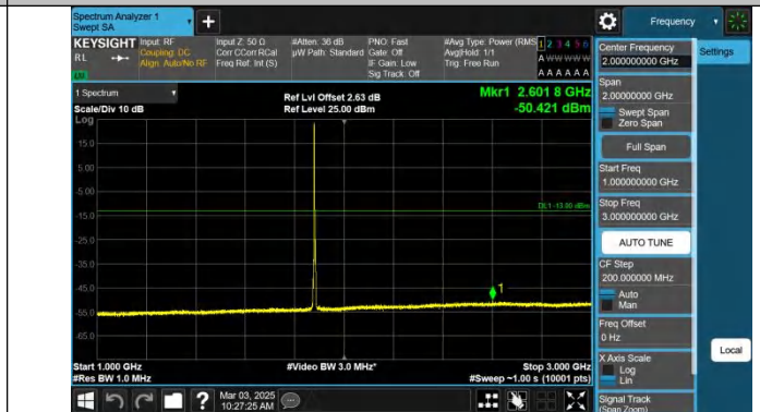
Band2-3MHz-QPSK-18900-1RB#0-1000~3000-PASS
