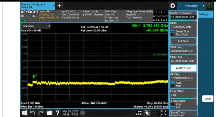
Band2-3MHz-QPSK-18900-1RB#14-3000~20000-PASS
