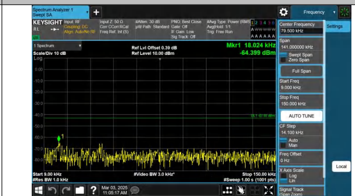
Band2-20MHz-QPSK-18900-1RB#99-0.009~0.15-PASS
