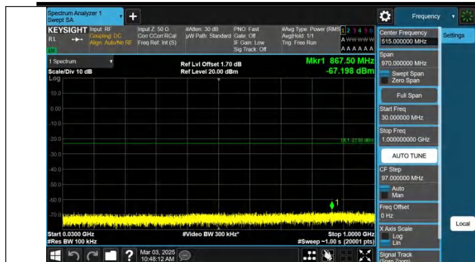
Band2-10MHz-QPSK-19150-1RB#0-30~1000-PASS
