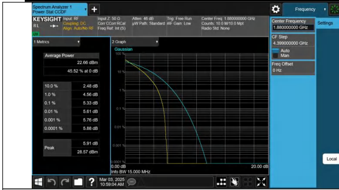
Band2-15MHz-QPSK-18900-75RB#0-PASS
