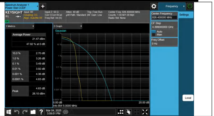
Band5-4132-2-PASS
