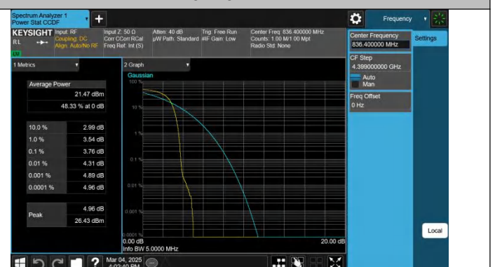
Band5-4182-4-PASS
