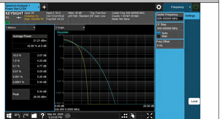
Band5-4132-4-PASS
