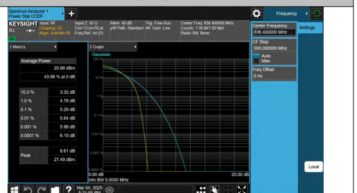
Band5-4182-3-PASS
