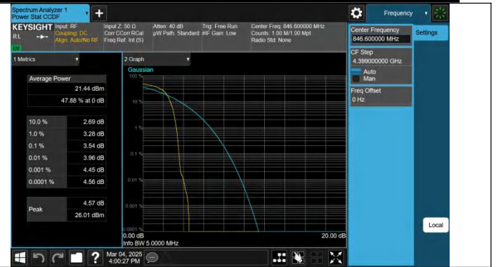
Band5-4233-2-PASS
