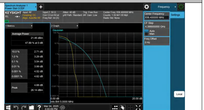
Band5-4182-2-PASS
