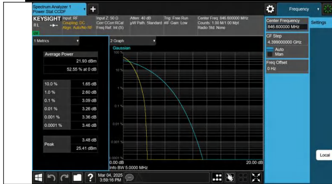
Band5-4233-1-PASS
