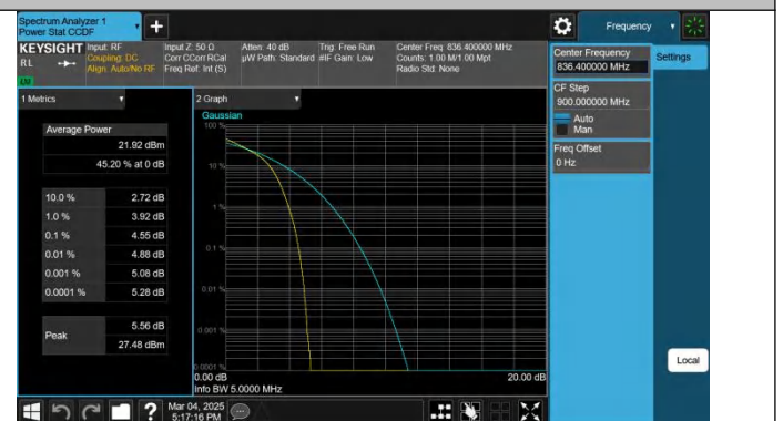
Band5-4182-1-PASS
