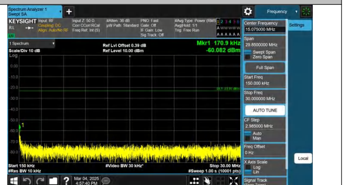
Band5-4182-4-0.15~30MHz-PASS
