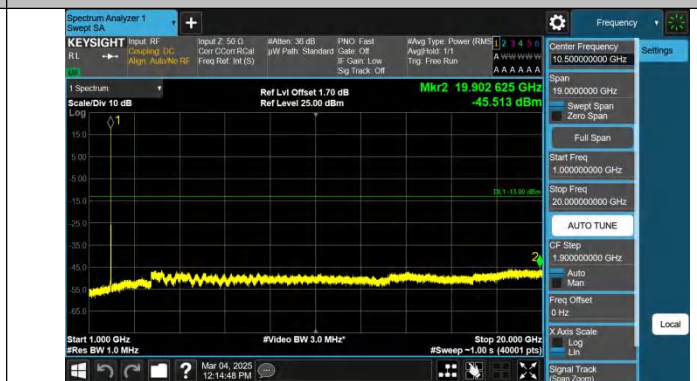
Band2-9538-5-1000~20000MHz-PASS
