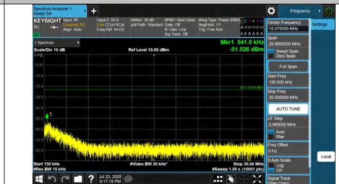
Band5-4233-0.15~30MHz-PASS
