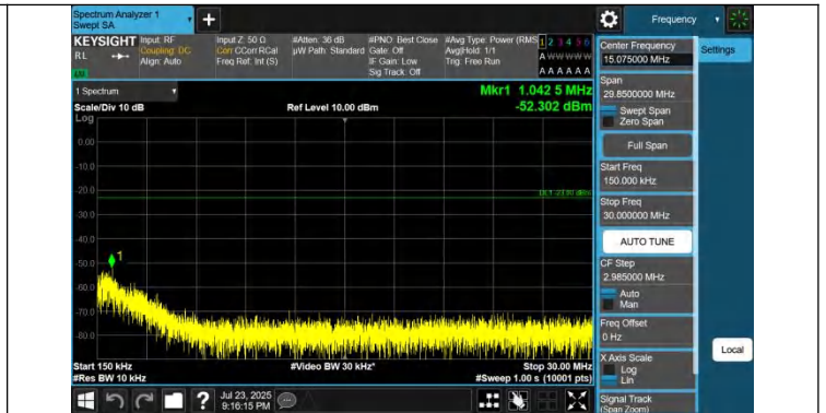
Band5-4132-0.15~30MHz-PASS
