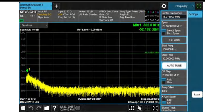
Band5-4132-3-0.15~30MHz-PASS
