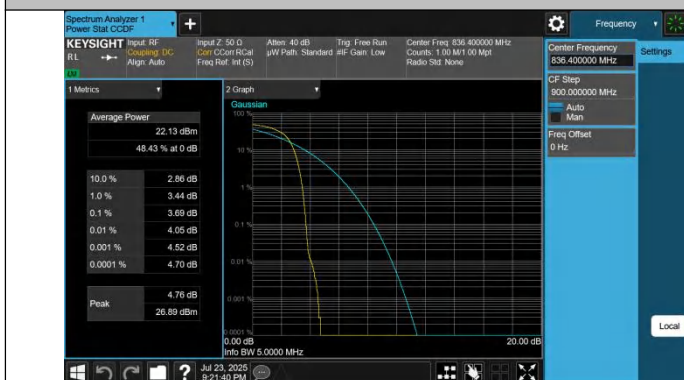
Band5-4182-3-PASS
