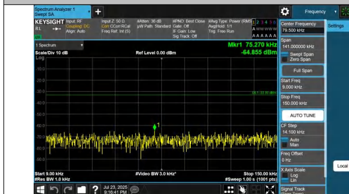
Band5-4182-0.009~0.15MHz-PASS
