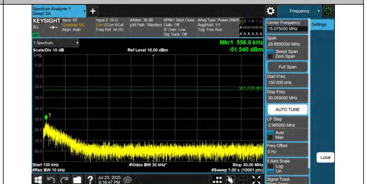
Band5-4182-0.15~30MHz-PASS
