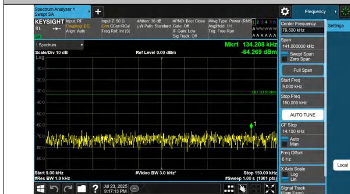
Band5-4233-0.009~0.15MHz-PASS
