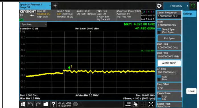
Band5-4182-1000~10000MHz-PASS
