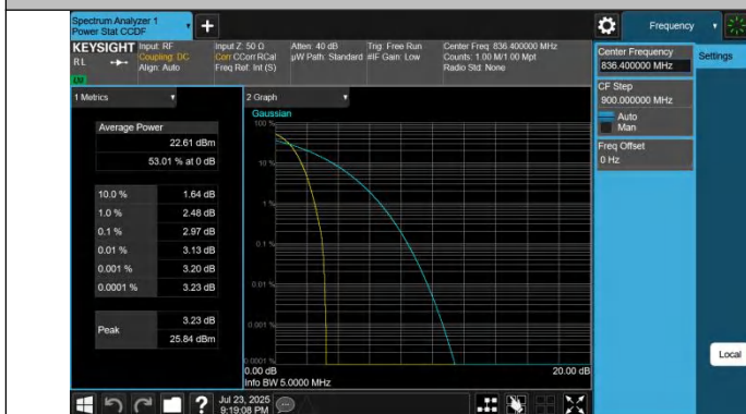
Band5-4182-1-PASS
