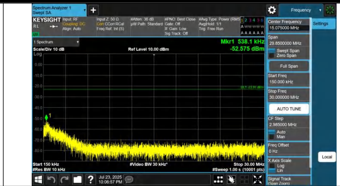
Band5-4182-1-0.15~30MHz-PASS
