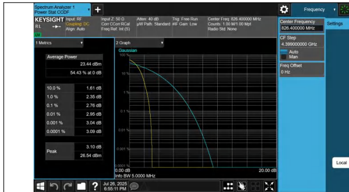
Band5-4132-PASS
