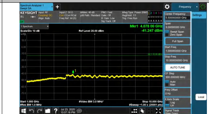
Band5-4182-1-1000~10000MHz-PASS
