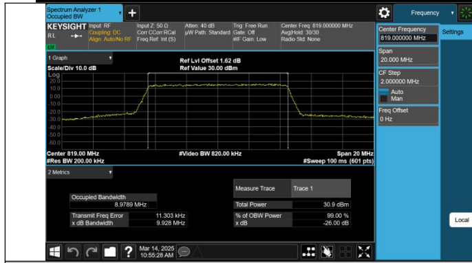
Band26(814-824)-10MHz-QPSK-26740-50RB#0-PASS
