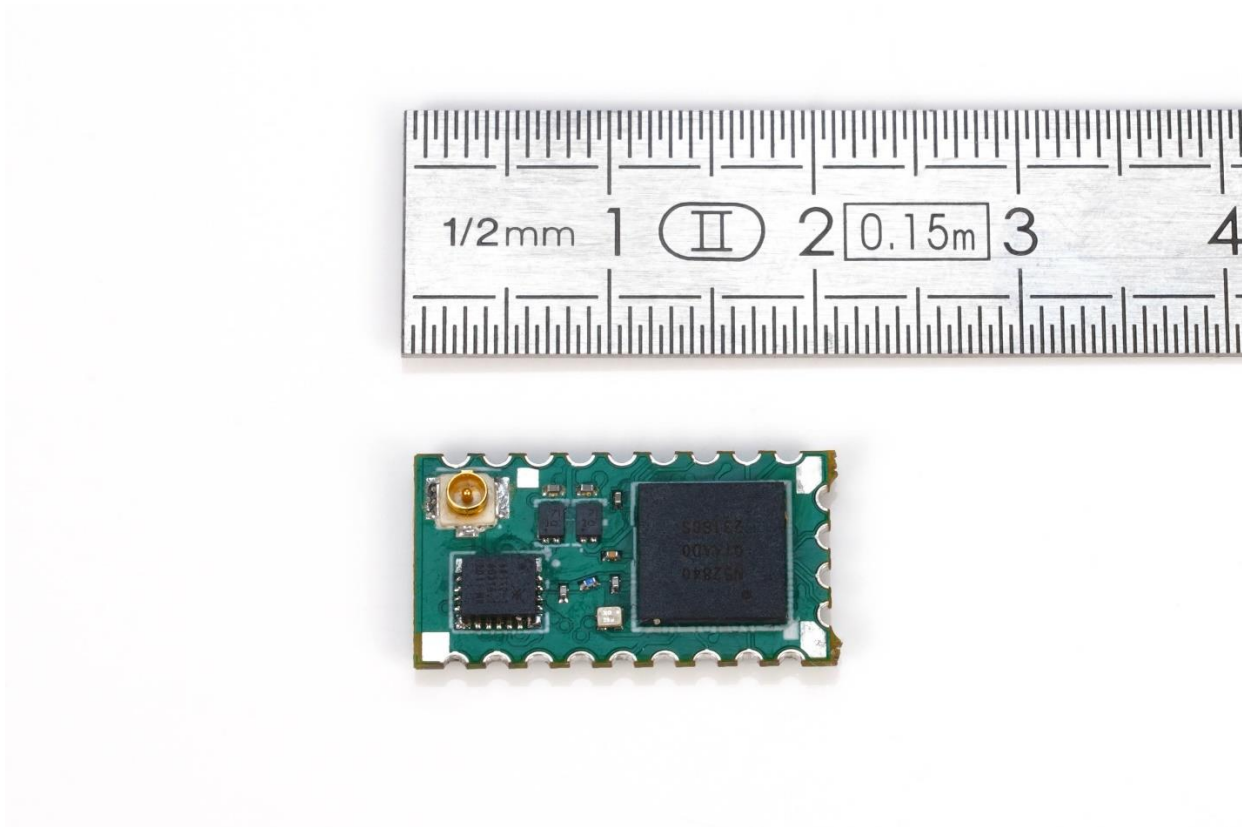
Internal Photo – Shielding removed
