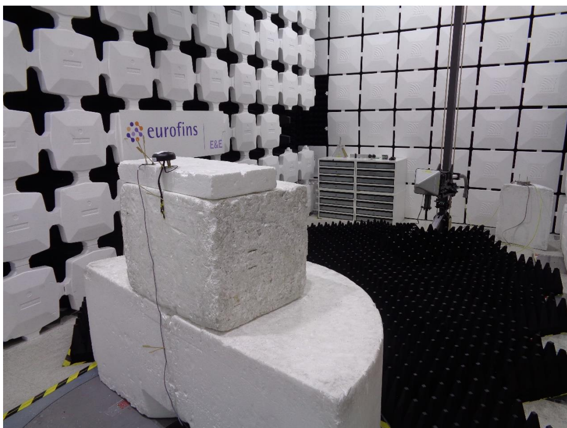
Radiated emissions 1-18GHz 3m distance – Puck antenna
