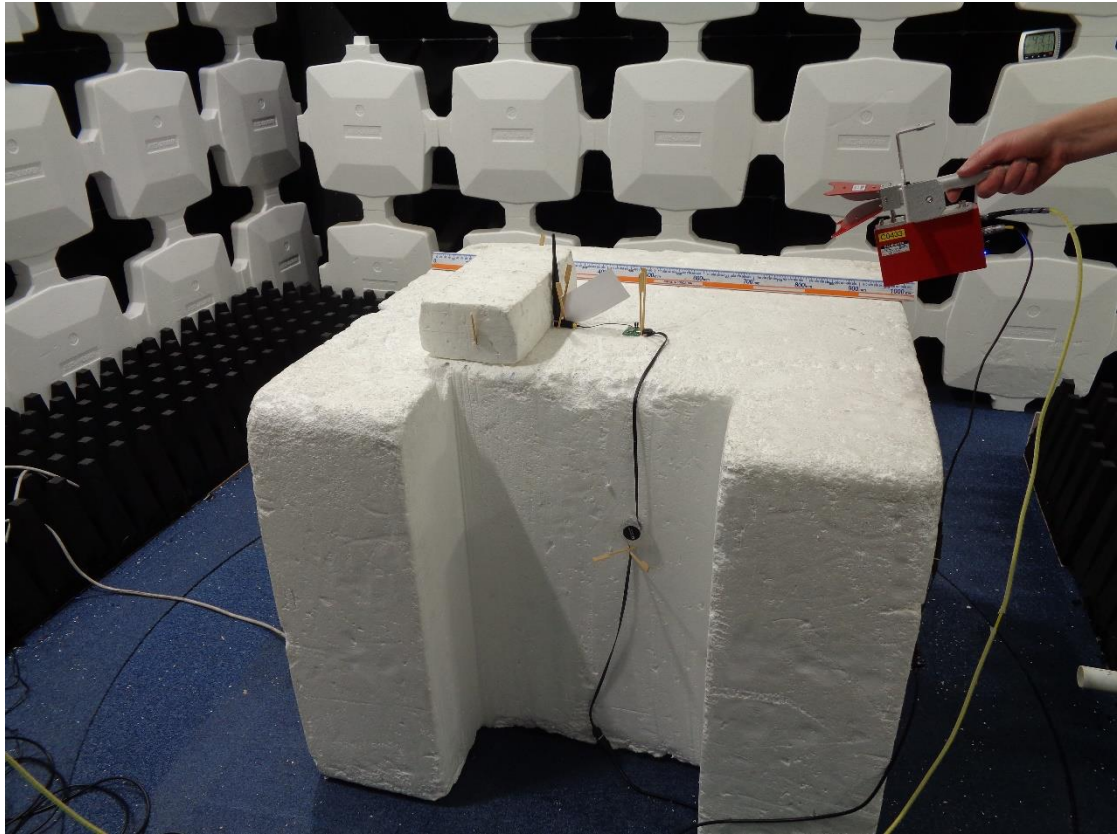
Investigative measurements 18-26GHz – Whip antenna
