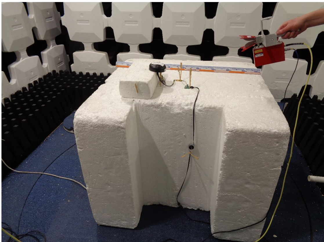
Investigative measurements 18-26GHz – Puck antenna
