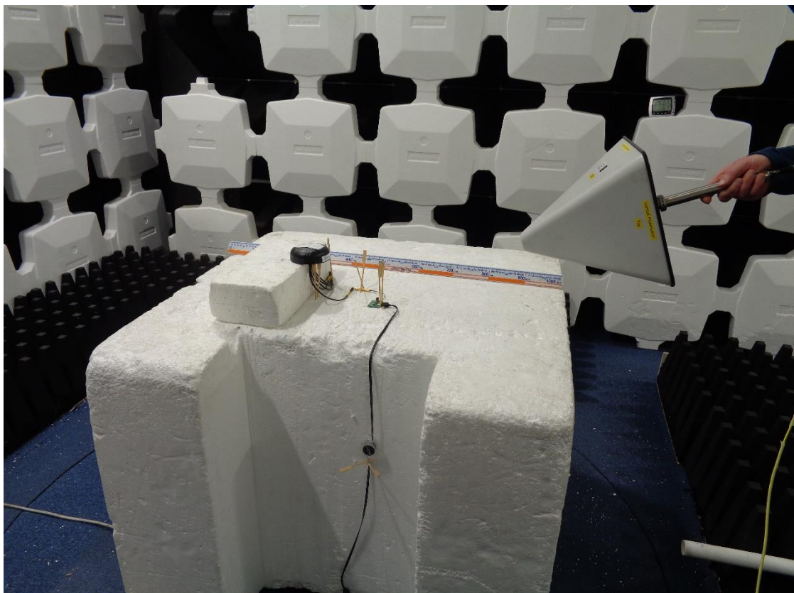
Investigative measurements 1-18GHz – Puck antenna
