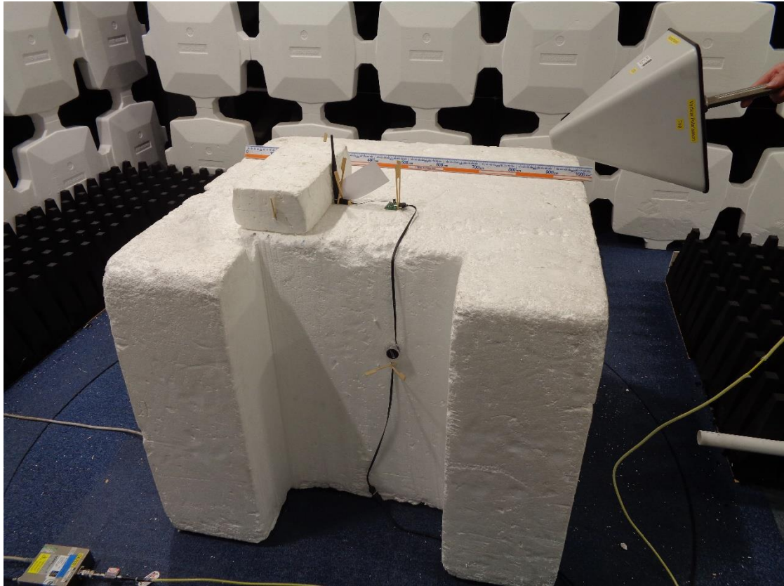
Investigative measurements 1-18GHz – Whip antenna
