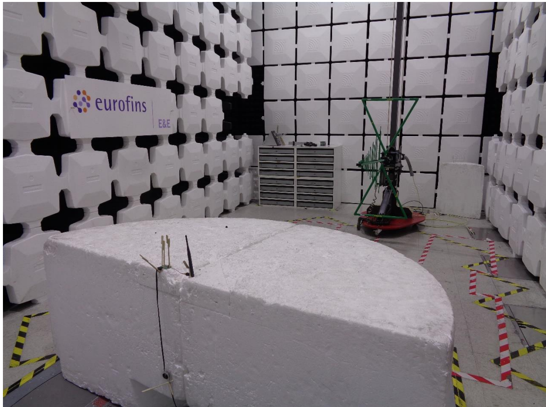
Radiated tests 30MHz to 1GHz – Whip antenna
