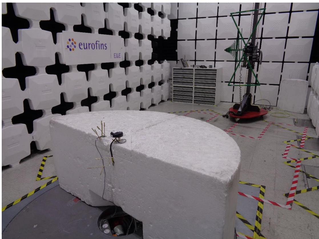
Radiated tests 30MHz to 1GHz – Puck antenna
