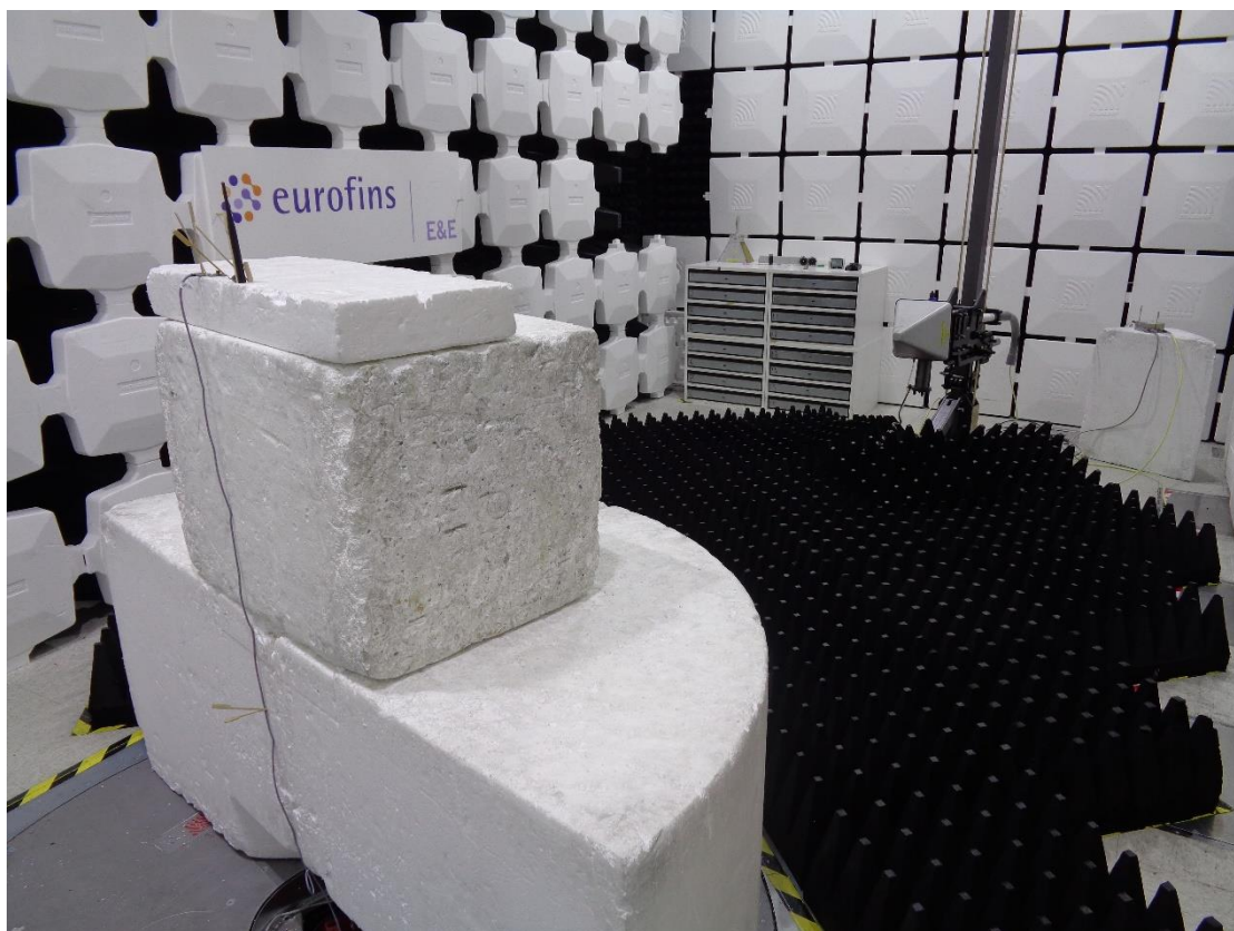
Radiated emissions 1-18GHz 3m distance – Whip antenna
