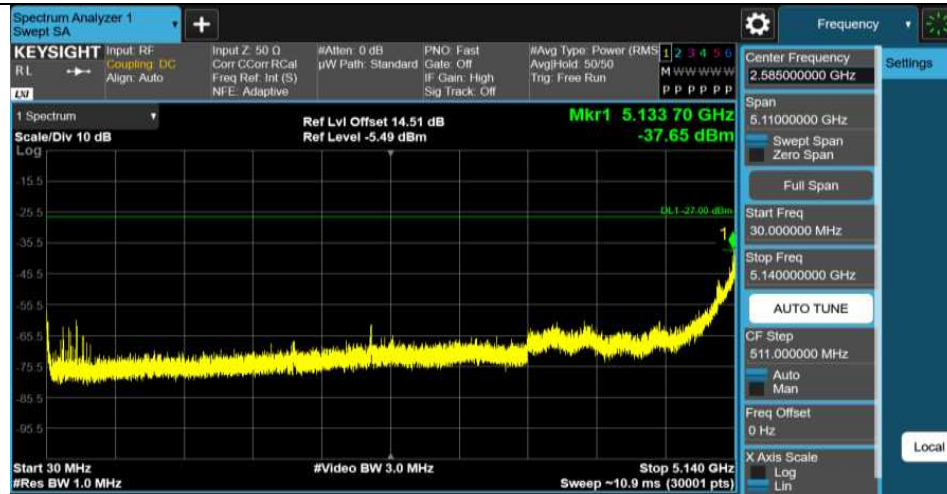
11AC40MIMO-Ant1-5190-30~5140-PASS
