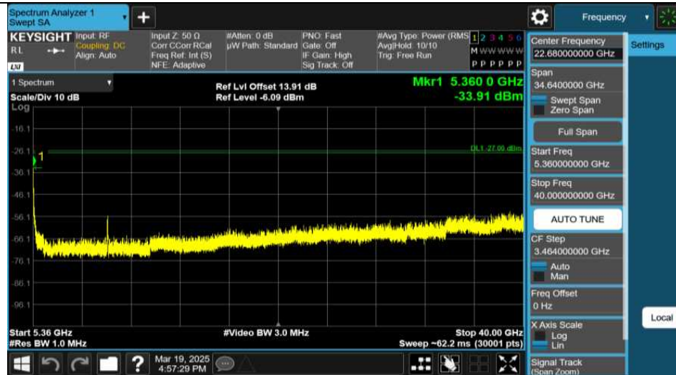
11AC40MIMO-Ant2-5310-5360~40000-PASS
