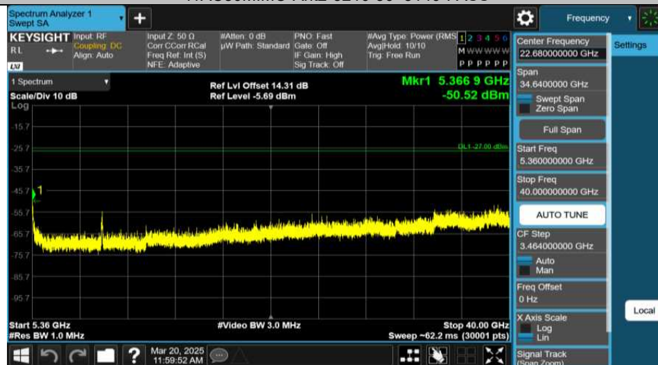
11AC80MIMO-Ant1-5210-5360~40000-PASS
