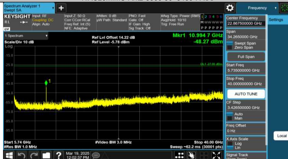
11AC20MIMO-Ant1-5500-5735~40000-PASS
