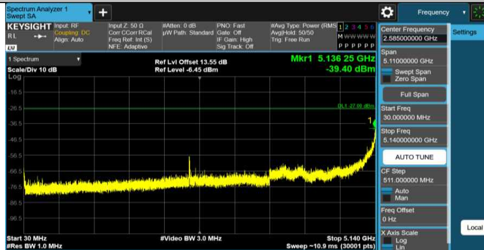
11AC40MIMO-Ant1-5190-30~5140-PASS
