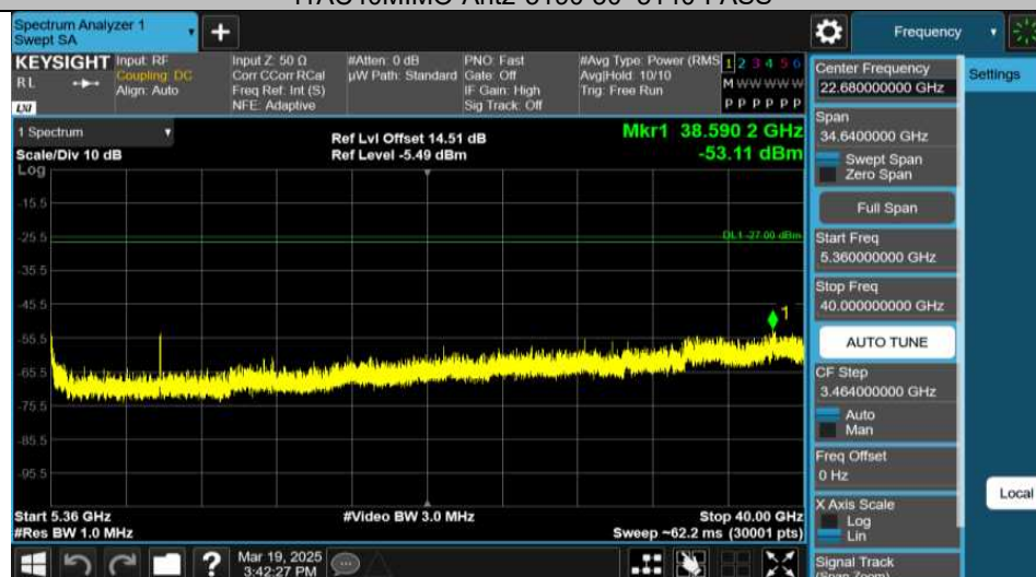
11AC40MIMO-Ant1-5190-5360~40000-PASS
