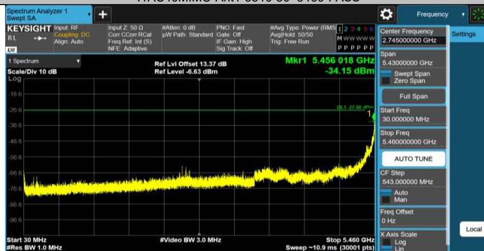
11AC40MIMO-Ant1-5510-30~5460-PASS
