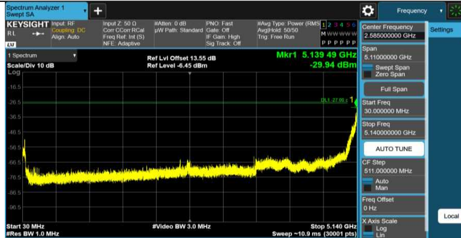
11AC80MIMO-Ant1-5210-30~5140-PASS
