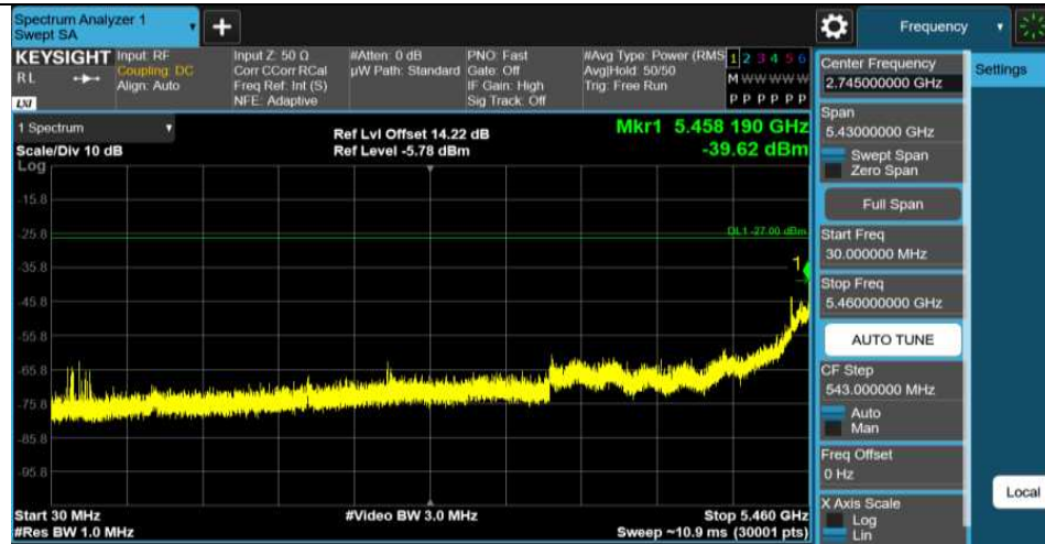
11AC20MIMO-Ant1-5500-30~5460-PASS
