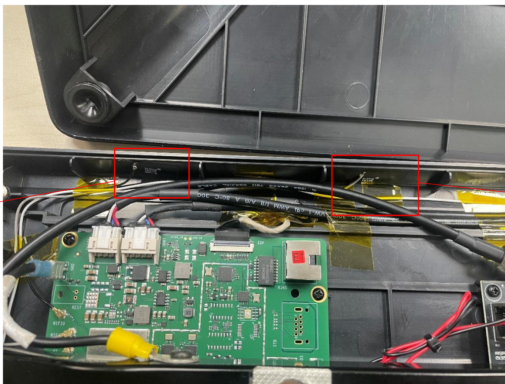
Wi-Fi 0 Antenna
