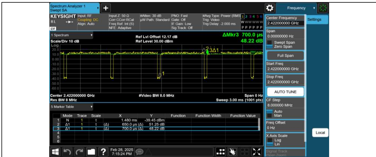
NTVN-11N40MIMO-Ant1-2422
