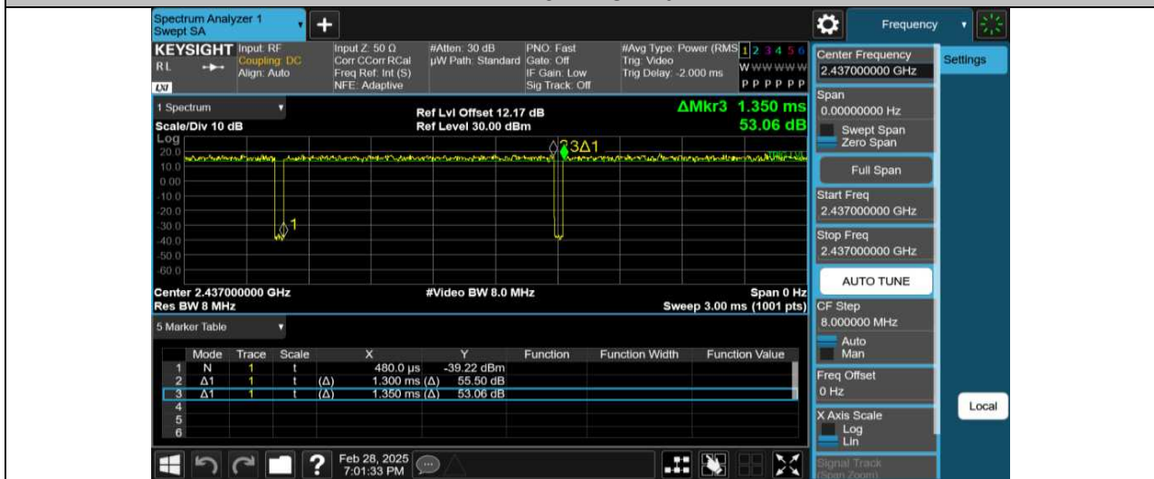
NTVN-11N20MIMO-Ant1-2437
