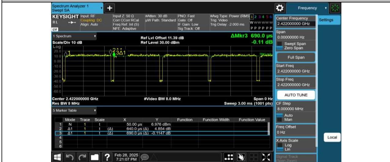
NTVN-11N40MIMO-Ant2-2422
