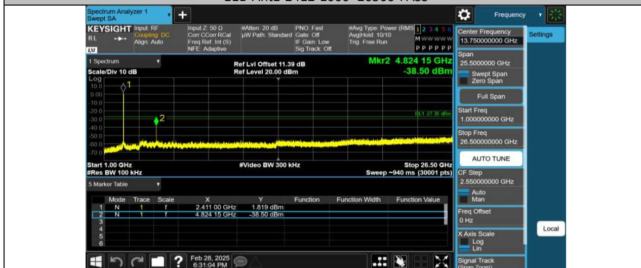
11B-Ant2-2412-1000~26500-PASS
