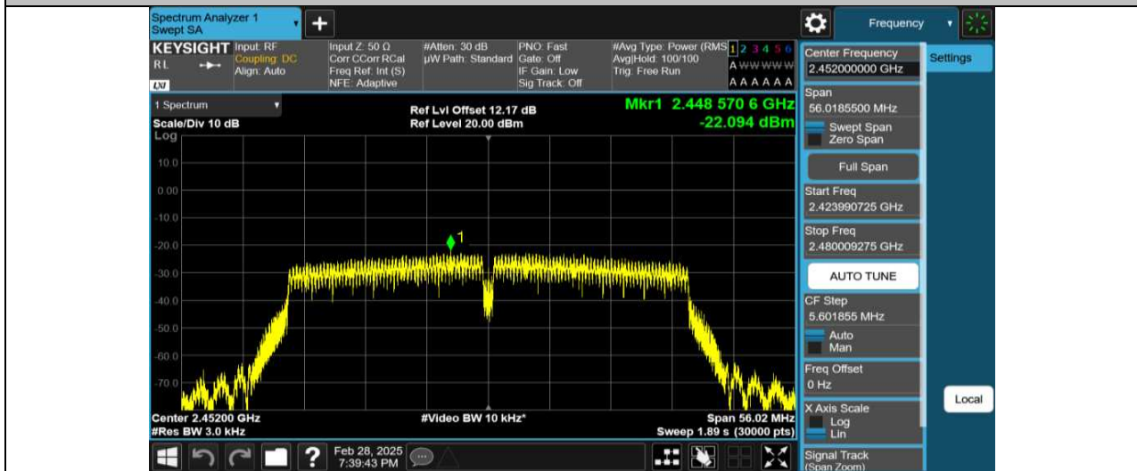
11N40MIMO-Ant1-2452-PASS
