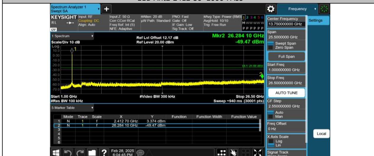
11B-Ant1-2412-1000~26500-PASS
