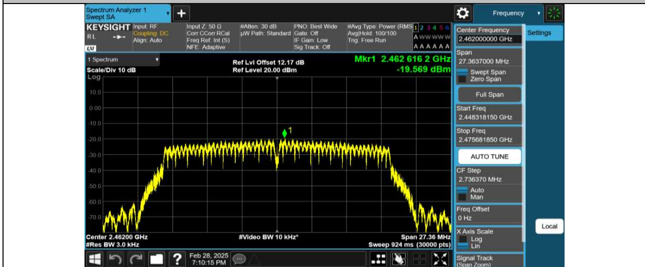
11N20MIMO-Ant1-2462-PASS
