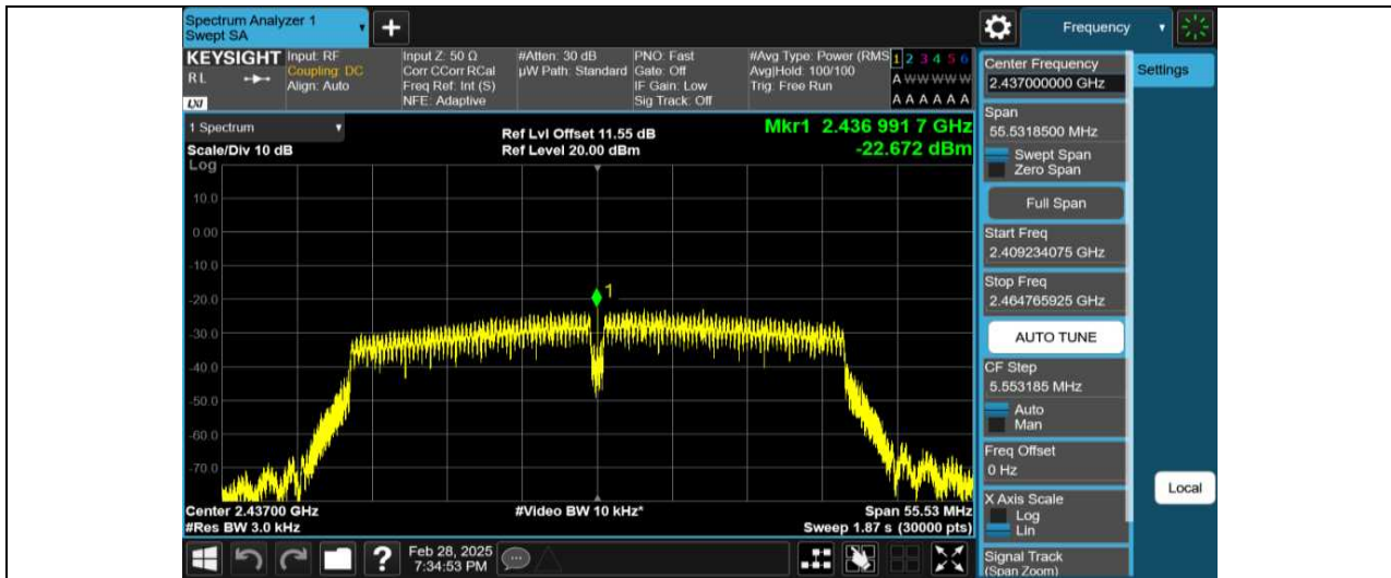
11N40MIMO-Ant2-2437-PASS
