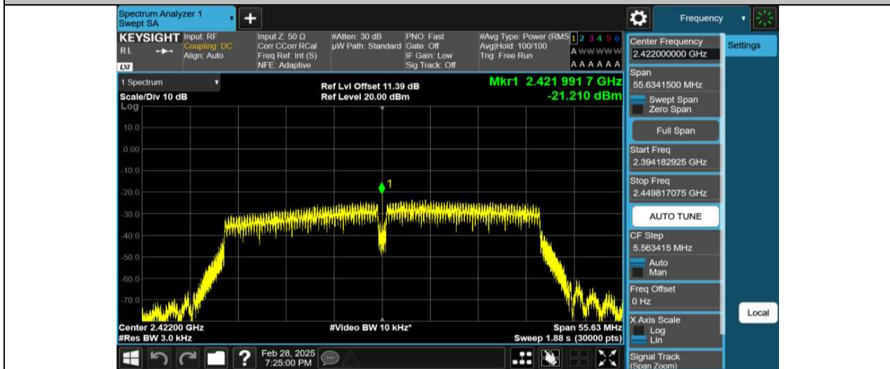
11N40MIMO-Ant2-2422-PASS
