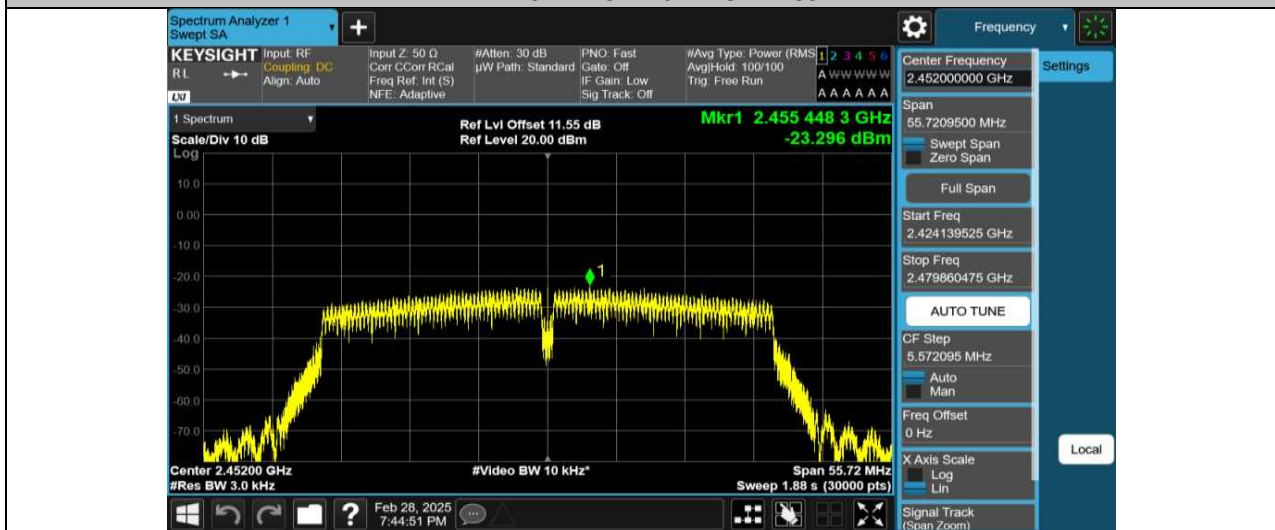
11N40MIMO-Ant2-2452-PASS
