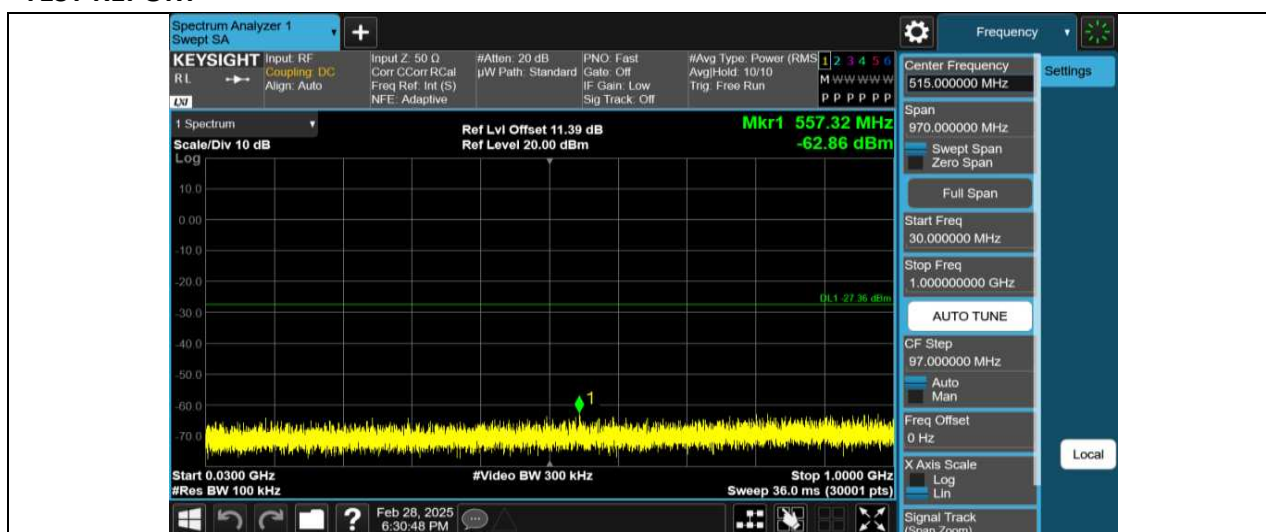
11B-Ant2-2412-30~1000-PASS
