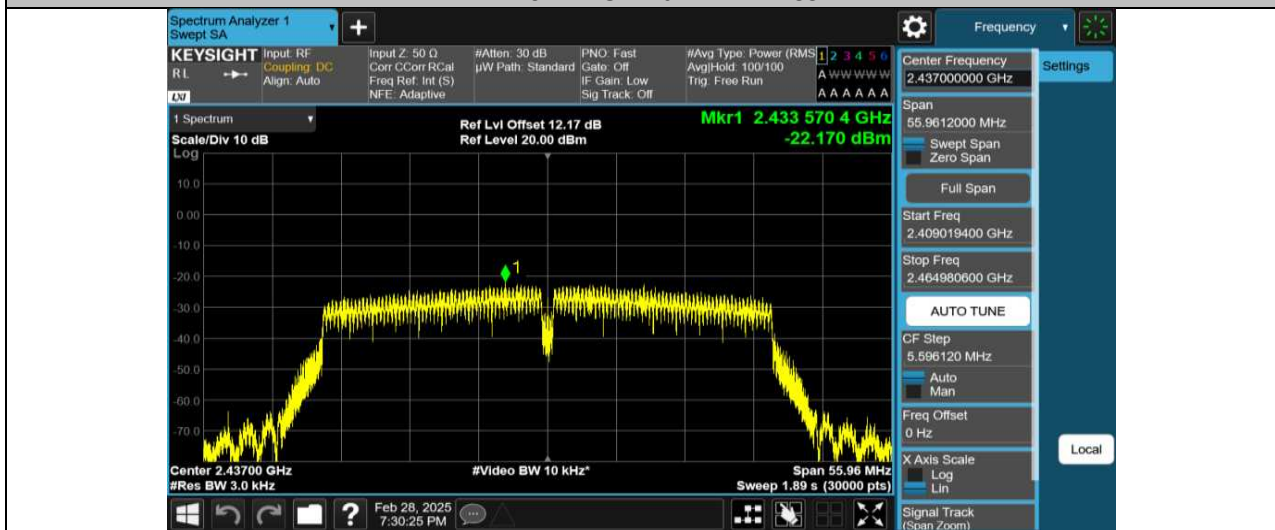
11N40MIMO-Ant1-2437-PASS
