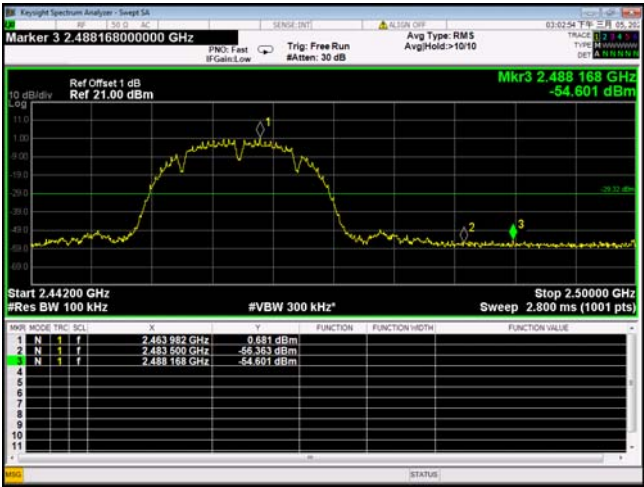
TX 11b: Band edge-right side
