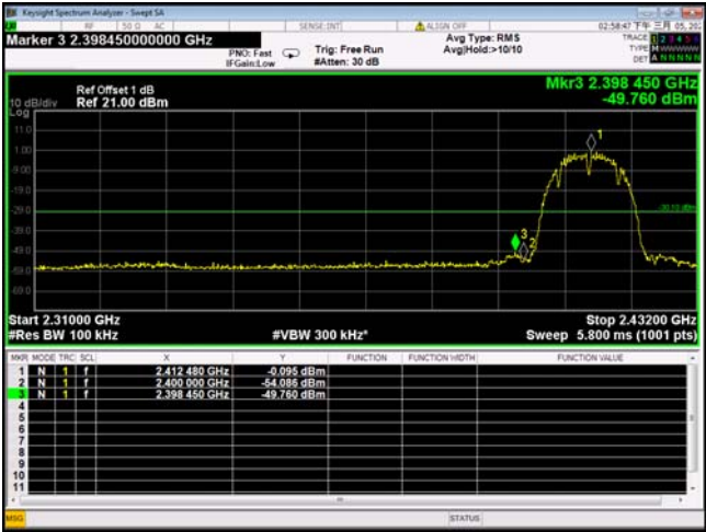
TX 11b: Band edge-left side
