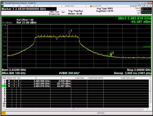
TX 11g: Band edge-right side
