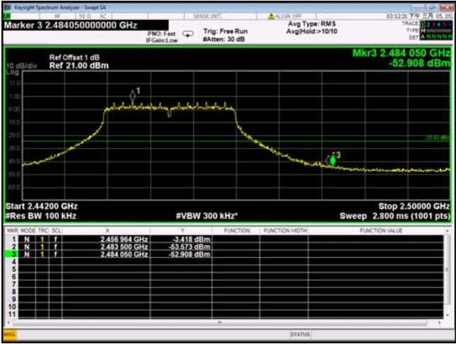
TX 11n HT20: Band edge-right side
