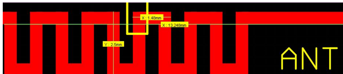
Figure 1 :keyboard Anten
