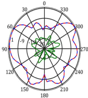
frequency=2450MHz, Y-Z Plane
