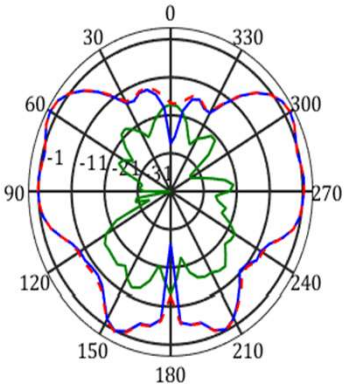
frequency=2450MHz, X-Z Plane
