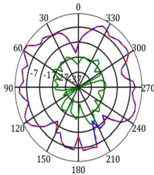
frequency=5850MHz, Y-Z Plane
