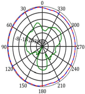
frequency=2450MHz, X-Y Plane
