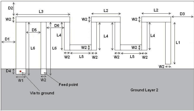
Figure 3: Antenna Dimensions
