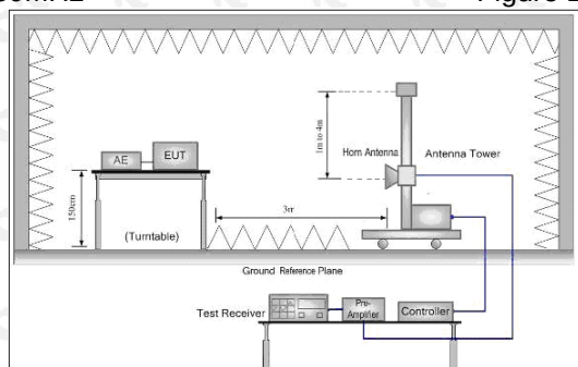
Figure 3, Above 1GHz
