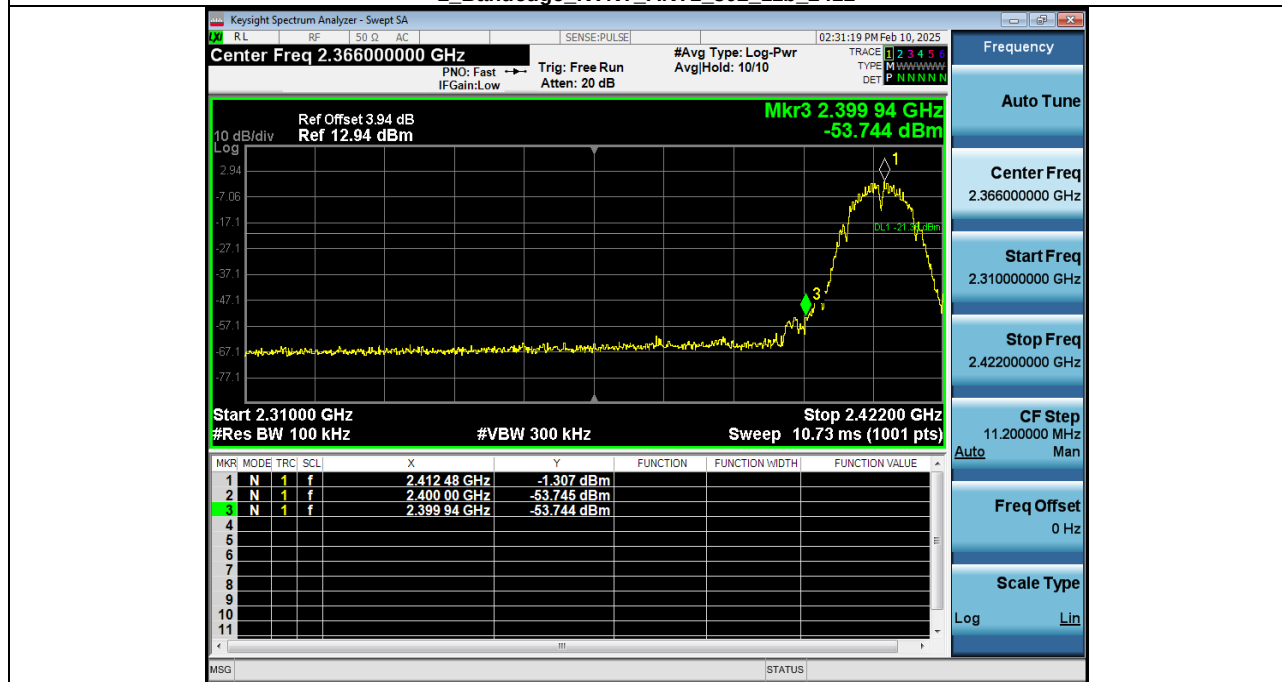
2 Bandedge_NVNT_ANT1_802_11b_2412
