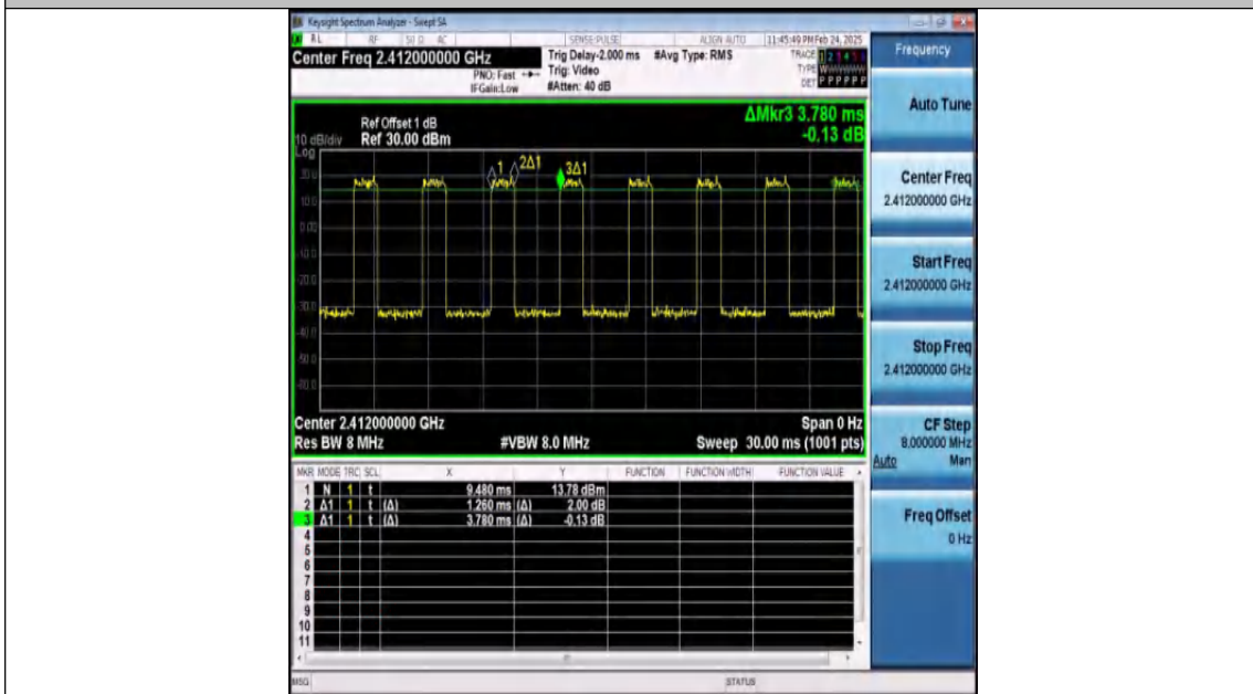
NTNV-11N20MIMO-Ant2-2412
