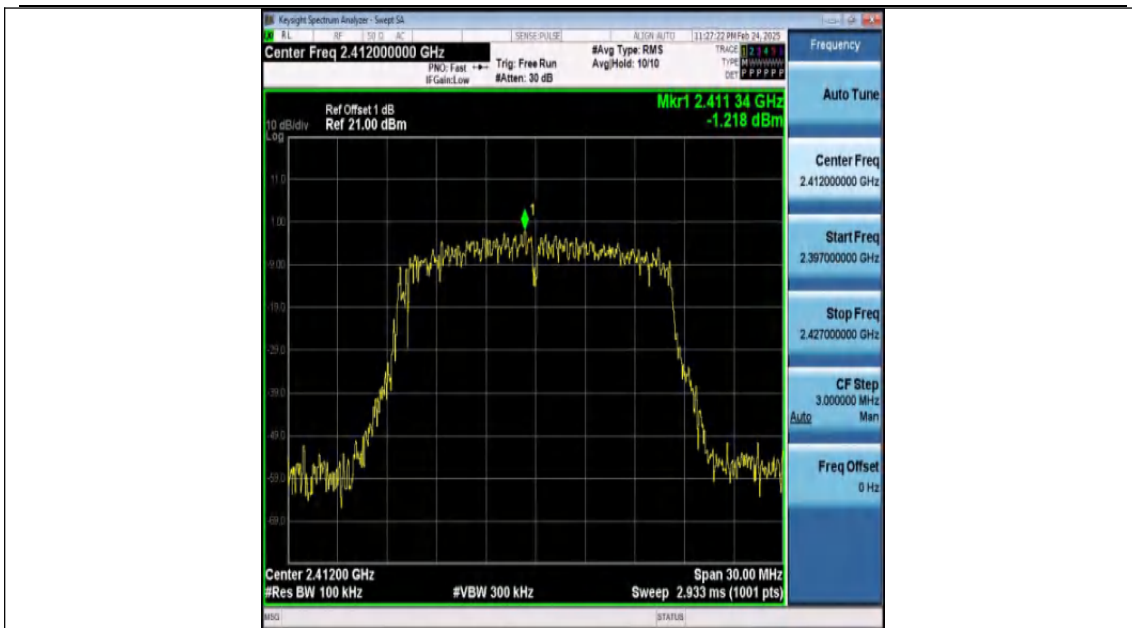
11G-Ant1-2412-0~Reference-PASS
