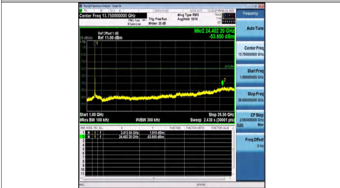
11B-Ant2-2412-1000~26500-PASS
