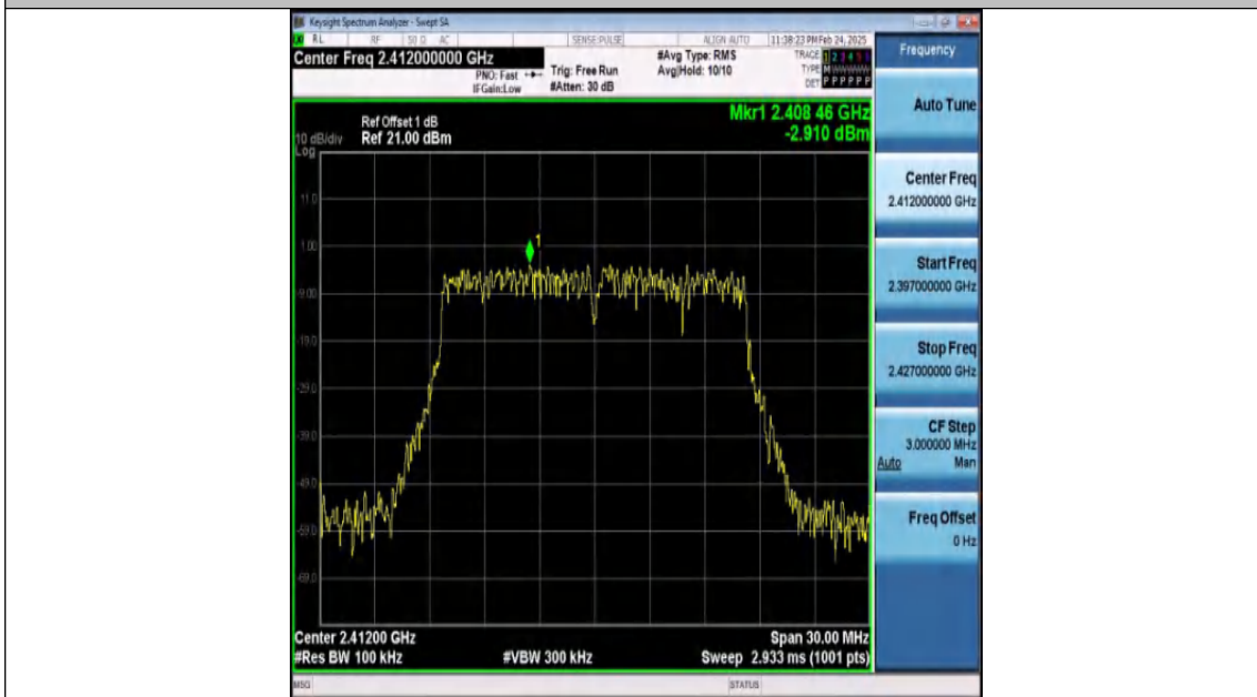
11G-Ant2-2412-0~Reference-PASS
