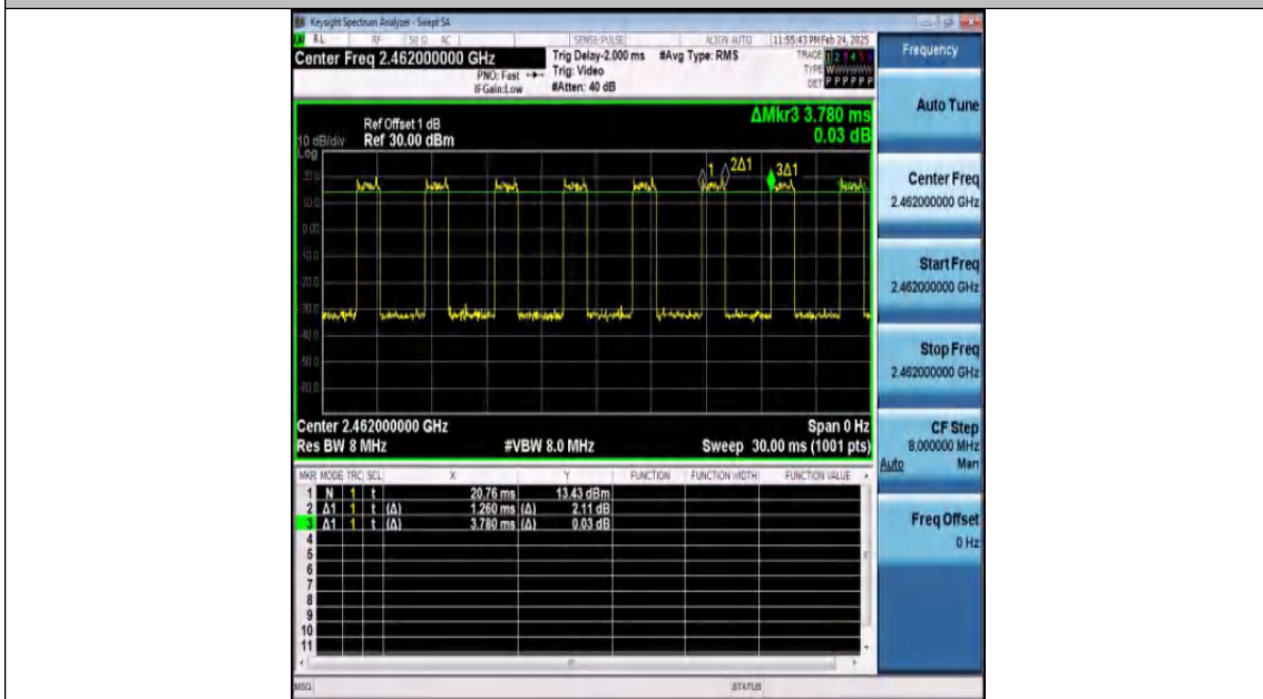
NTNV-11N20MIMO-Ant2-2462
