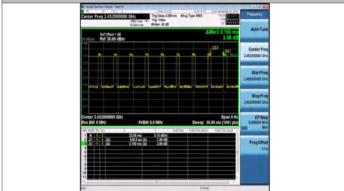
NTNV-11N40MIMO-Ant2-2452
