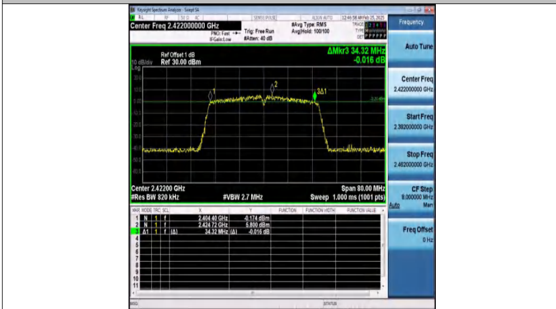
11N40MIMO-Ant2-2422-PASS
