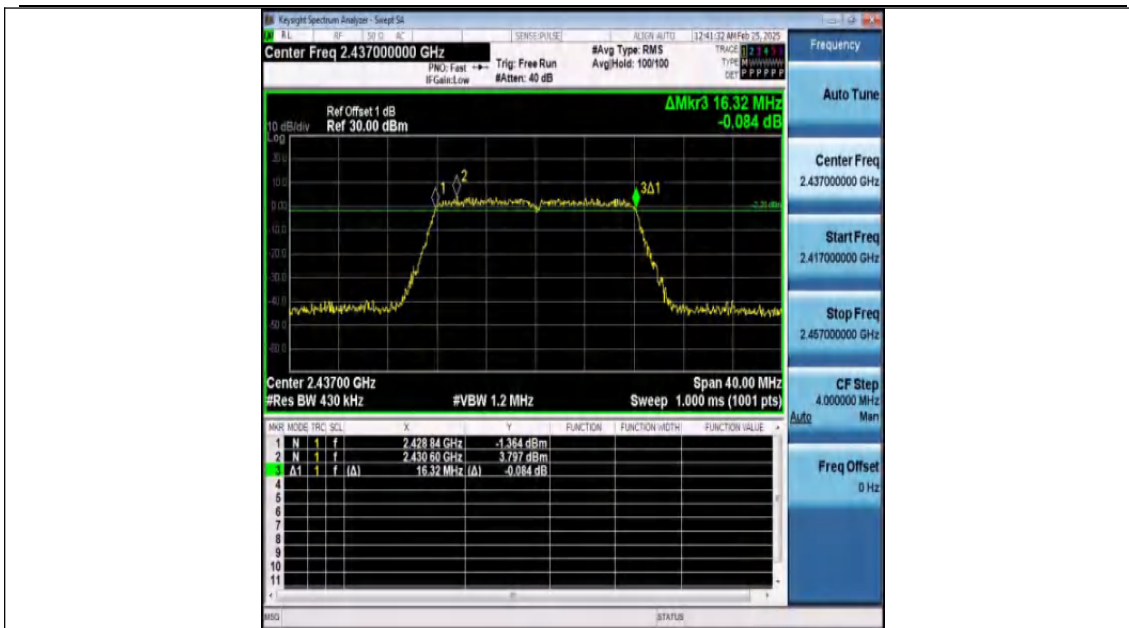
11G-Ant1-2437-PASS
