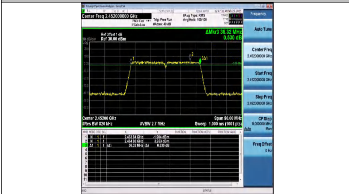
11N40MIMO-Ant2-2452-PASS
