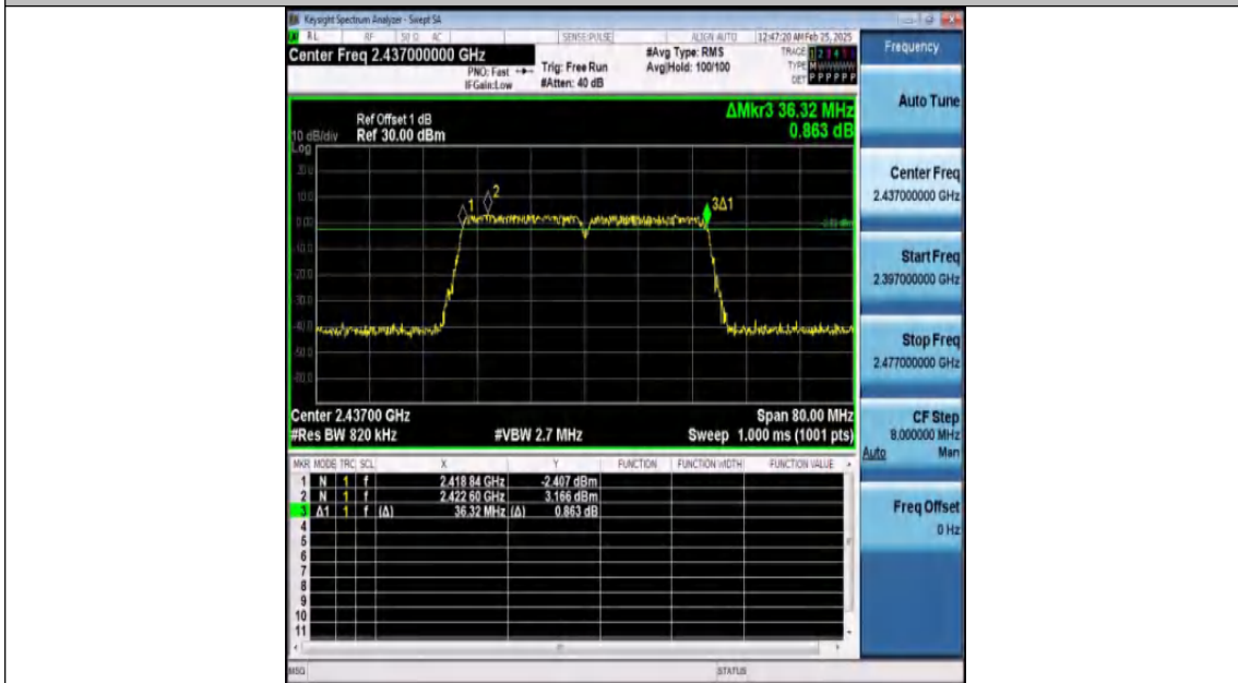
11N40MIMO-Ant2-2437-PASS
