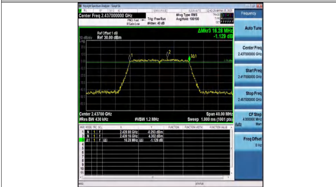
11G-Ant2-2437-PASS
