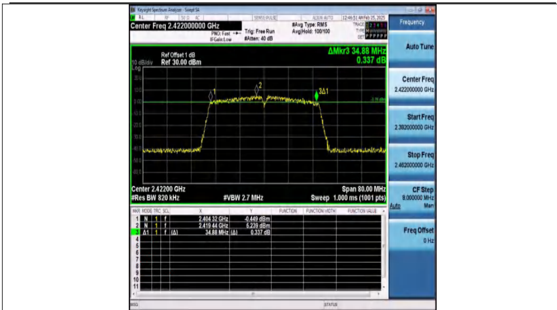
11N40MIMO-Ant1-2422-PASS
