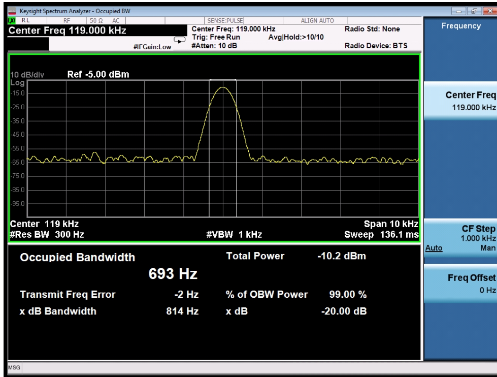
20dB Bandwidth
