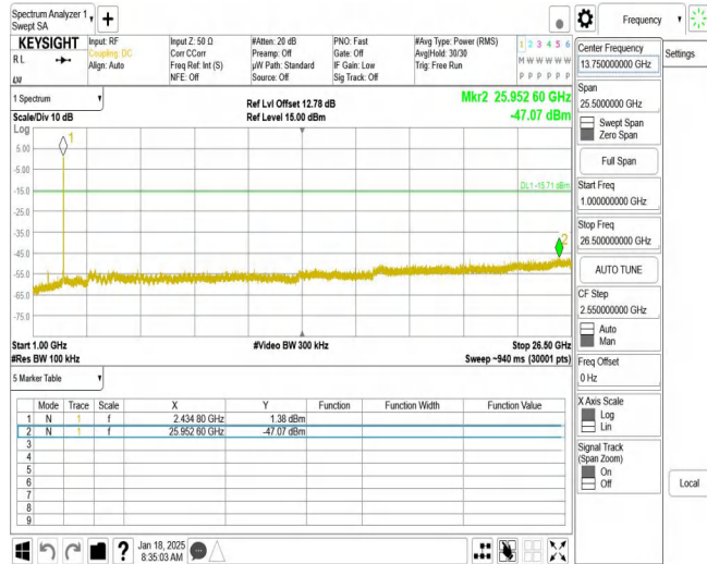
11G_Ant2_2437_1000~26500
