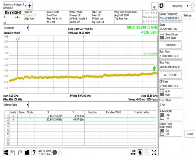
11G_Ant1_2437_1000~26500
