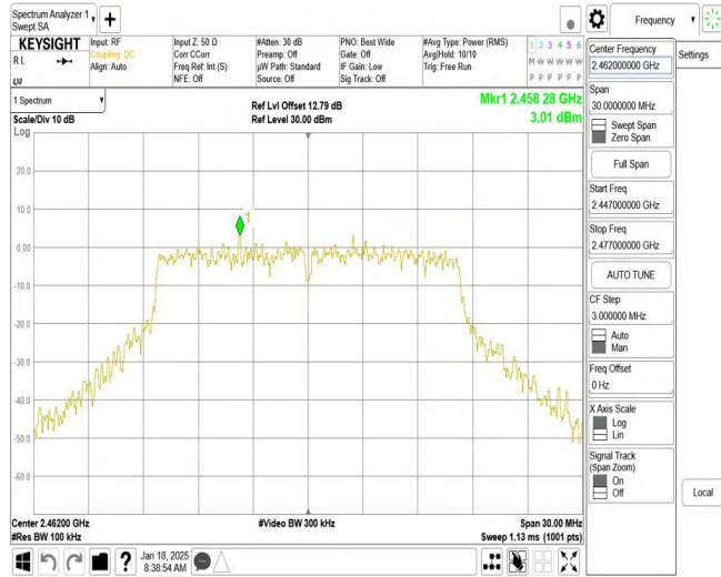
11G_Ant2_2462_0~Reference
