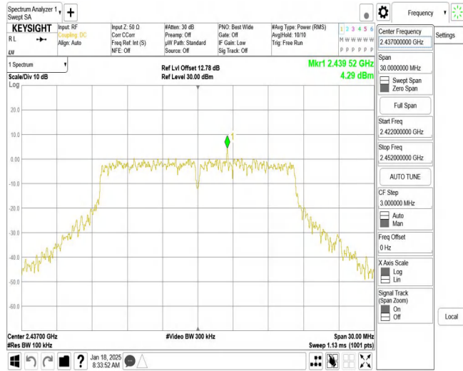
11G_Ant2_2437_0~Reference
