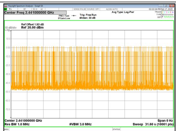
3DH5-2441MHz-Accumulated
