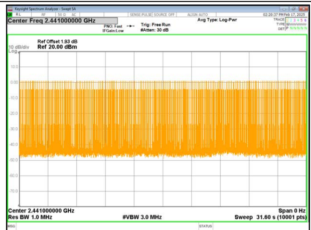
2DH3-2441MHz-Accumulated
