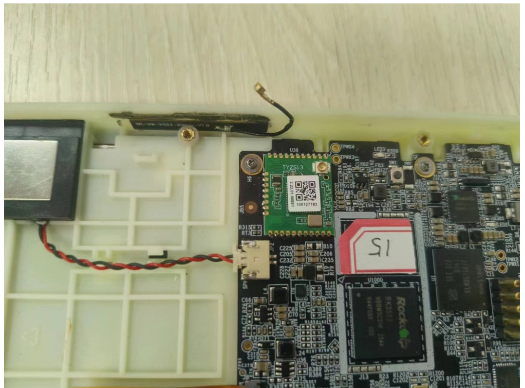
Antenna Zigbee
