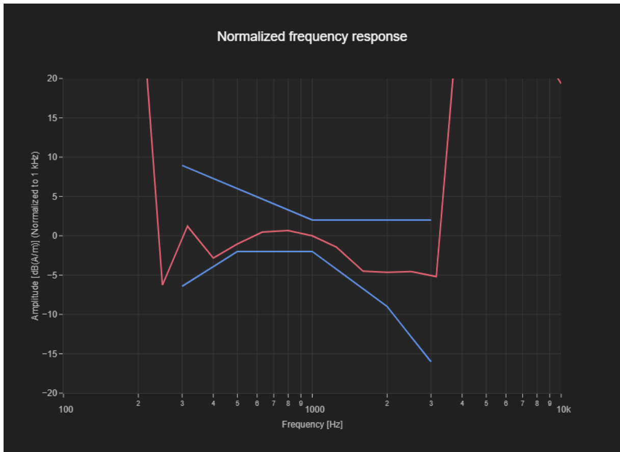
Figure C.4 Frequency Response of LTE B48 ANT4-OTT
