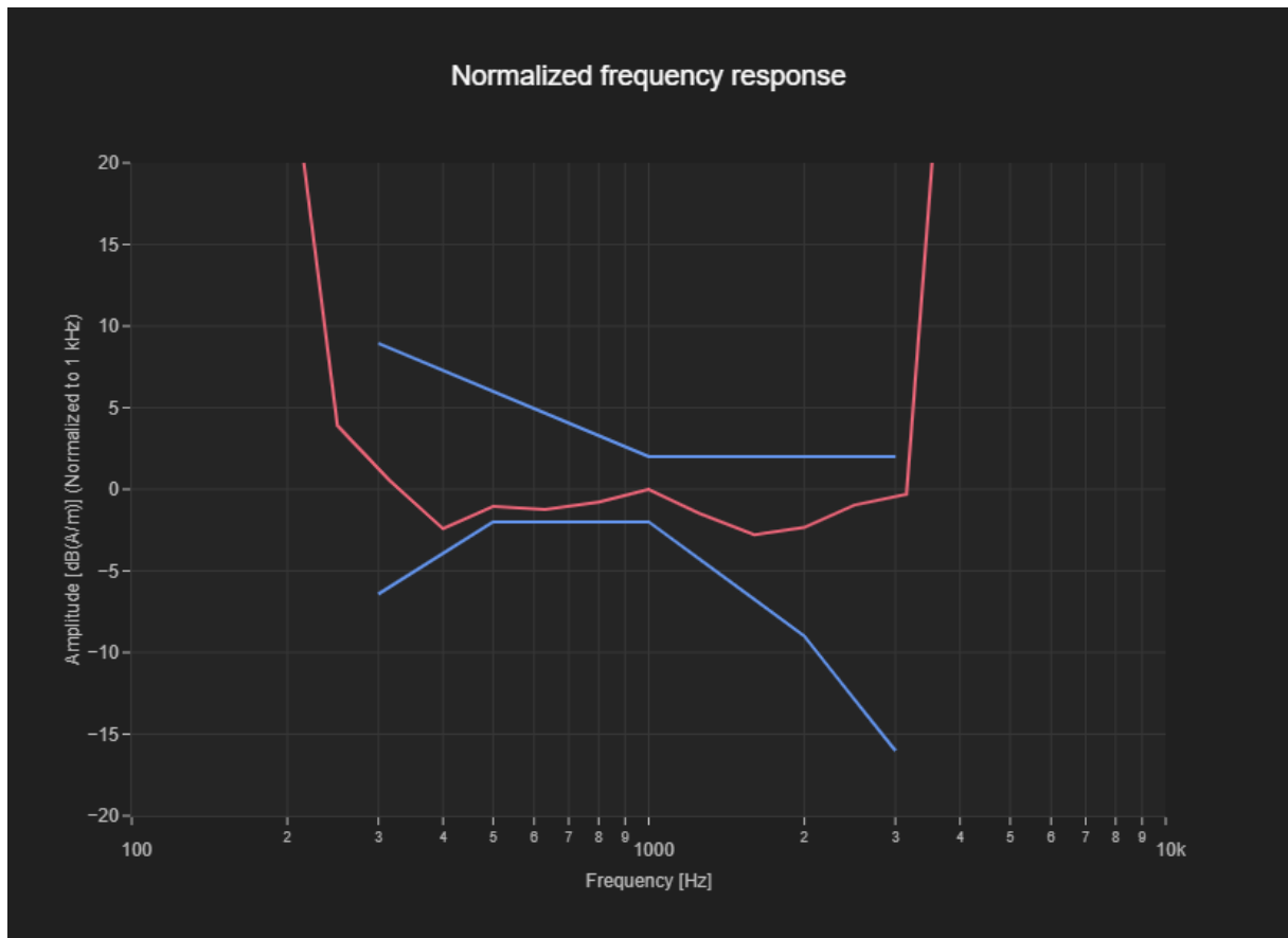
Figure C.3 Frequency Response of GSM850 ANT2-OTT
