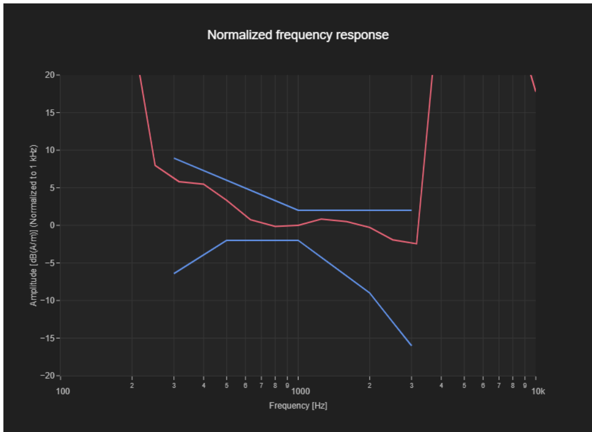
Figure C.2 Frequency Response of NR B66-N41
