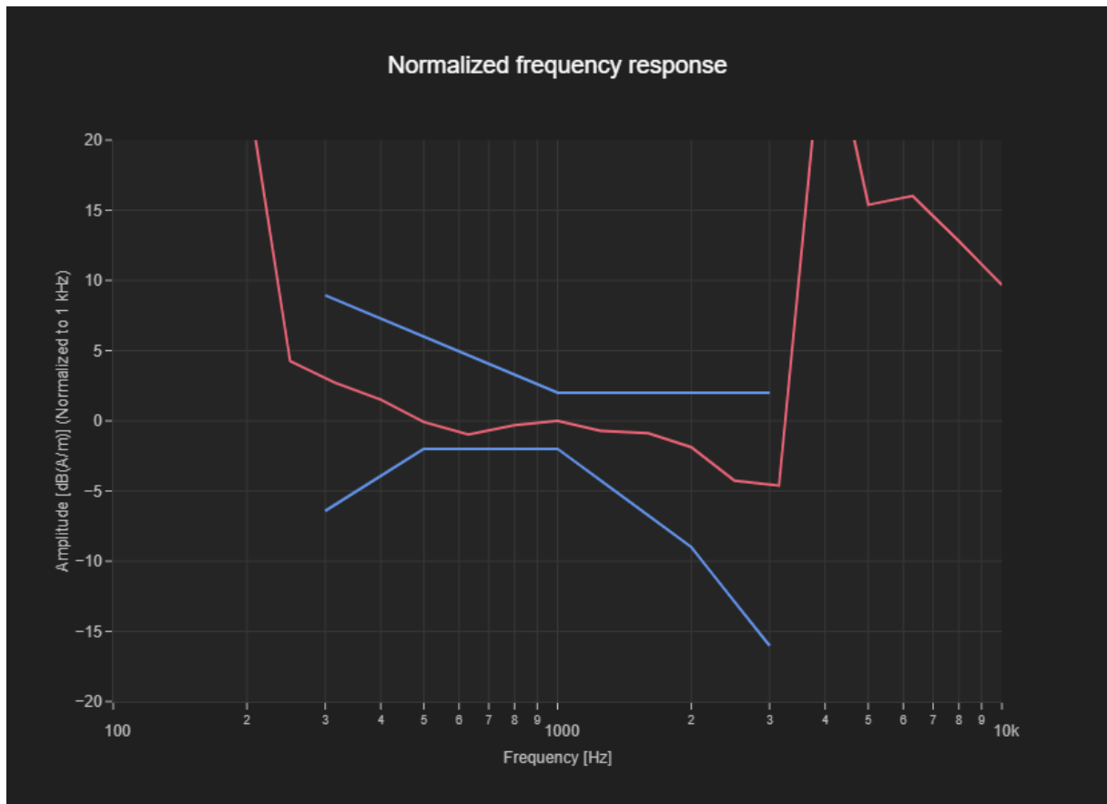
Figure C.1 Frequency Response of GSM1900 ANT1
