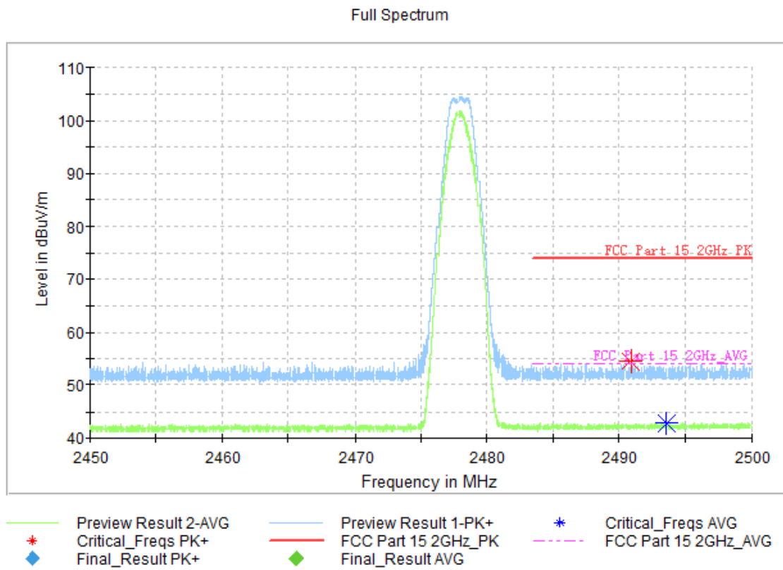
Fig.19. Frequency Band Edges: BLE 2M, 2478 MHz, Hopping Off , 2.45 GHz - 2.50GHz
