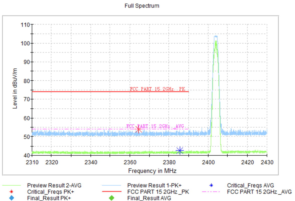
Fig.18. Frequency Band Edges: BLE 2M, 2404 MHz, Hopping Off, 2.31 GHz – 2.43GHz
