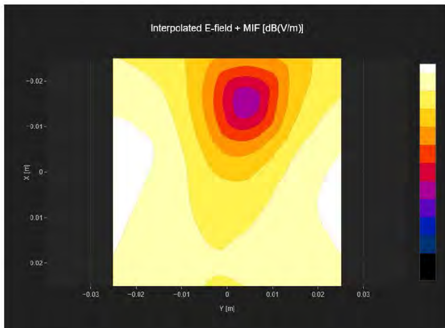
Fig B.2 GSM 1900 ANT3
