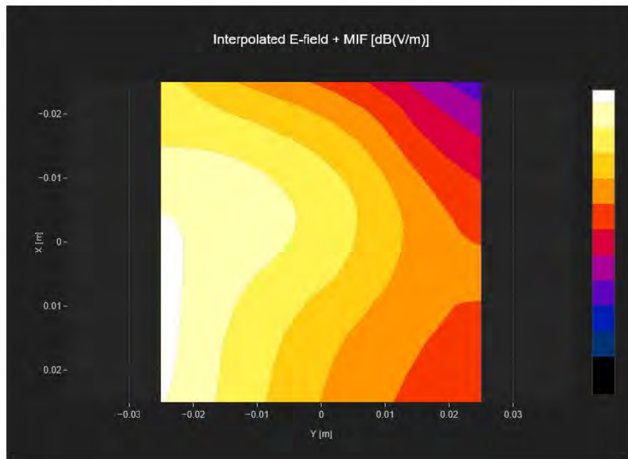
Fig B.3 LTE Band41 PC2 ANT3
