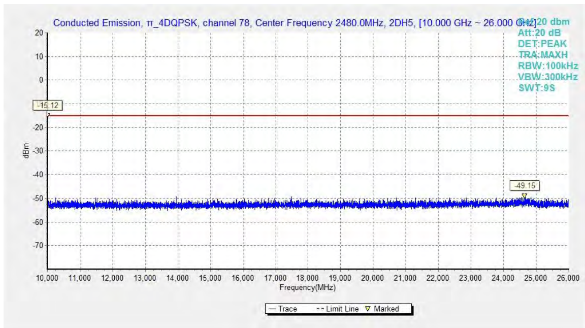
Fig.42. Conducted spurious emission: \pi_4 /4 DQPSK, Channel 78, 10GHz - 26GHz
