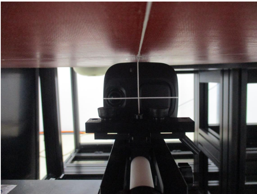
Right Side from Flat Phantom (Separation Distance: 0.5 cm)_Ant.1
