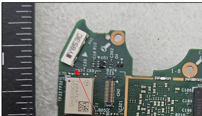
Chip Antenna
