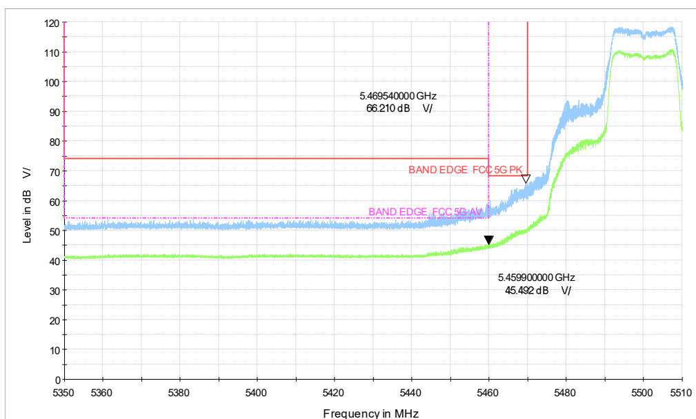
5G WIFI_a CH100_5.35-5.51GHz_6M
