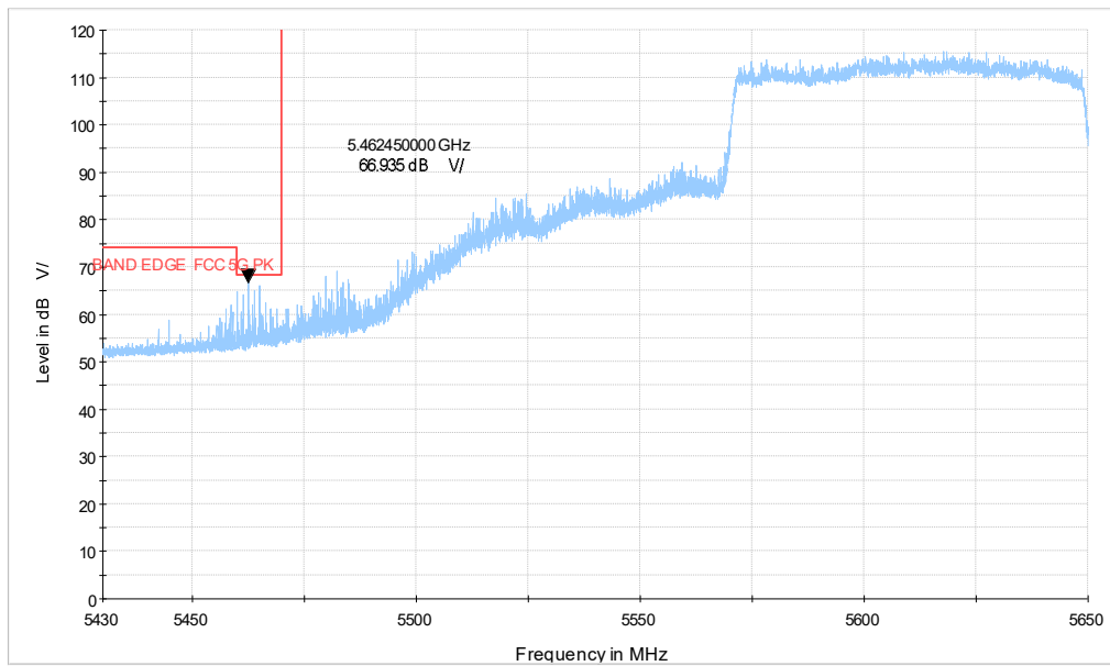
5G WIFI_ax80 CH122_5.43-5.65GHz_MCS0
