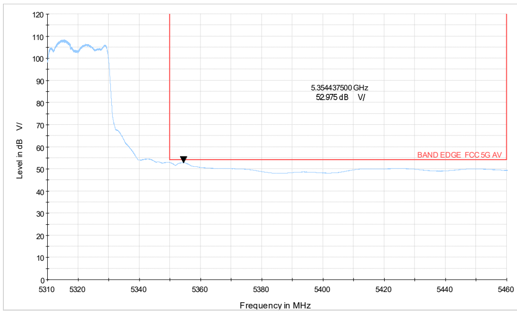
5G WIFI_ax20 CH64_5.31-5.46GHz_AV
