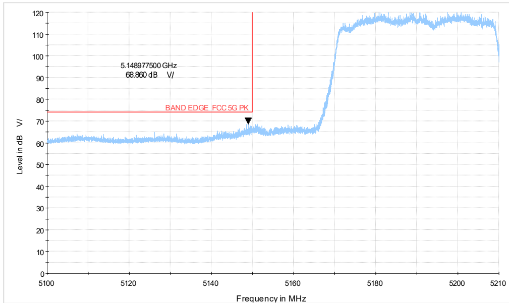
5G WIFI_ax40 CH38_5.1-5.21GHz_PK
