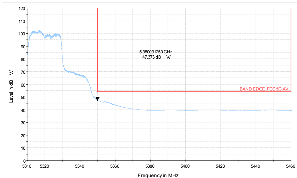
5G WIFI_n20 CH64_5.31-5.46GHz_MCS0_AV
