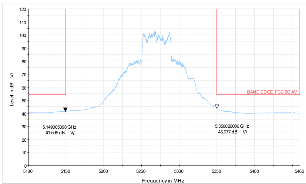
5G WIFI_n40 CH54_5.1-5.46GHz_MCS0_AV
