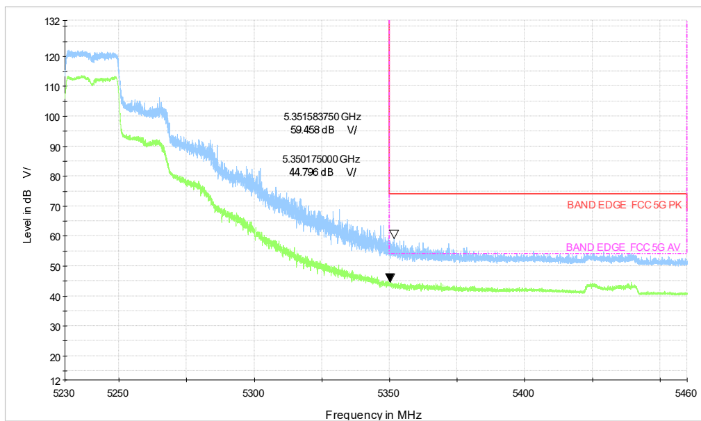
5G WIFI_ax20 CH48_5.23-5.46GHz_MCS0
