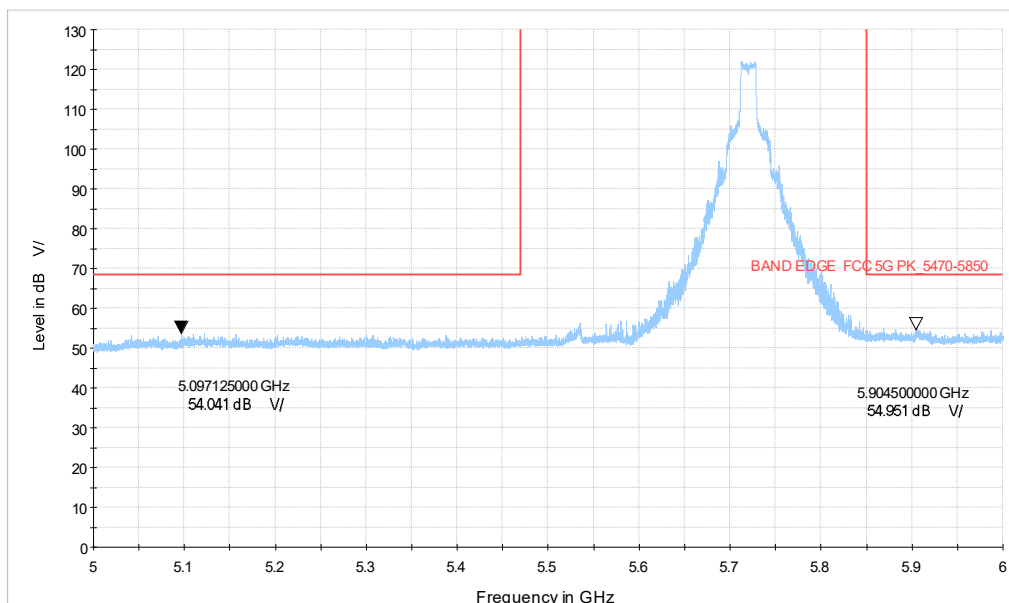
5G WIFI_a CH144_5-6GHz_6M
