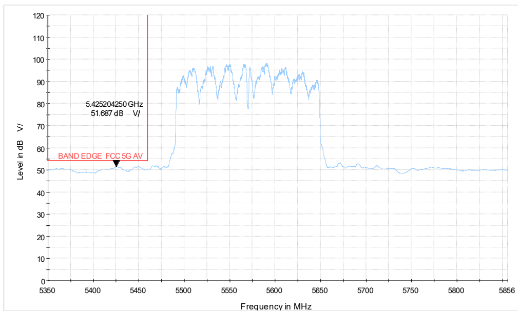
5G WIFI_ac160 CH114_5.35-5.856GHz_AV
