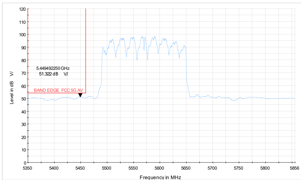
5G WIFI_ax160 CH114_5.35-5.856GHz_AV
