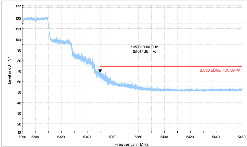
5G WIFI_ax20 CH60_5.29-5.46GHz_MCS0_PK
