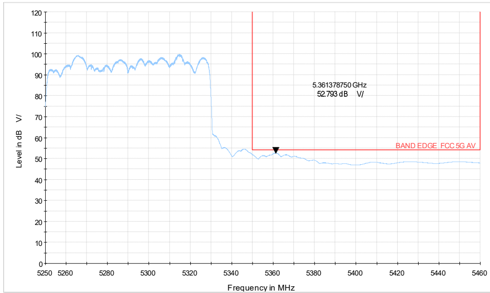
ax80-996TONE_CH58_5.25-5.46GHz_AV
