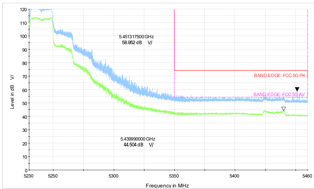
5G WIFI_n20 CH48_5.23-5.46GHz_MCS0
