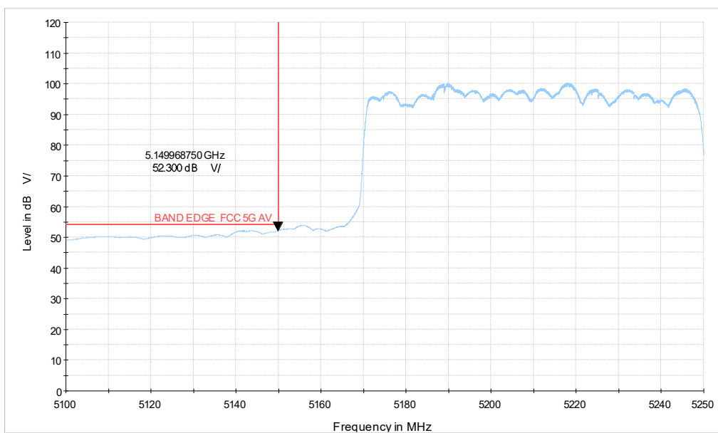
5G WIFI_ax80 CH42_5.1-5.25GHz_AV
