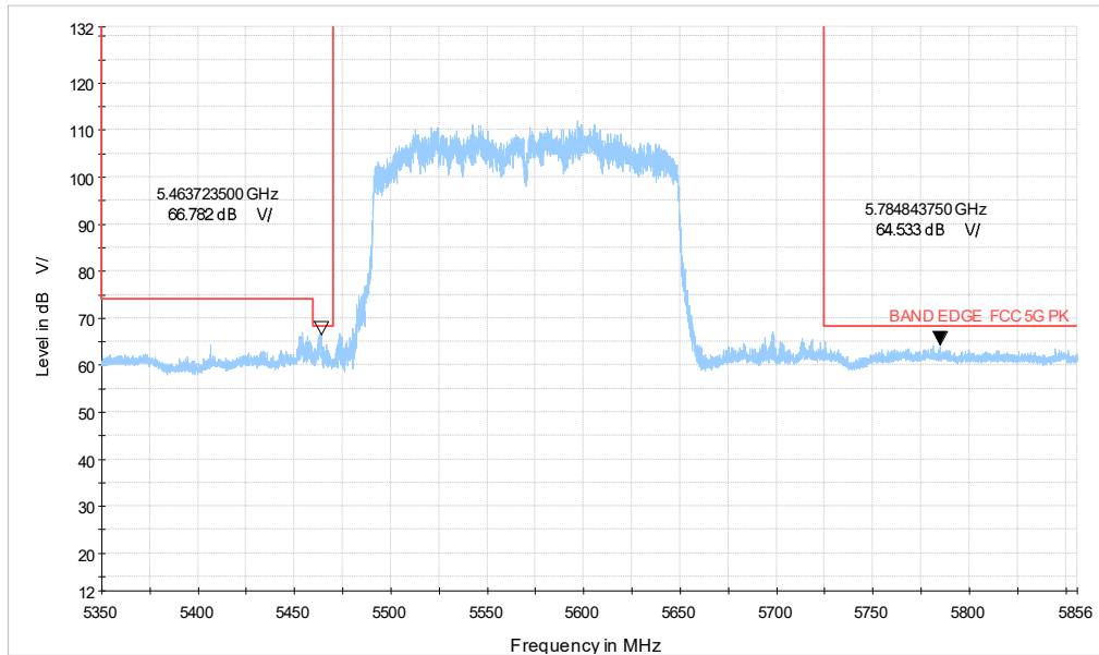
ax160-996x2TONE_CH114_5.35-5.856GHz_PK
