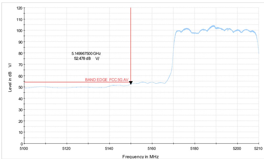
5G WIFI_ax40 CH38_5.1-5.21GHz_AV
