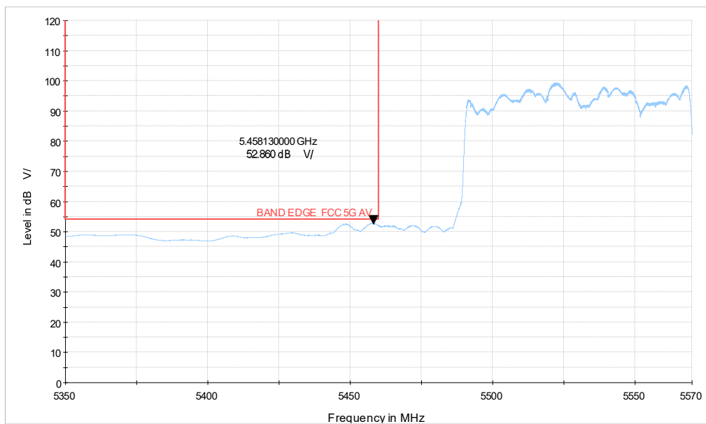
ax80-996TONE_CH106_5.35-5.57GHz_AV
