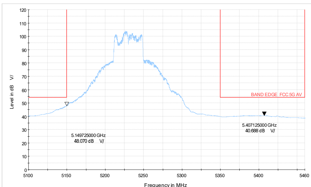
5G WIFI_n40 CH46_5.1-5.46GHz_MCS0_AV
