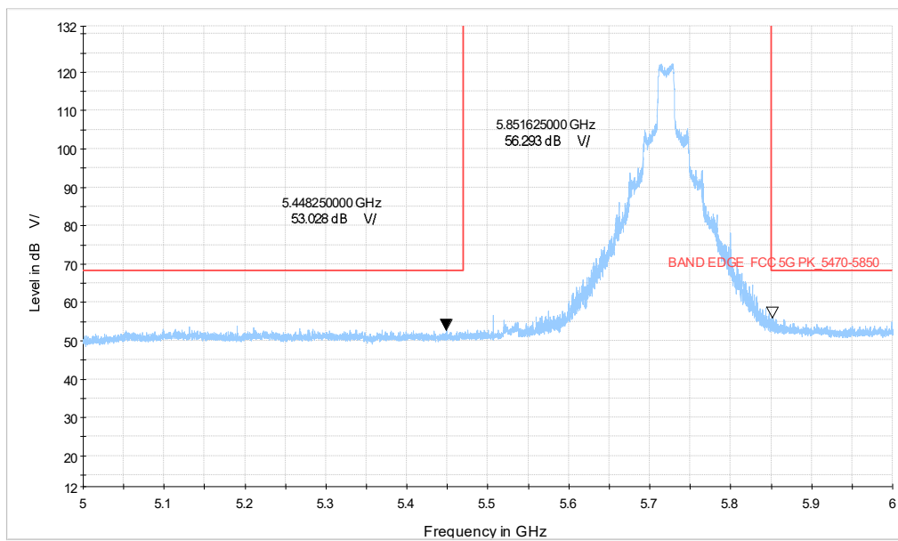
5G WIFI_ax20 CH144_5-6GHz_MCS0
