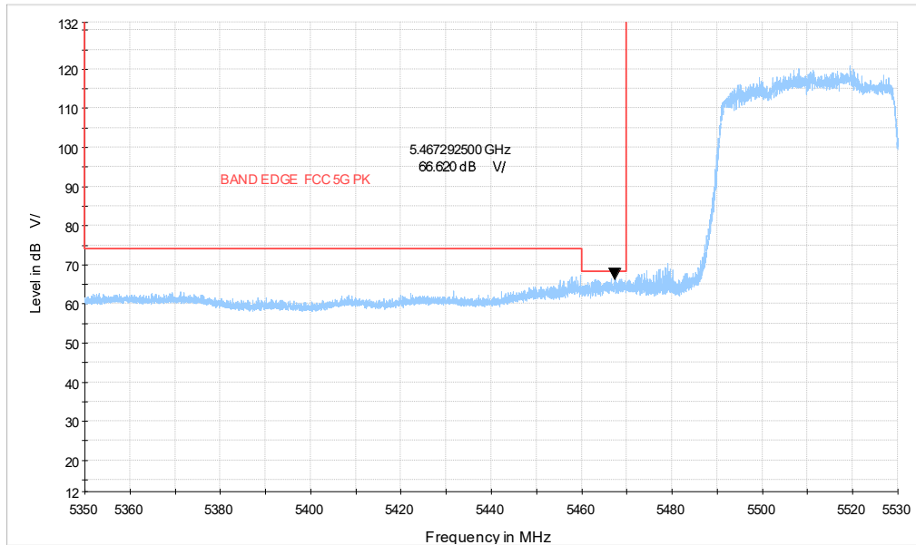
ax40-484TONE_CH102_5.35-5.53GHz_PK
