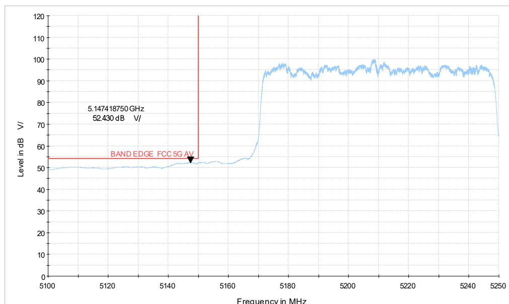
5G WIFI_ac80 CH42_5.1-5.25GHz_AV
