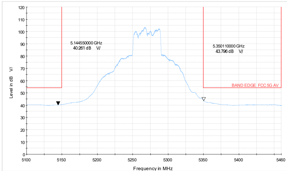
5G WIFI_ax40 CH54_5.1-5.46GHz_MCS0_AV
