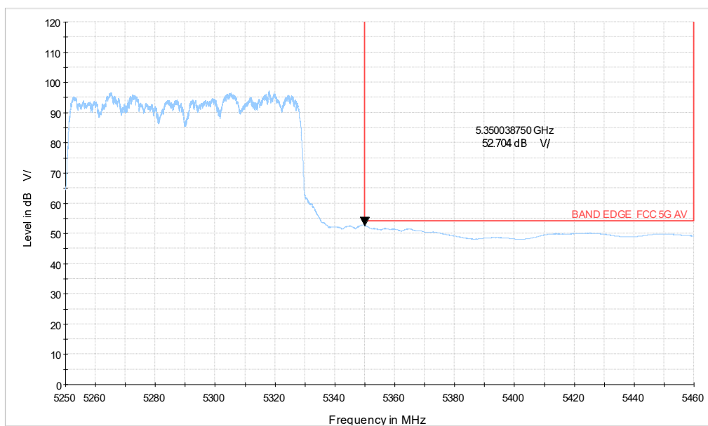
5G WIFI_ac80 CH58_5.25-5.46GHz_AV
