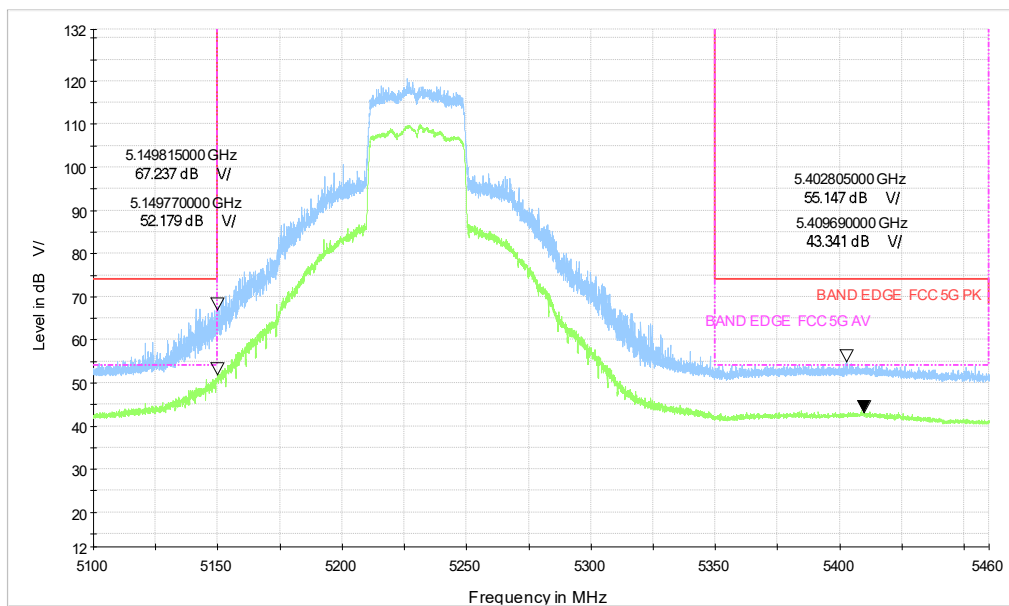
5G WIFI_ax40 CH46_5.1-5.46GHz_MCS0
