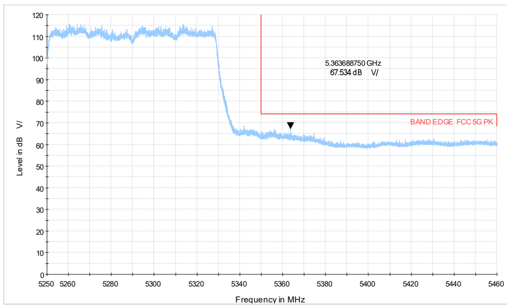
ax80-996TONE_CH58_5.25-5.46GHz_PK
