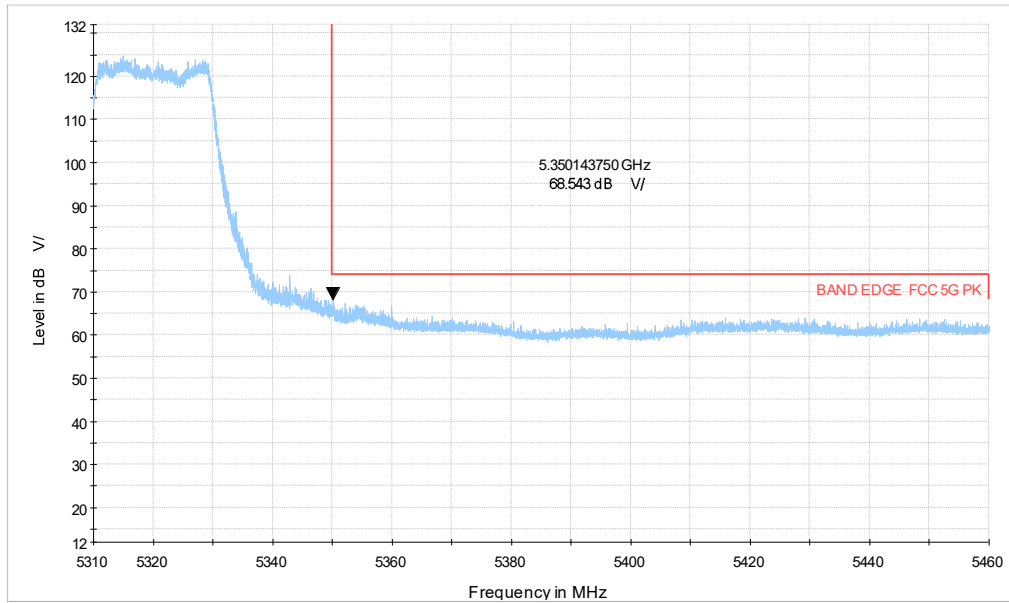
5G WIFI_ax20 CH64_5.31-5.46GHz_PK
