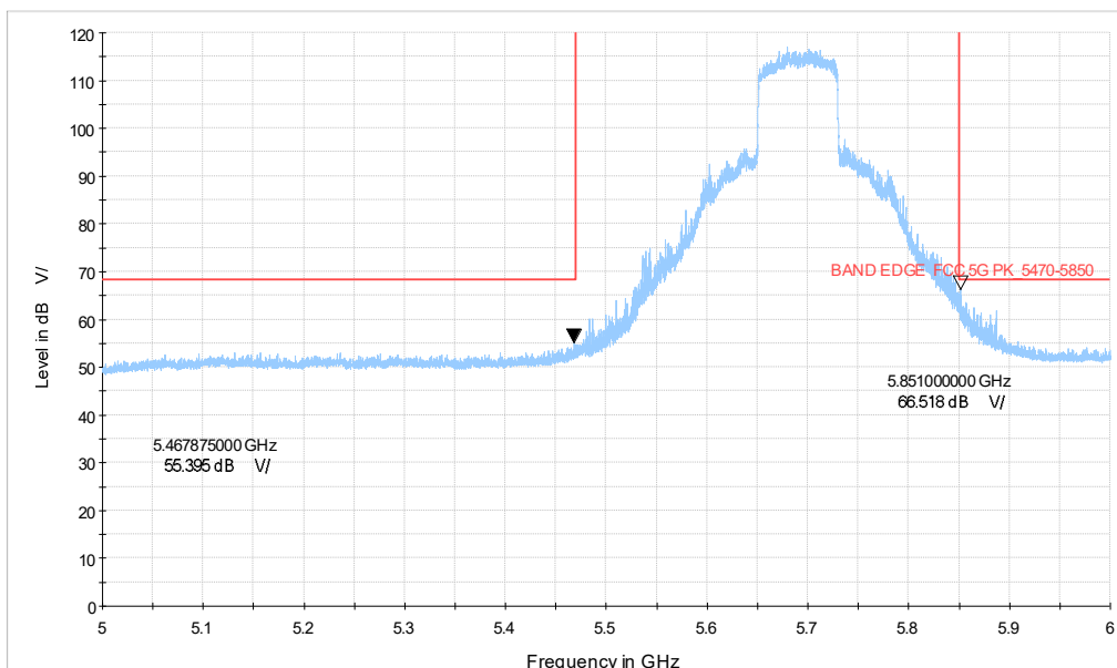
5G WIFI_ax80 CH138_5-6GHz_MCS0
