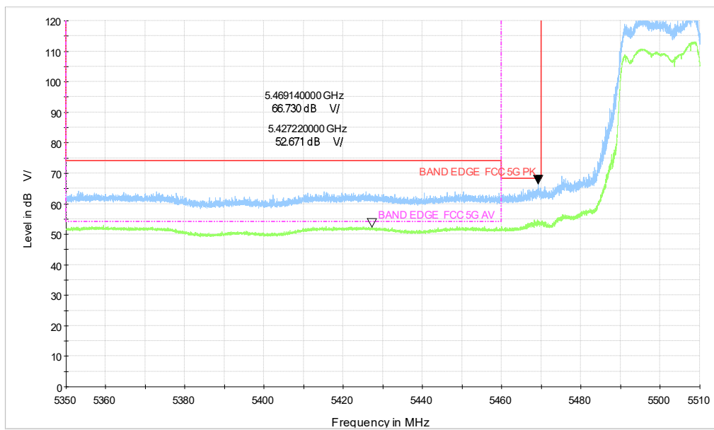
5G WIFI_ax20 CH100_5.35-5.51GHz
