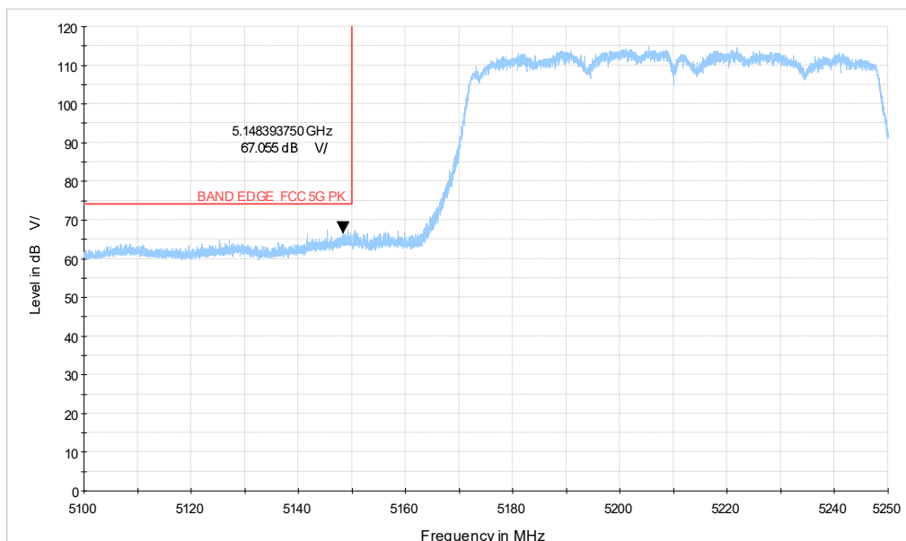
5G WIFI_ac80 CH42_5.1-5.25GHz_PK
