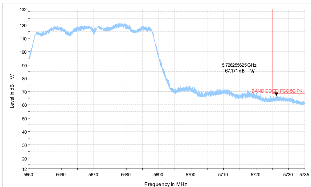
5G WIFI_n40 CH134_5.65-5.735GHz
