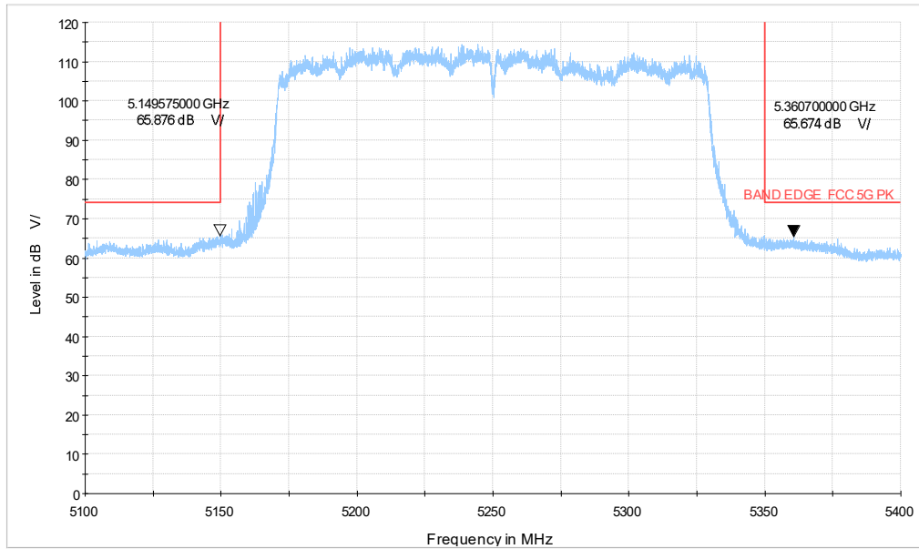
5G WIFI_ax160 CH50_5.1-5.4GHz_PK
