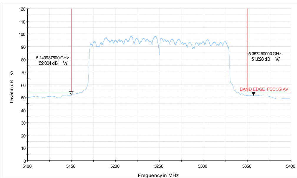
5G WIFI_ax160 CH50_5.1-5.4GHz_AV
