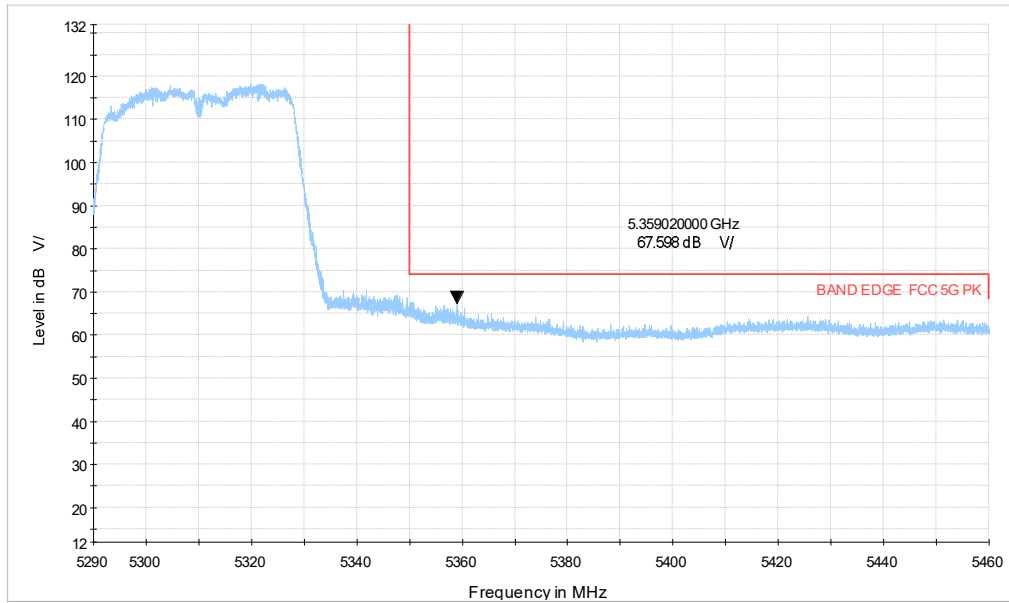
5G WIFI_n40 CH62_5.29-5.46GHz_PK
