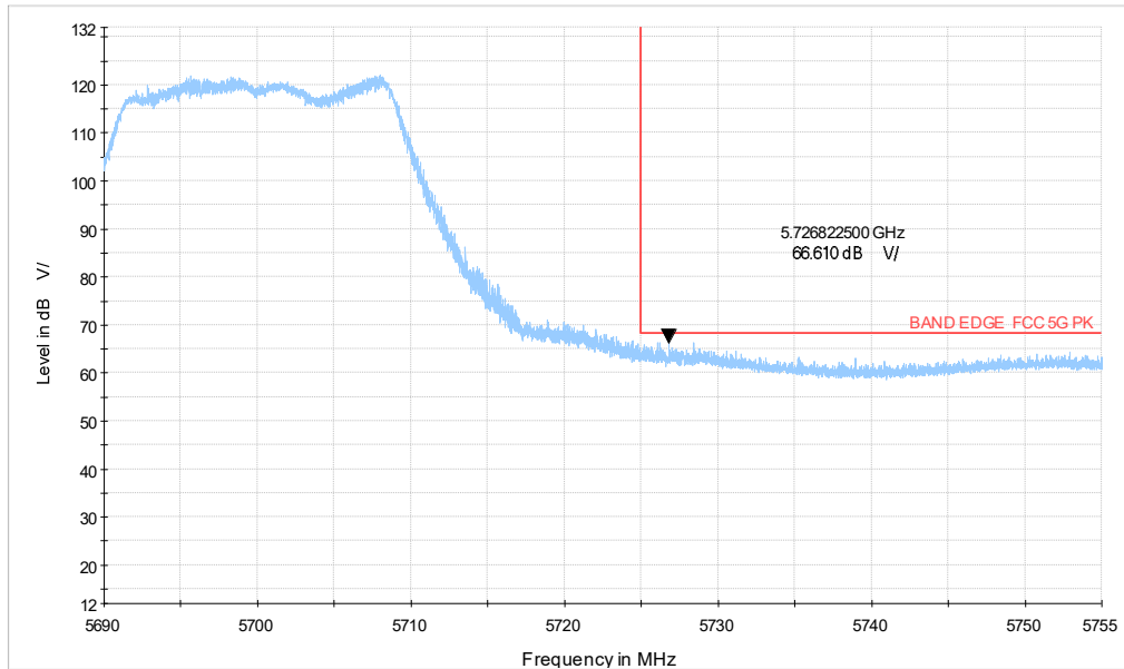
5G WIFI_n20 CH140_5.69-5.755GHz
