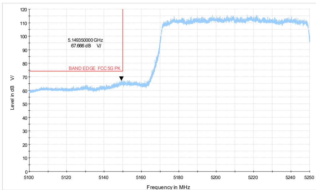
ax80-996TONE_CH42_5.1-5.25GHz_PK
