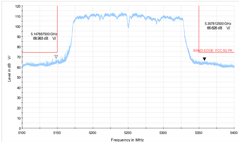
5G WIFI_ac160 CH50_5.1-5.4GHz_PK
