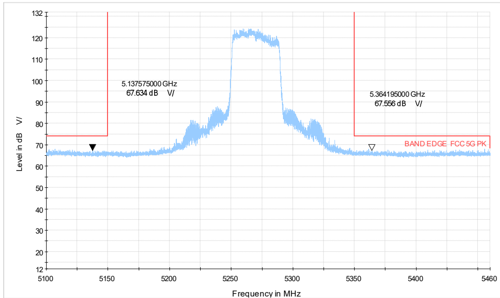
ax40-484TONE_CH54_5.1-5.46GHz_PK
