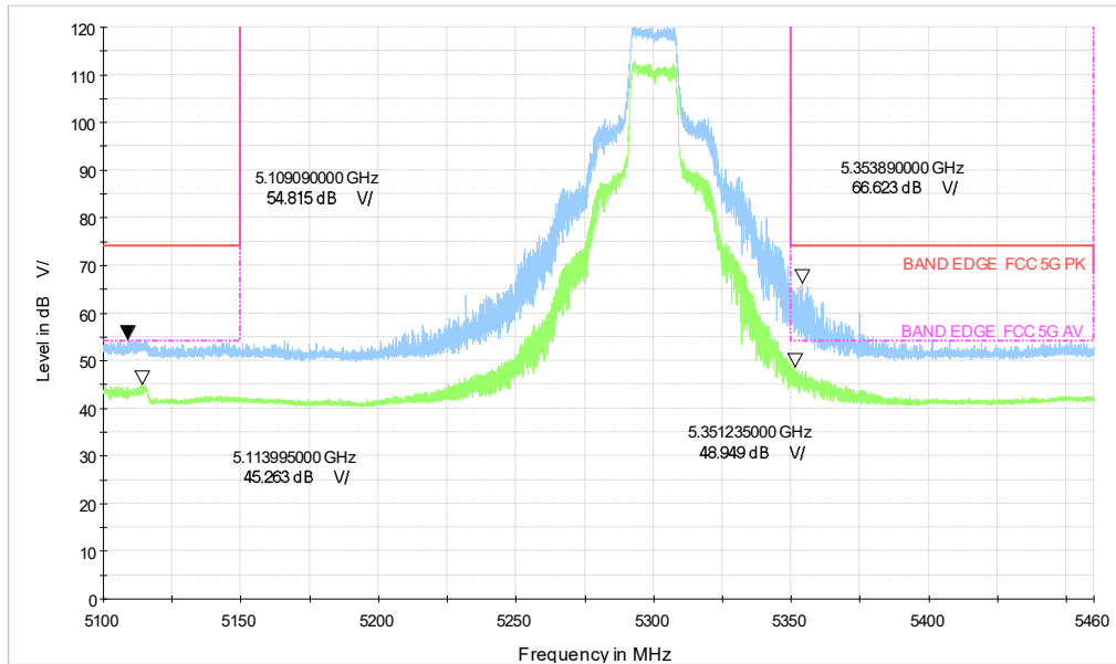
5G WIFI_a CH60_5.1-5.46GHz_6M
