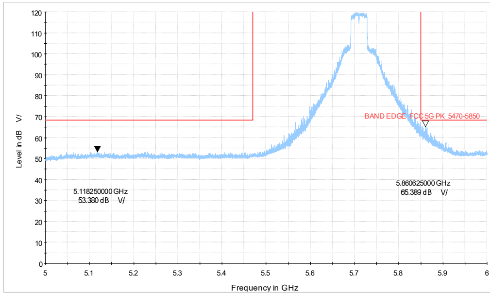
5G WIFI_n40 CH142_5-6GHz_MCS0
