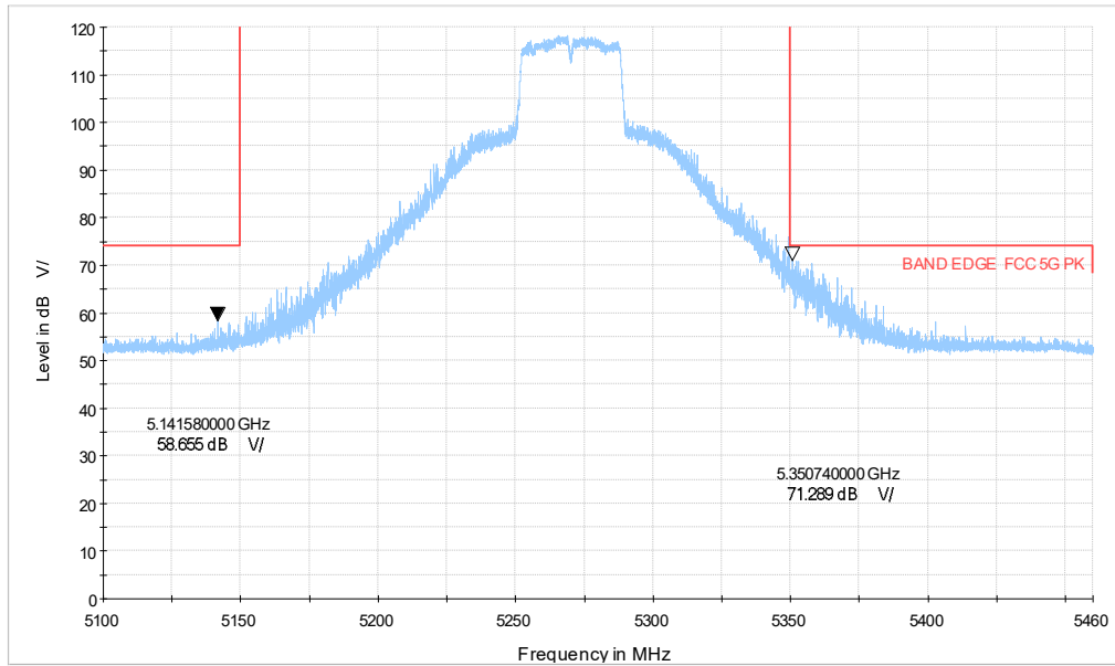
5G WIFI_n40 CH54_5.1-5.46GHz_MCS0_PK
