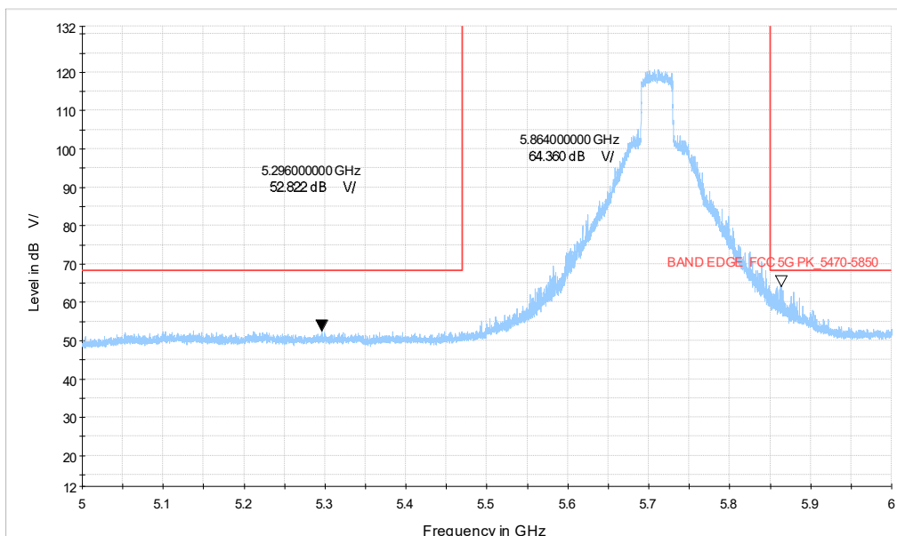
5G WIFI_ax40 CH142_5-6GHz_MCS0
