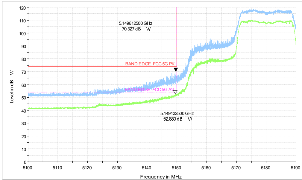
5G WIFI_n20 CH36_5.1-5.19GHz_MCS0
