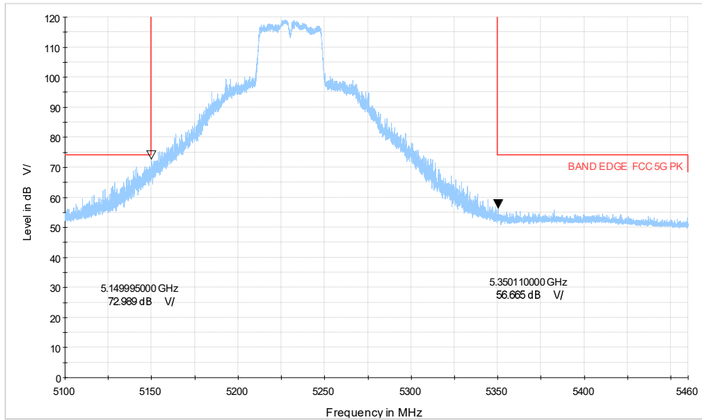
5G WIFI_n40 CH46_5.1-5.46GHz_MCS0_PK
