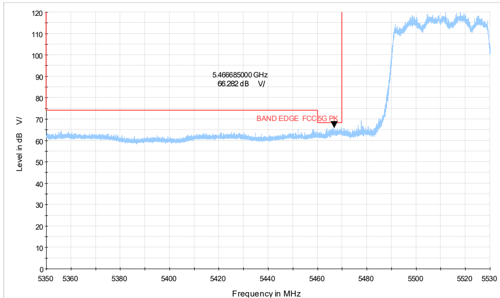
5G WIFI_ax40 CH102_5.35-5.53GHz_PK
