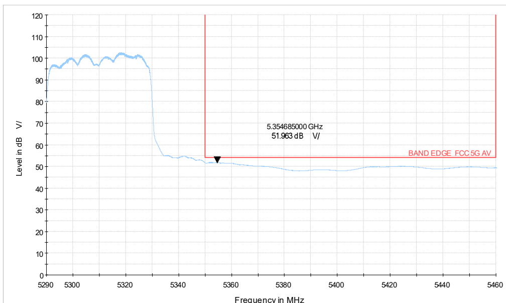
5G WIFI_ax40 CH62_5.29-5.46GHz_AV
