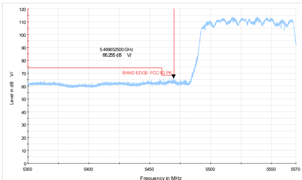
5G WIFI_ac80 CH106_5.35-5.57GHz_PK
