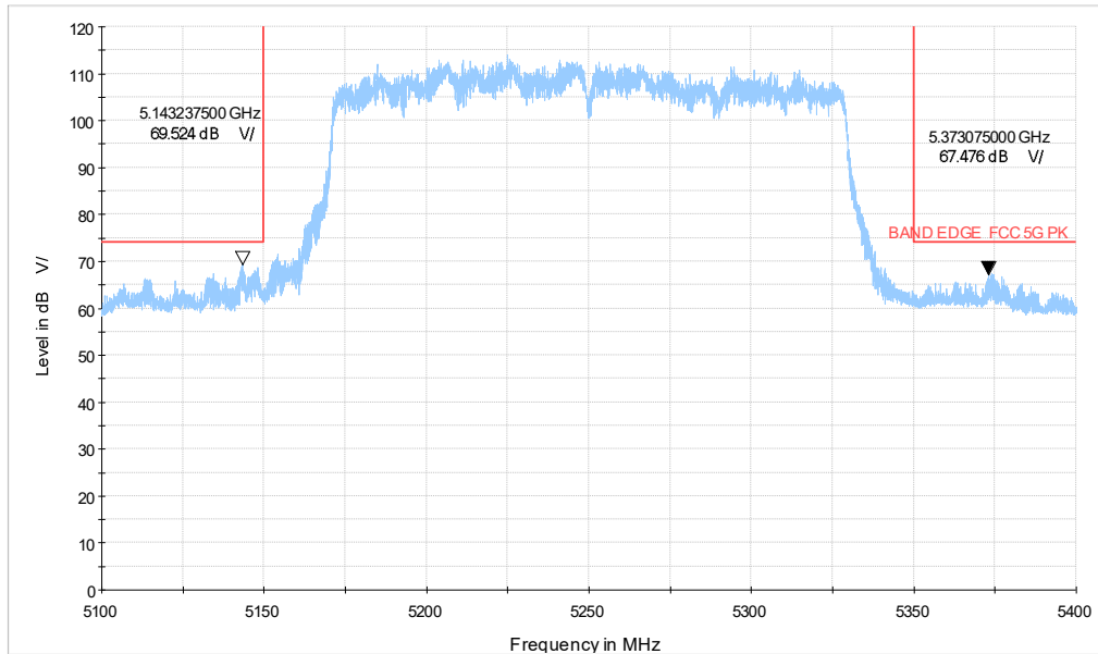
ax160-996x2TONE_CH50_5.1-5.4GHz_PK
