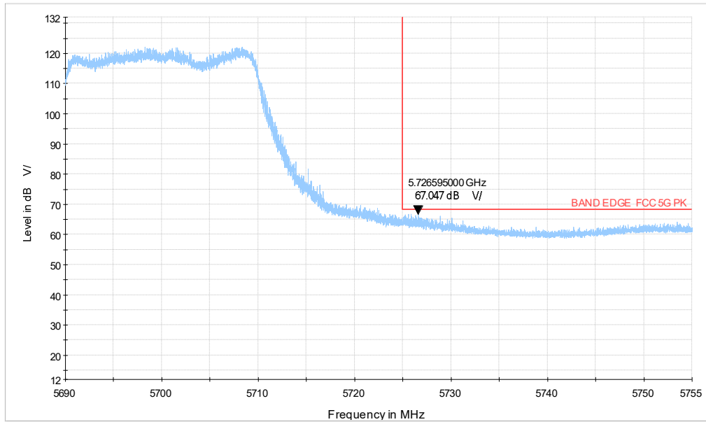
5G WIFI_ax20 CH140_5.69-5.755GHz
