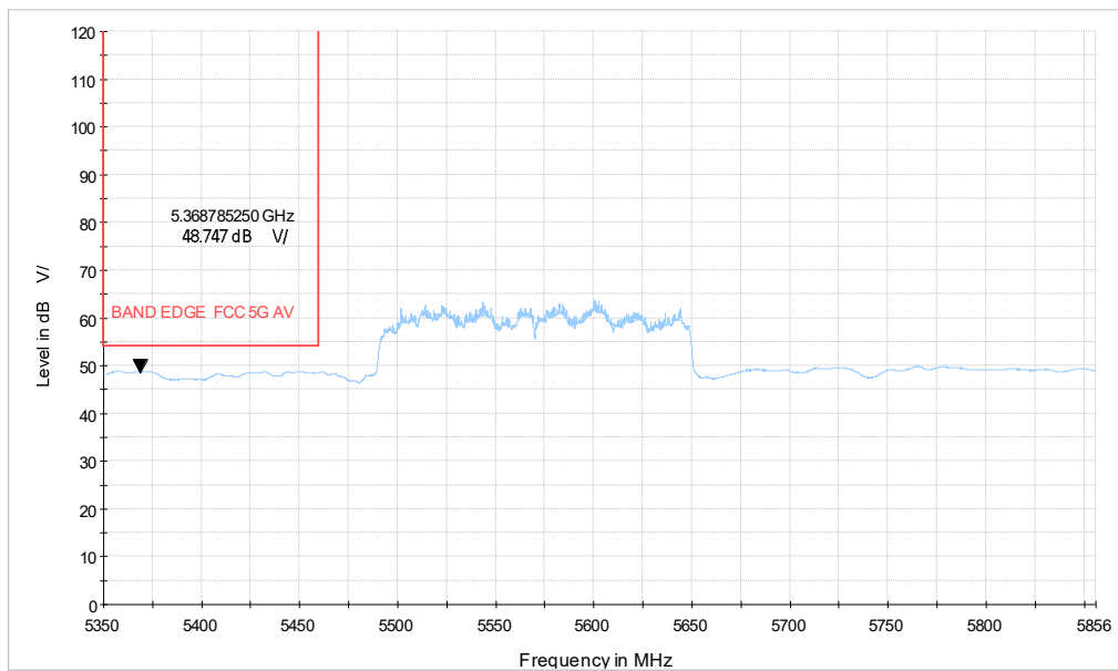
ax160-996x2TONE_CH114_5.35-5.856GHz_AV
