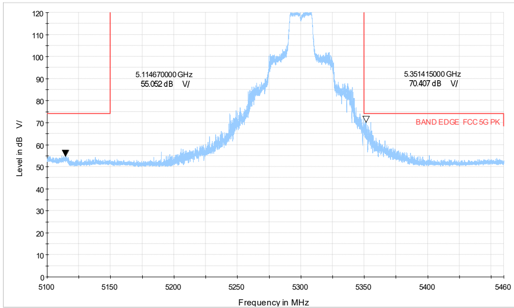
5G WIFI_n20 CH60_5.1-5.46GHz_MCS0
