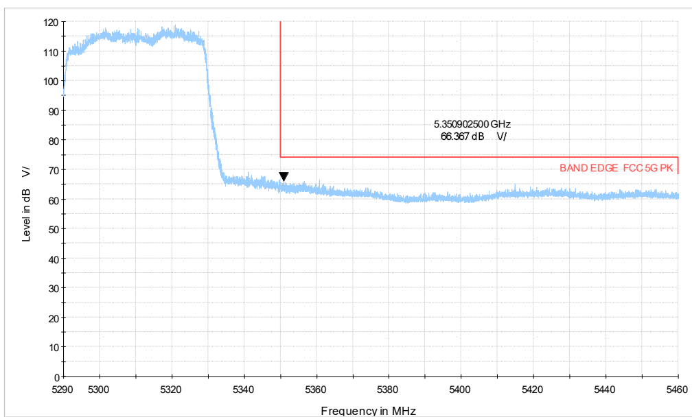
5G WIFI_ax40 CH62_5.29-5.46GHz_PK
