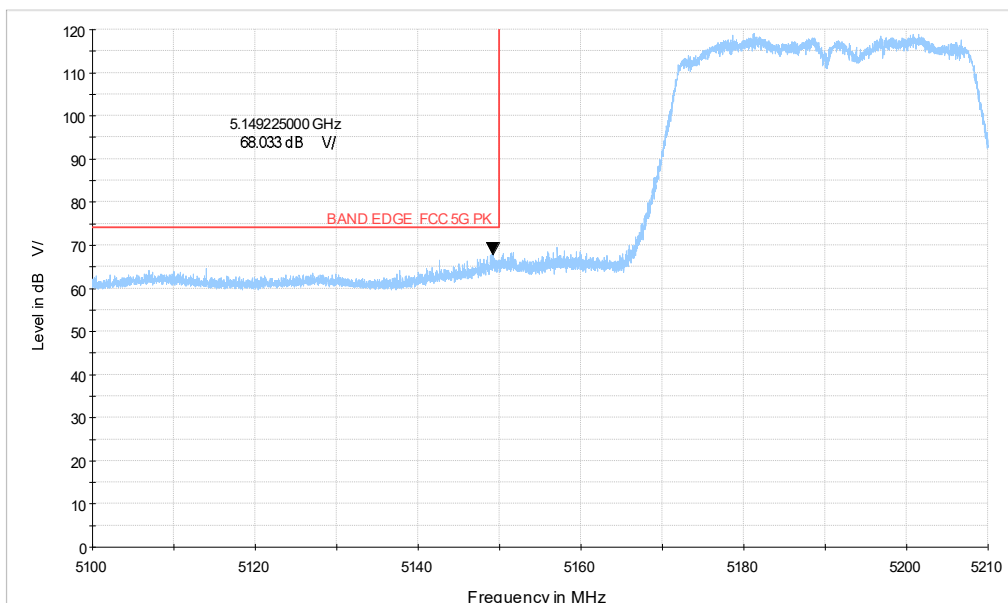
5G WIFI_n40 CH38_5.1-5.21GHz_PK
