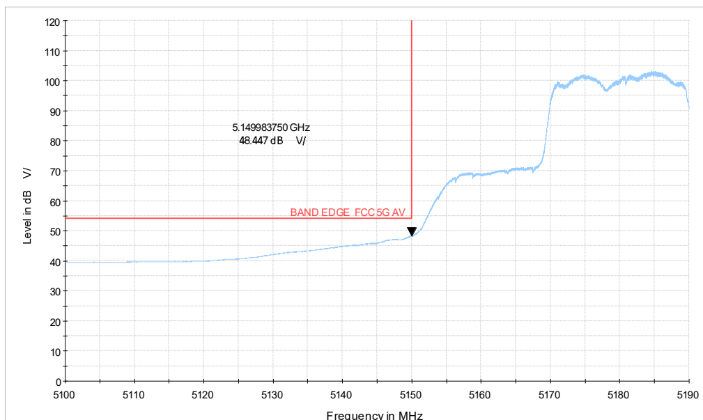
5G WIFI_ax20 CH36_5.1-5.19GHz_MCS0_AV
