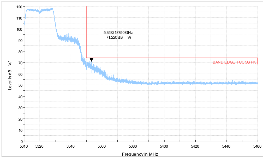
5G WIFI_n20 CH64_5.31-5.46GHz_MCS0_PK
