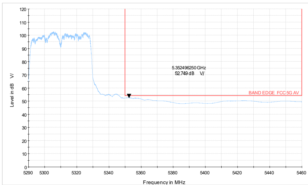
5G WIFI_n40 CH62_5.29-5.46GHz_AV
