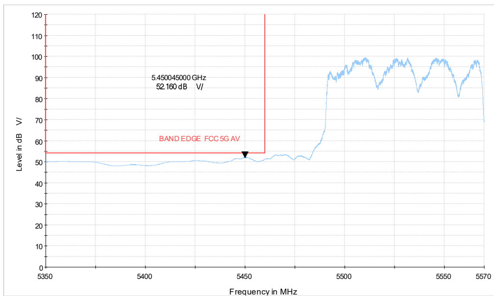
5G WIFI_ac80 CH106_5.35-5.57GHz_AV
