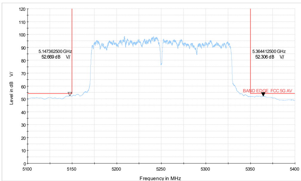
5G WIFI_ac160 CH50_5.1-5.4GHz_AV
