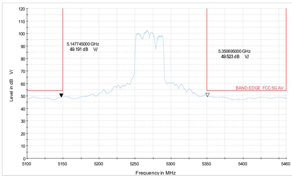
ax40-484TONE_CH54_5.1-5.46GHz_AV
