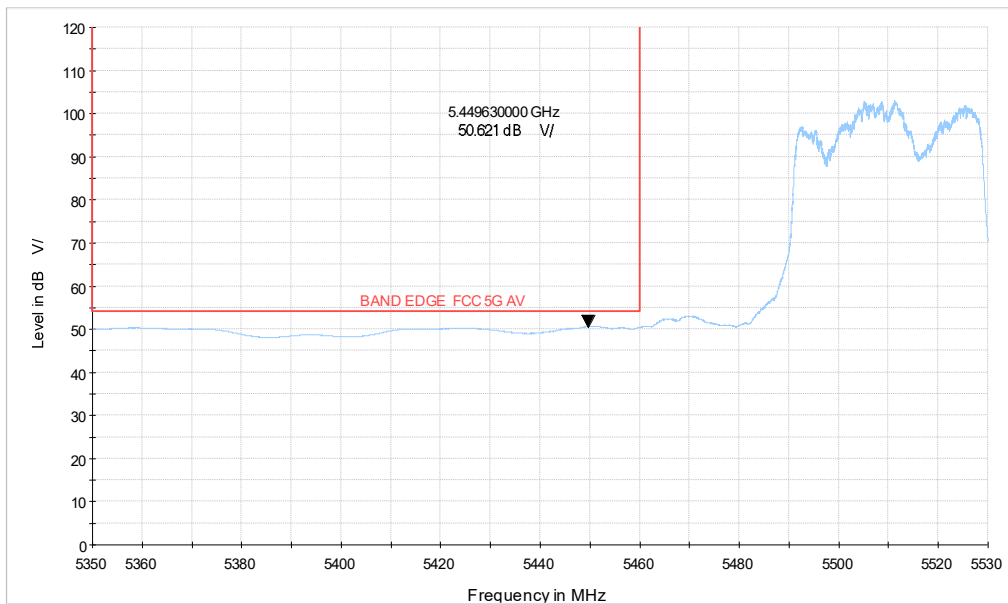
5G WIFI_n40 CH102_5.35-5.53GHz_AV
