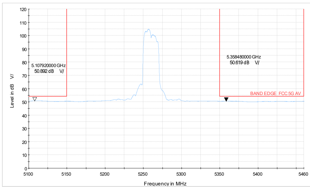
ax20-242TONE_CH52_5.1-5.46GHz_AV
