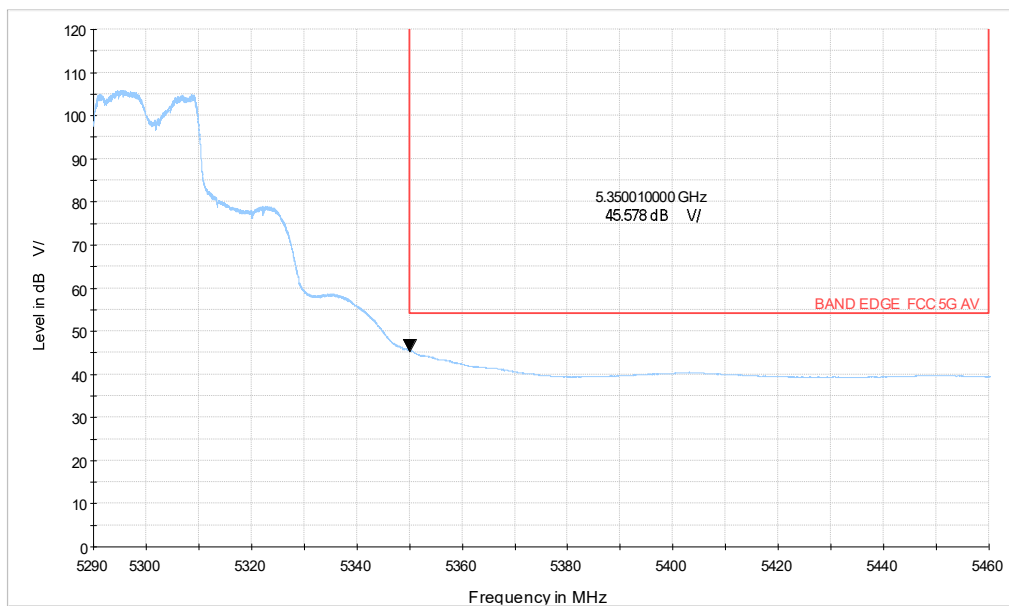
5G WIFI_ax20 CH60_5.29-5.46GHz_MCS0_AV
