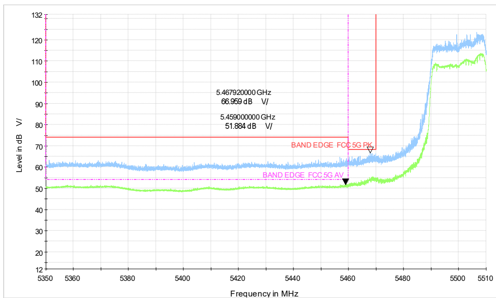
ax20-242TONE_CH100_5.35-5.51GHz
