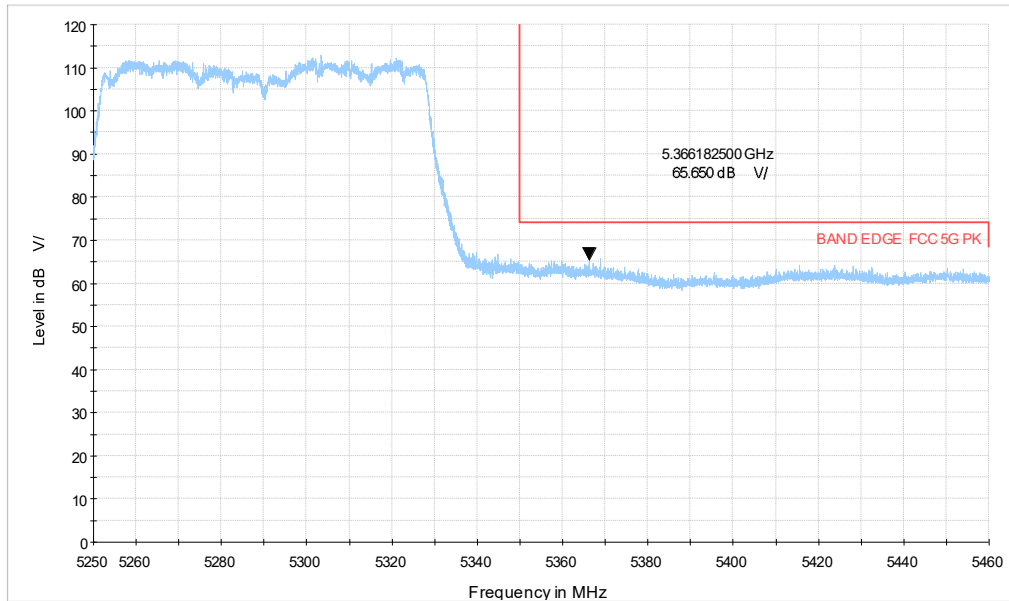
5G WIFI_ac80 CH58_5.25-5.46GHz_PK
