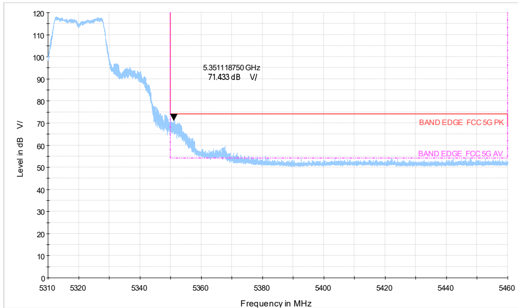
5G WIFI_a CH64_5.31-5.46GHz_6M_PK
