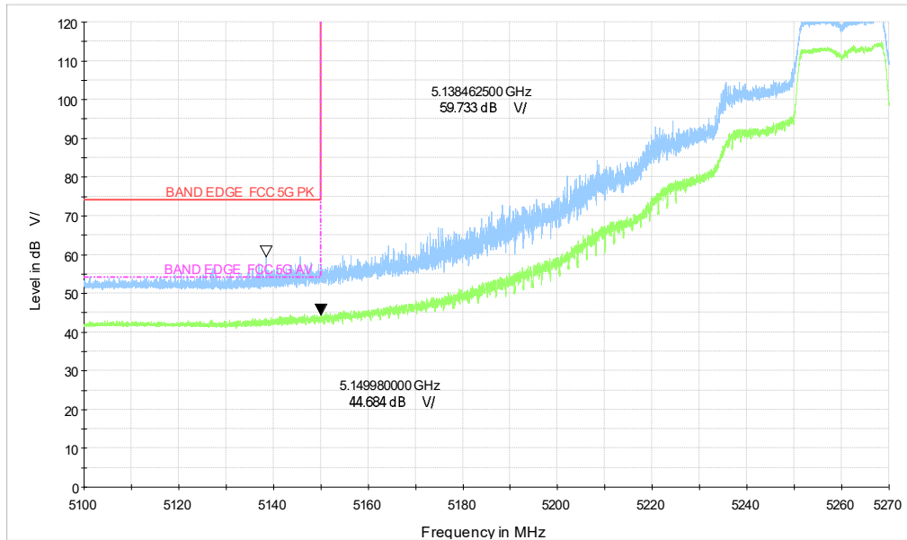
5G WIFI_n20 CH52_5.1-5.27GHz_MCS0
