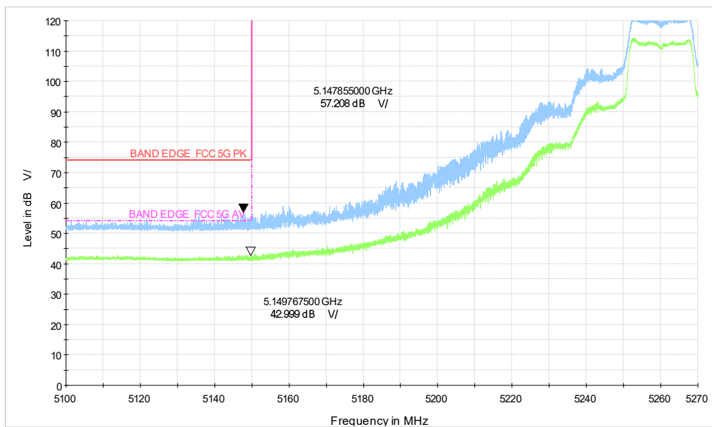
5G WIFI_a CH52_5.1-5.27GHz_6M
