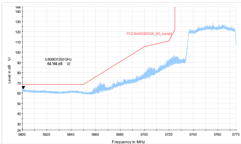
ax40-484TONE_CH151_5.6-5.775GHz_0412
