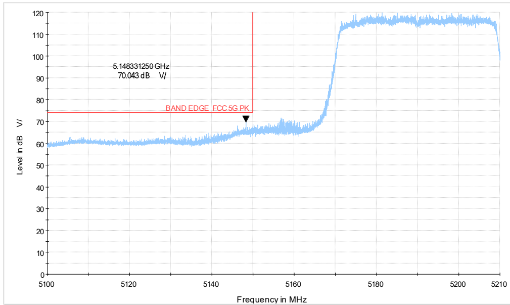
ax40-484TONE_CH38_5.1-5.21GHz_PK
