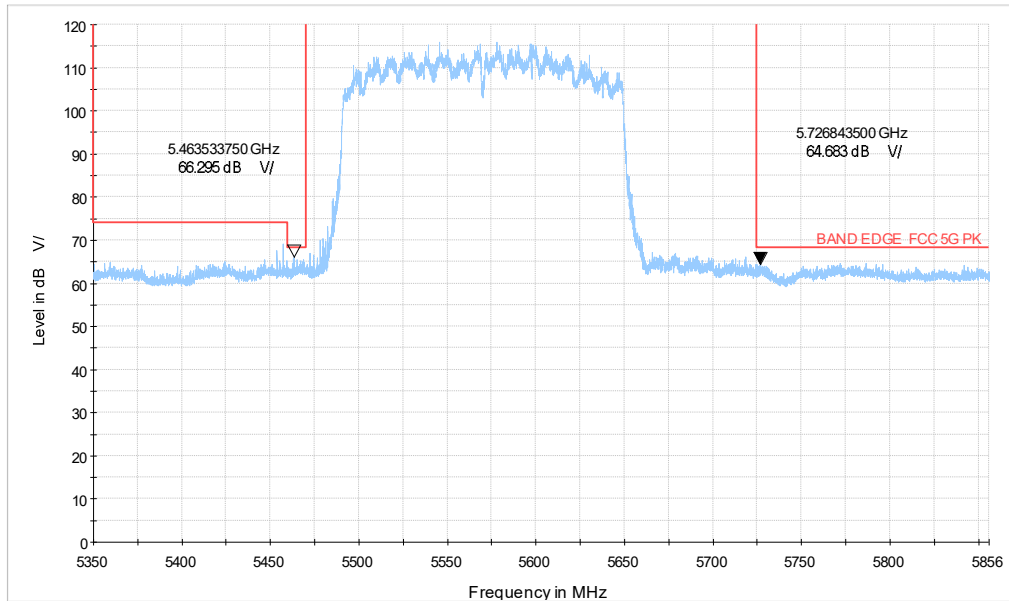
5G WIFI_ax160 CH114_5.35-5.856GHz_PK
