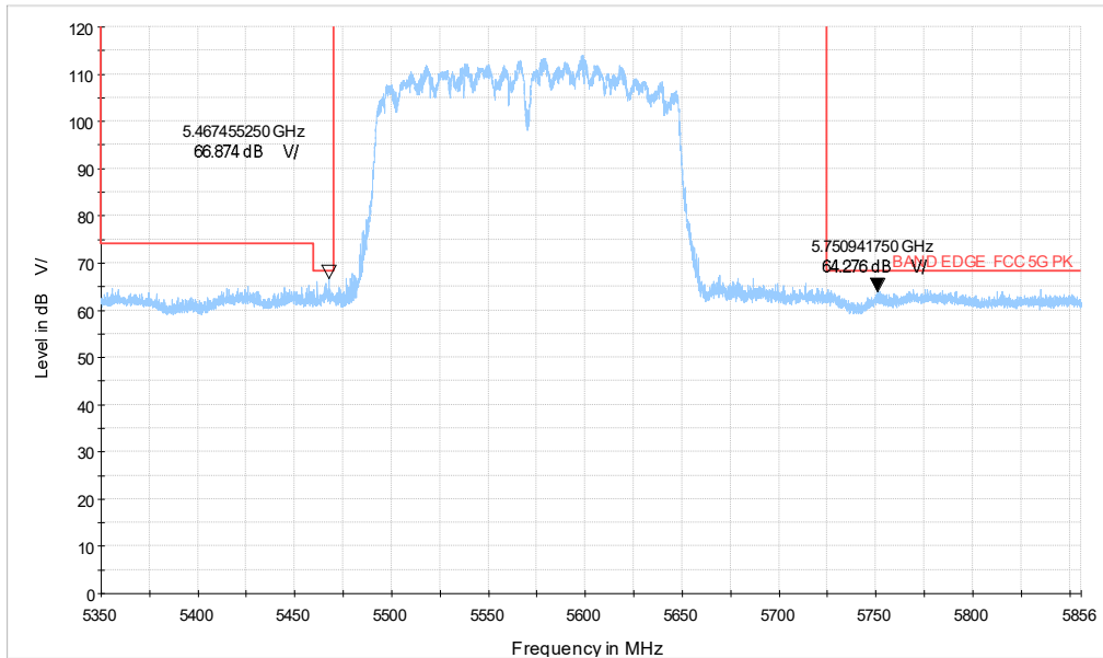
5G WIFI_ac160 CH114_5.35-5.856GHz_PK
