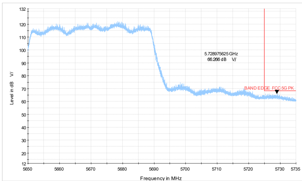
5G WIFI_ax40 CH134_5.65-5.735GHz
