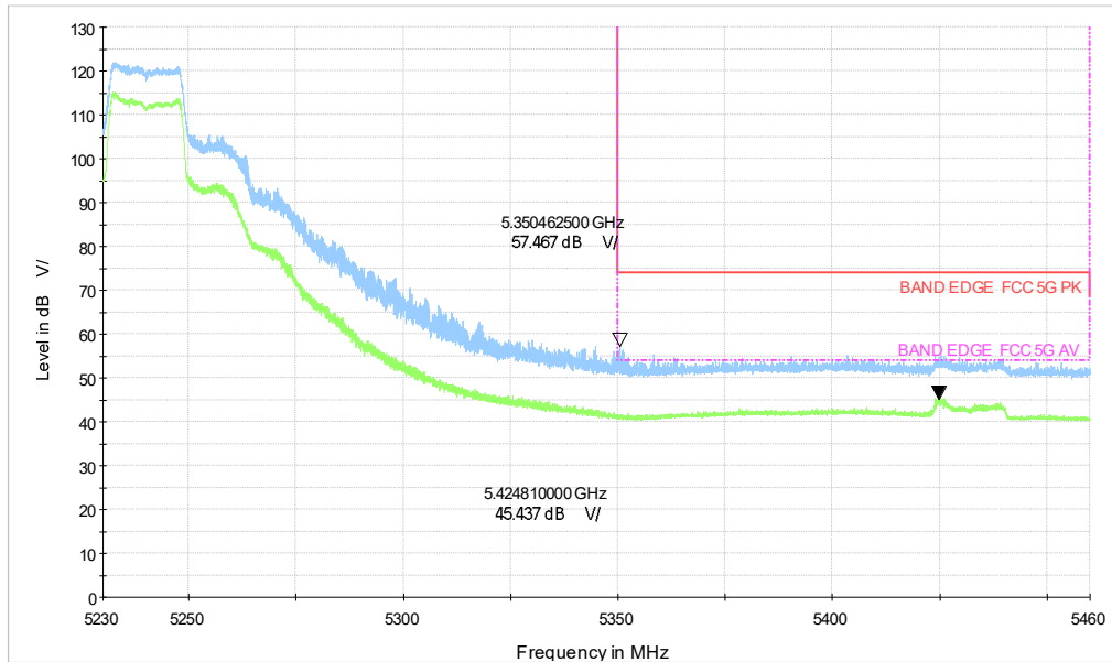
5G WIFI_a CH48_5.23-5.46GHz_6M
