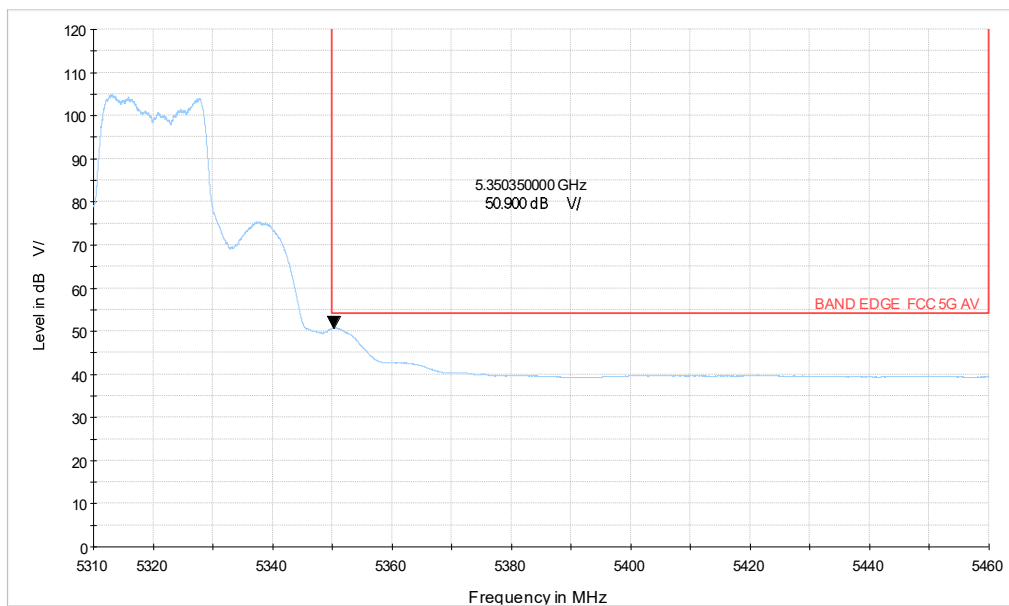
5G WIFI_a CH64_5.31-5.46GHz_6M_AV
