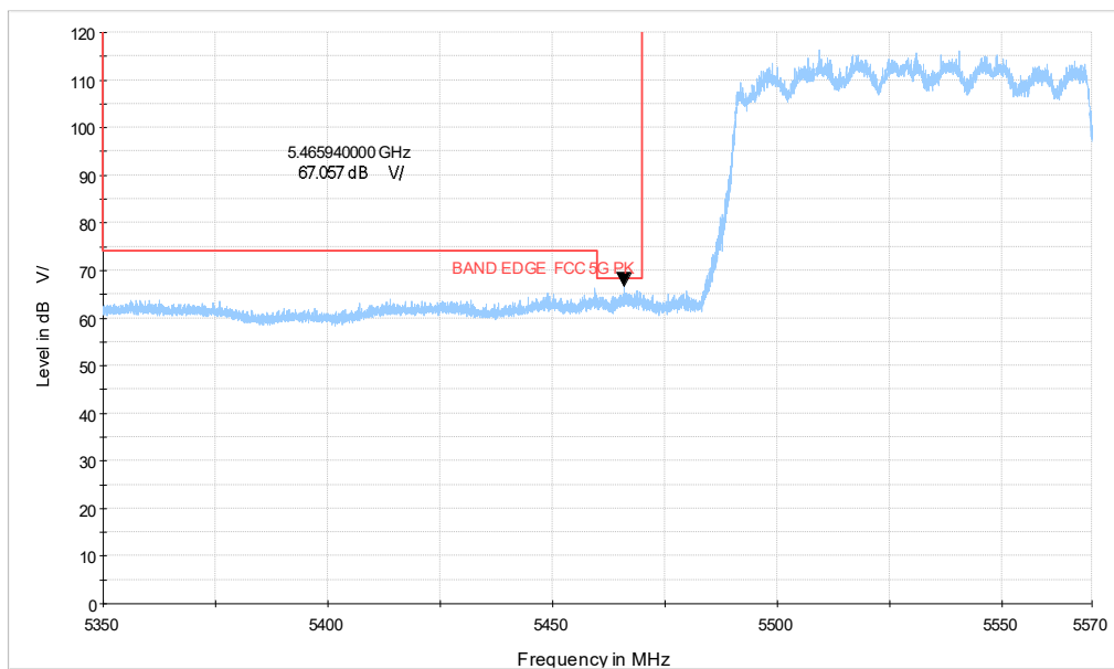
5G WIFI_ax80 CH106_5.35-5.57GHz_PK
