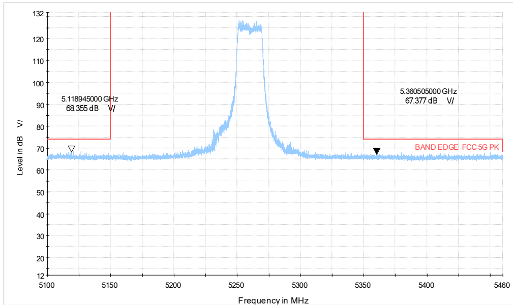
ax20-242TONE_CH52_5.1-5.46GHz_PK
