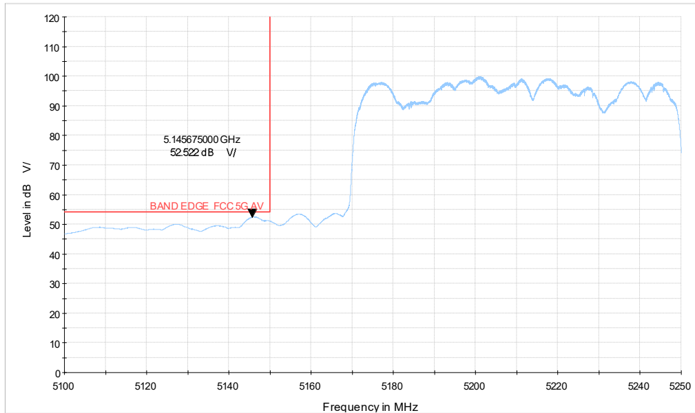
ax80-996TONE_CH42_5.1-5.25GHz_AV
