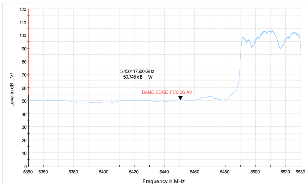
5G WIFI_ax40 CH102_5.35-5.53GHz_AV
