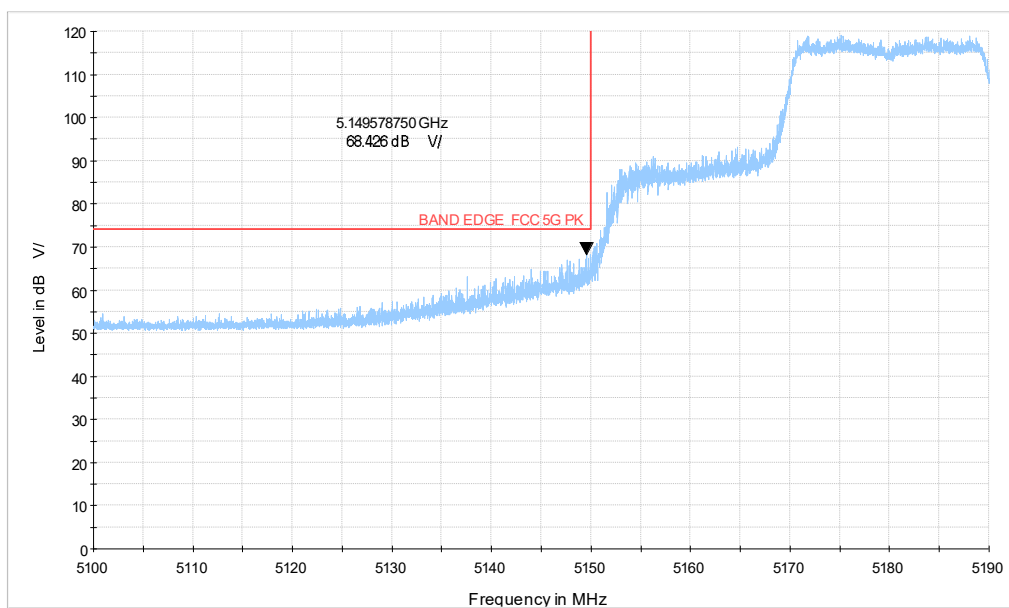
5G WIFI_ax20 CH36_5.1-5.19GHz_MCS0_PK
