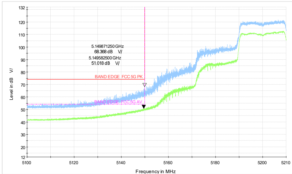
5G WIFI_ax20 CH40_5.1-5.21GHz_MCS0
