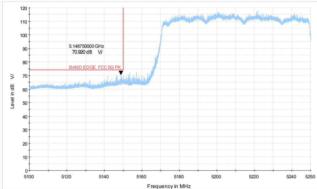
5G WIFI_ax80 CH42_5.1-5.25GHz_PK
