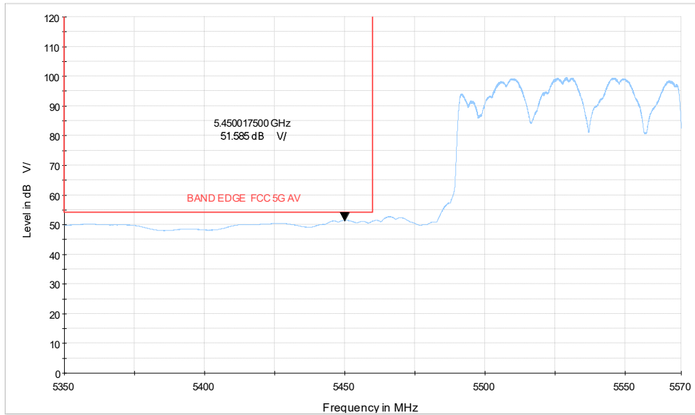
5G WIFI_ax80 CH106_5.35-5.57GHz_AV
