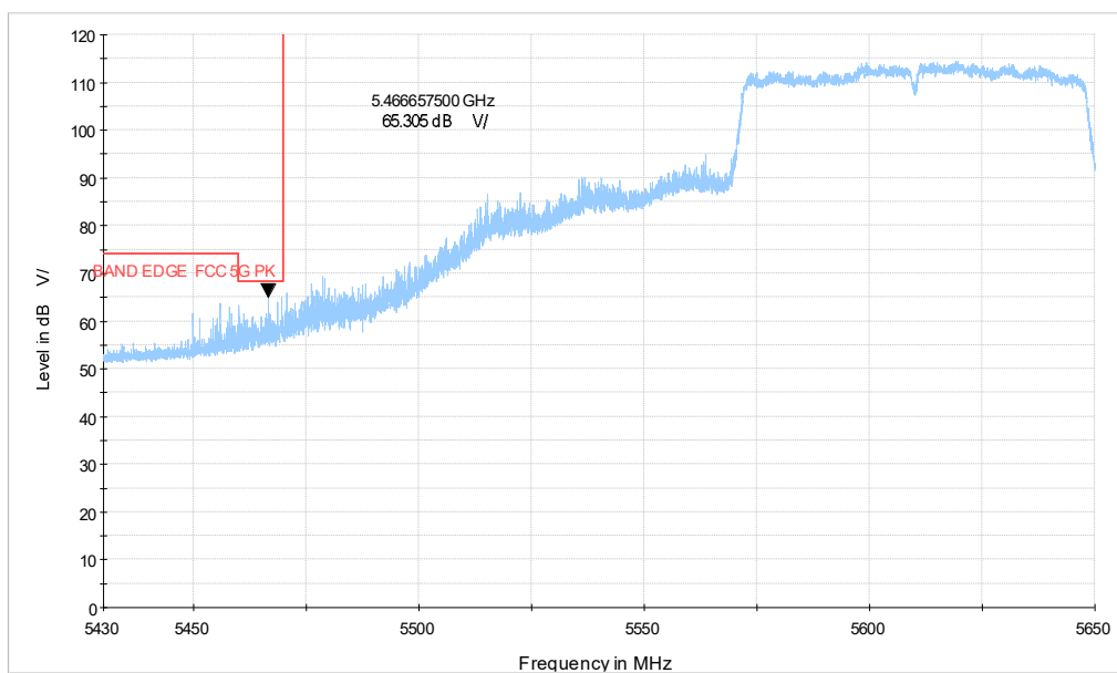
5G WIFI_ac80 CH122_5.43-5.65GHz_MCS0
