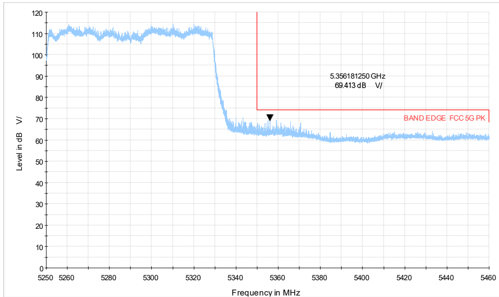
5G WIFI_ax80 CH58_5.25-5.46GHz_PK
