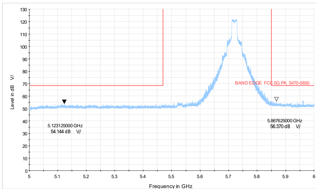
5G WIFI_n20 CH144_5-6GHz_MCS0
