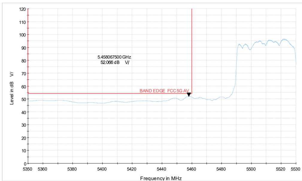
ax40-484TONE_CH102_5.35-5.53GHz_AV
