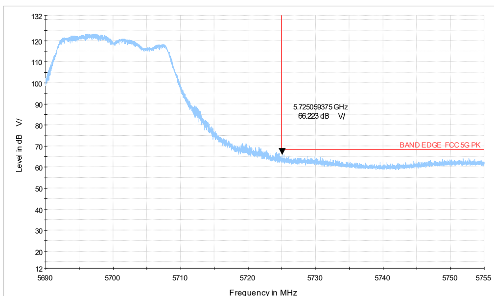
5G WIFI_a CH140_5.69-5.755GHz
