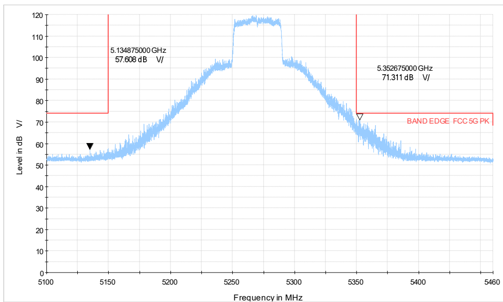
5G WIFI_ax40 CH54_5.1-5.46GHz_MCS0_PK
