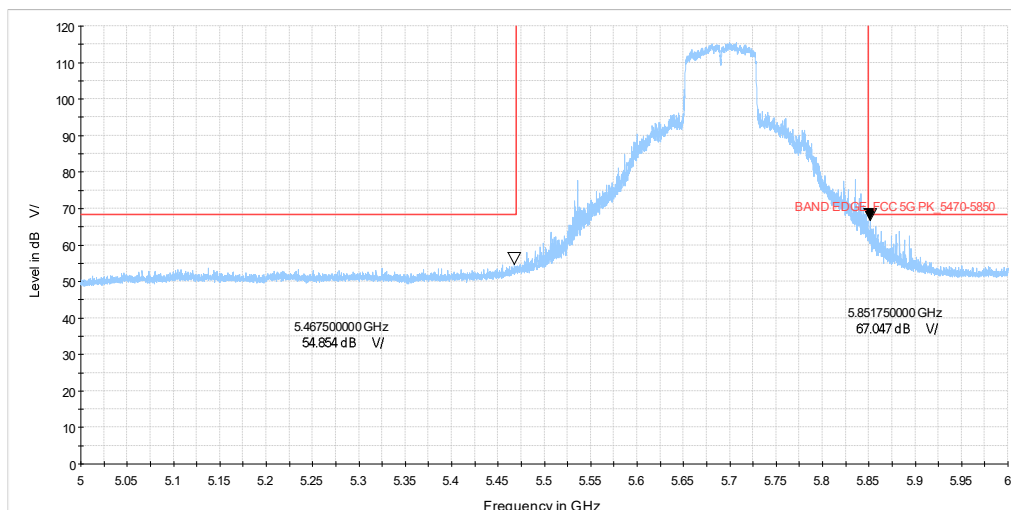
5G WIFI_ac80 CH138_5-6GHz_MCS0
