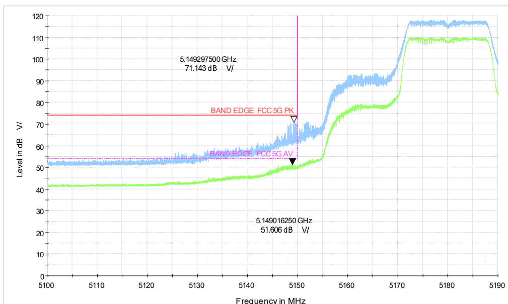
5G WIFI_a CH36_5.1-5.19GHz_6M
