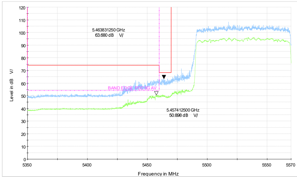
5G WIFI_ax80 CH106_5.35-5.57GHz_MCS0
