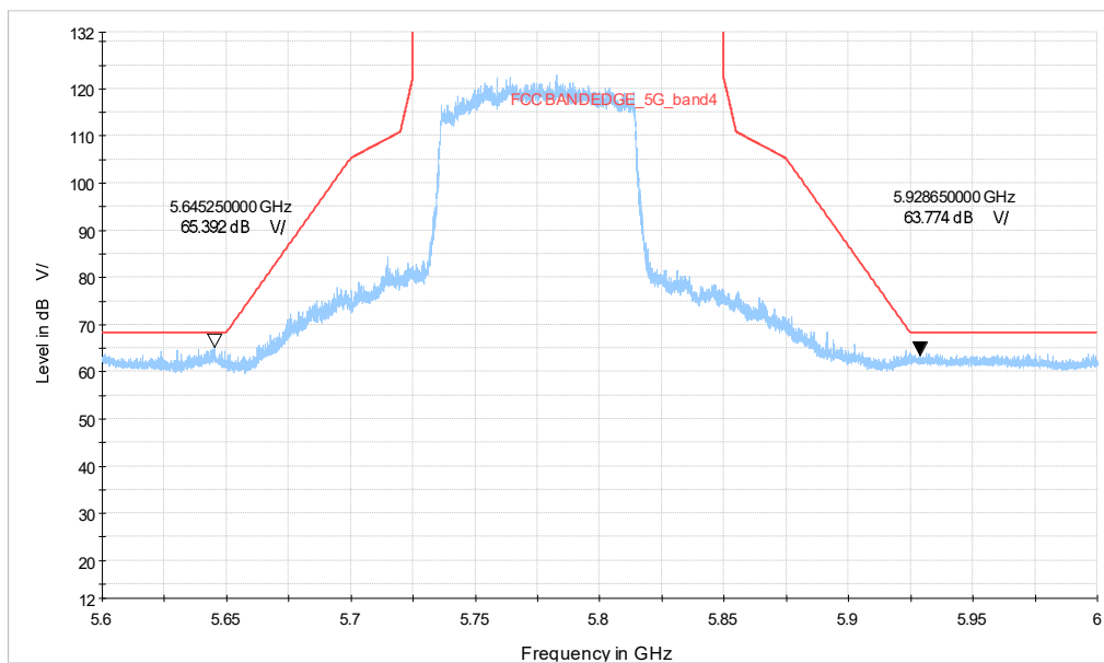
ax80-996TONE_CH155_5.6-6GHz
