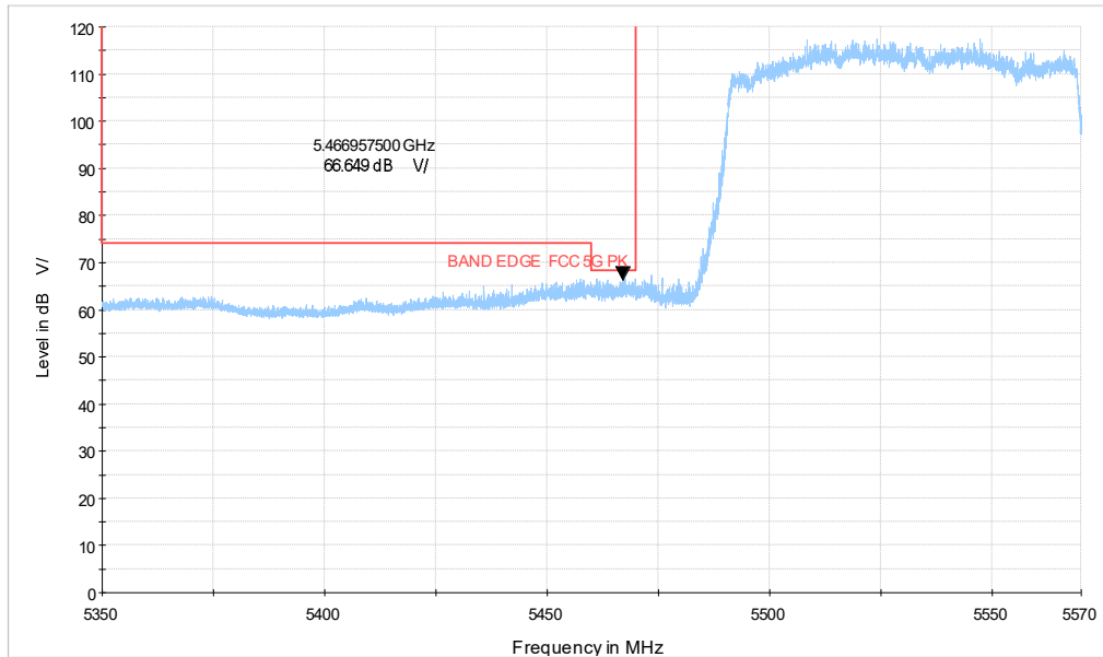
ax80-996TONE_CH106_5.35-5.57GHz_PK
