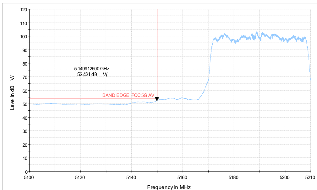
5G WIFI_n40 CH38_5.1-5.21GHz_AV
