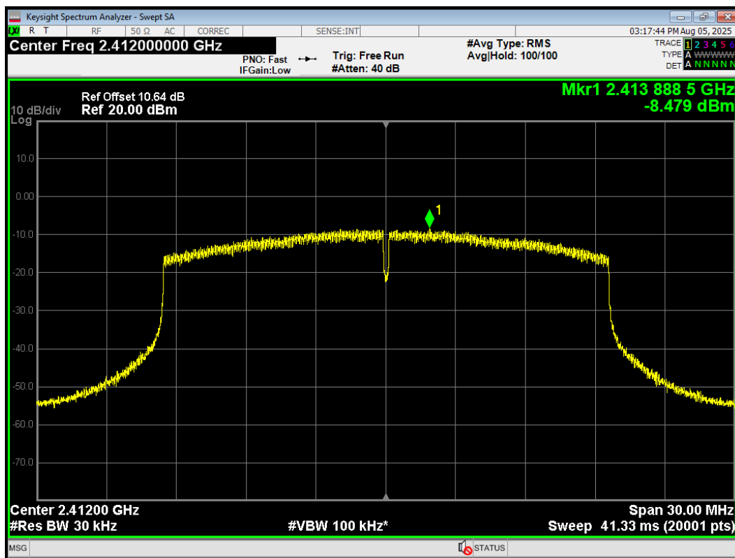
PSD 802.11ax(HE20)Index61 2412MHz Ant2
