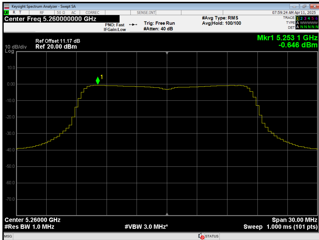
PSD 802.11a 5260MHz Ant2
