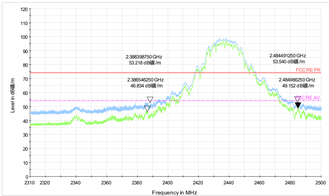
WiFi-2.4GBX54_b_CH6_2.31-2.50GHz_PK+AV
