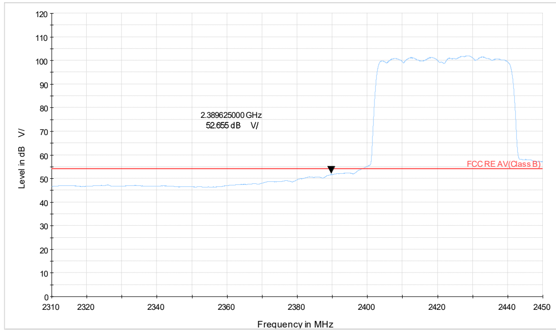
WiFi-2.4Gax40_CH3_2.31-2.45GHz_AV
