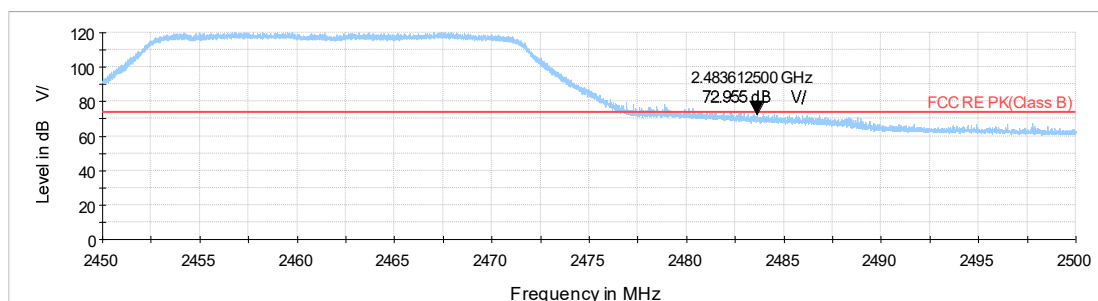
WiFi-2.4Gax20_CH11_2.45-2.5GHz_PK
