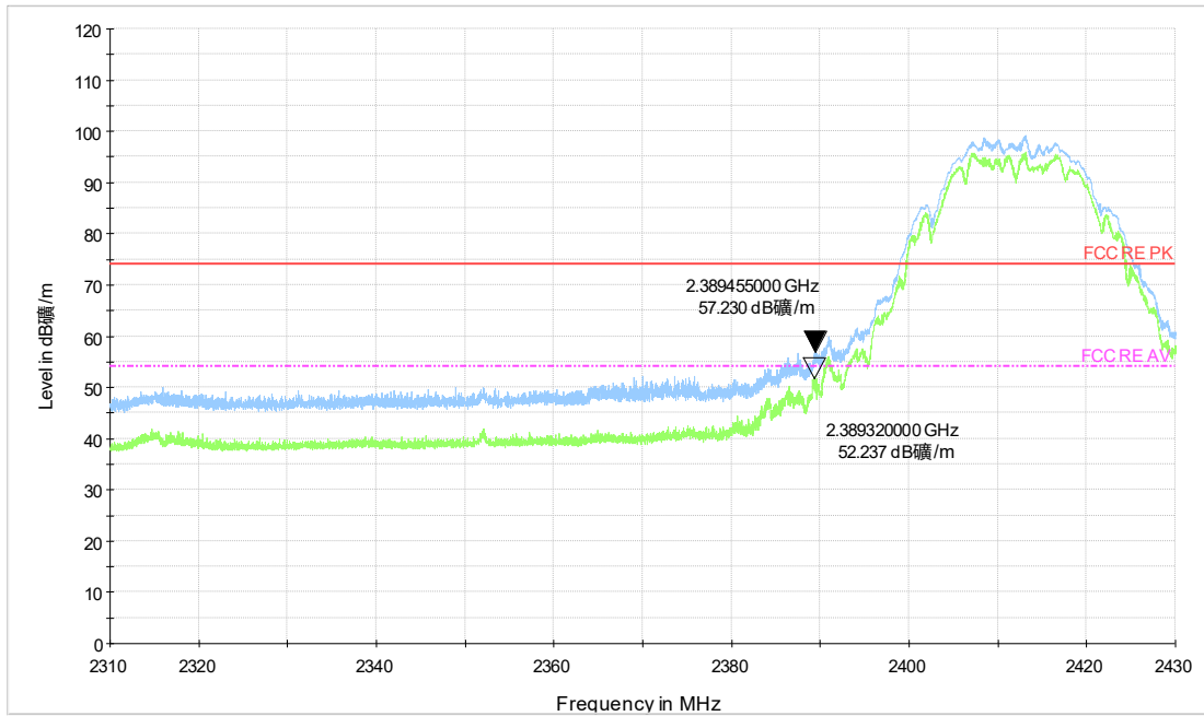
WiFi-2.4GBX54_b_CH1_2.31-2.43GHz_PK+AV
