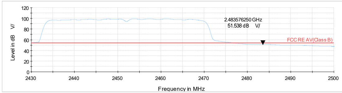
WiFi-2.4Gn40_CH9_2.43-2.5GHz_AV
