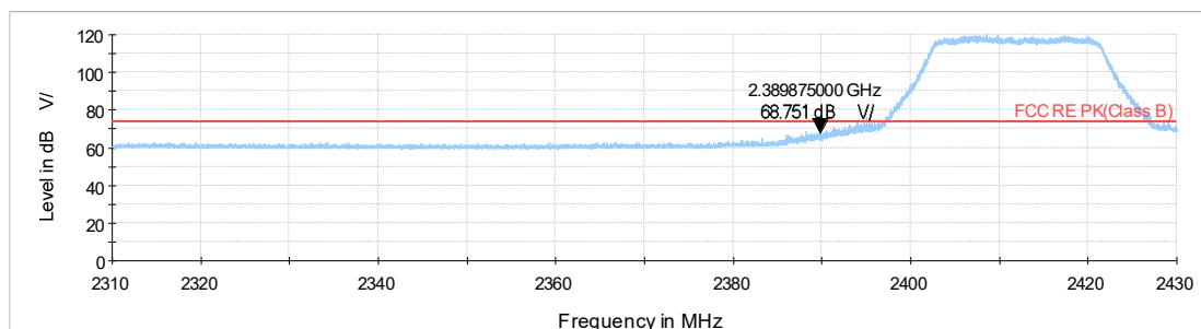
WiFi-2.4Gax20_CH1_2.31-2.43GHz_PK
