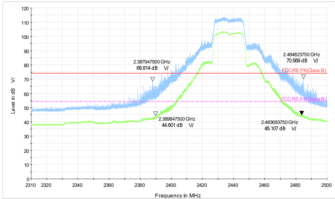
WiFi-2.4GBX54_ax20_CH6_2.31-2.5GHz_PK+AV
