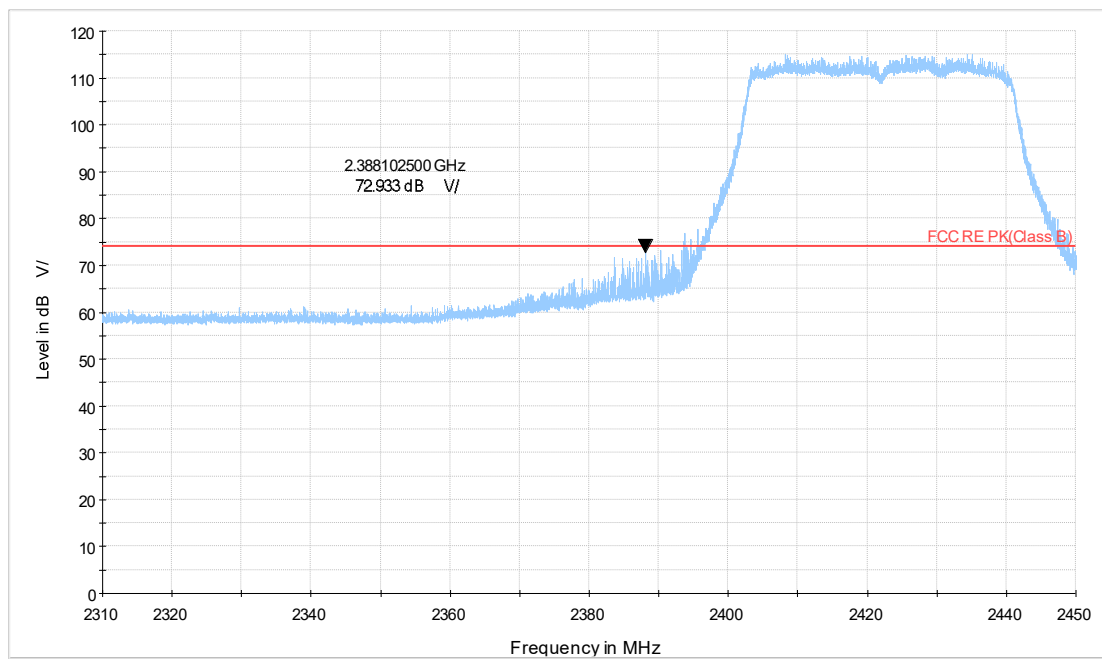
WiFi-2.4Gax40_CH3_2.31-2.45GHz_PK
