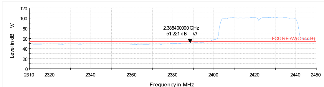
WiFi-2.4Gn40_CH3_2.31-2.45GHz_AV
