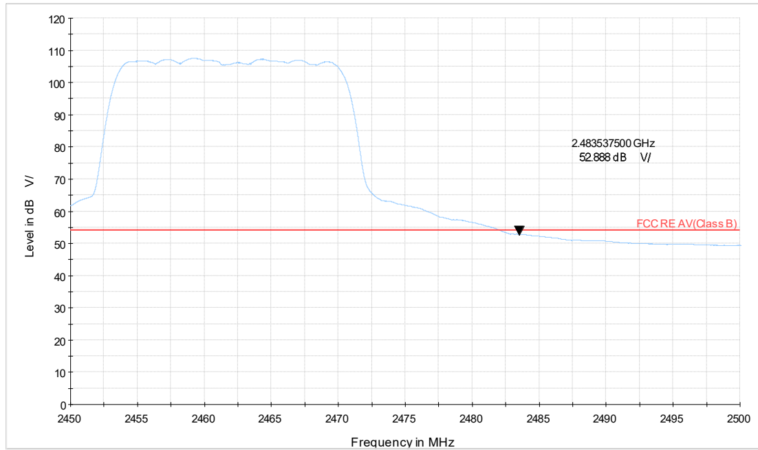
WiFi-2.4Gg_CH11_2.45-2.5GHz_AV
