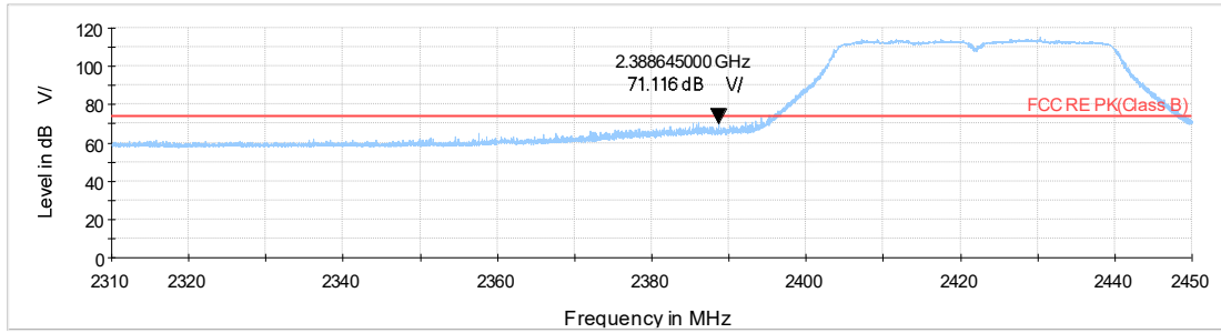
WiFi-2.4Gn40_CH3_2.31-2.45GHz_PK
