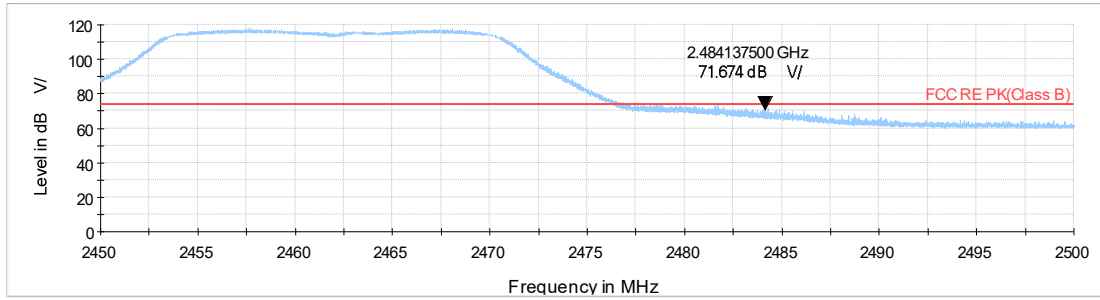
WiFi-2.4Gn20_CH11_2.45-2.5GHz_PK
