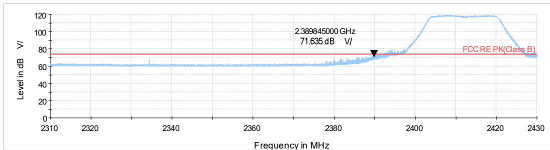
WiFi-2.4Gn20_CH1_2.31-2.43GHz_PK
