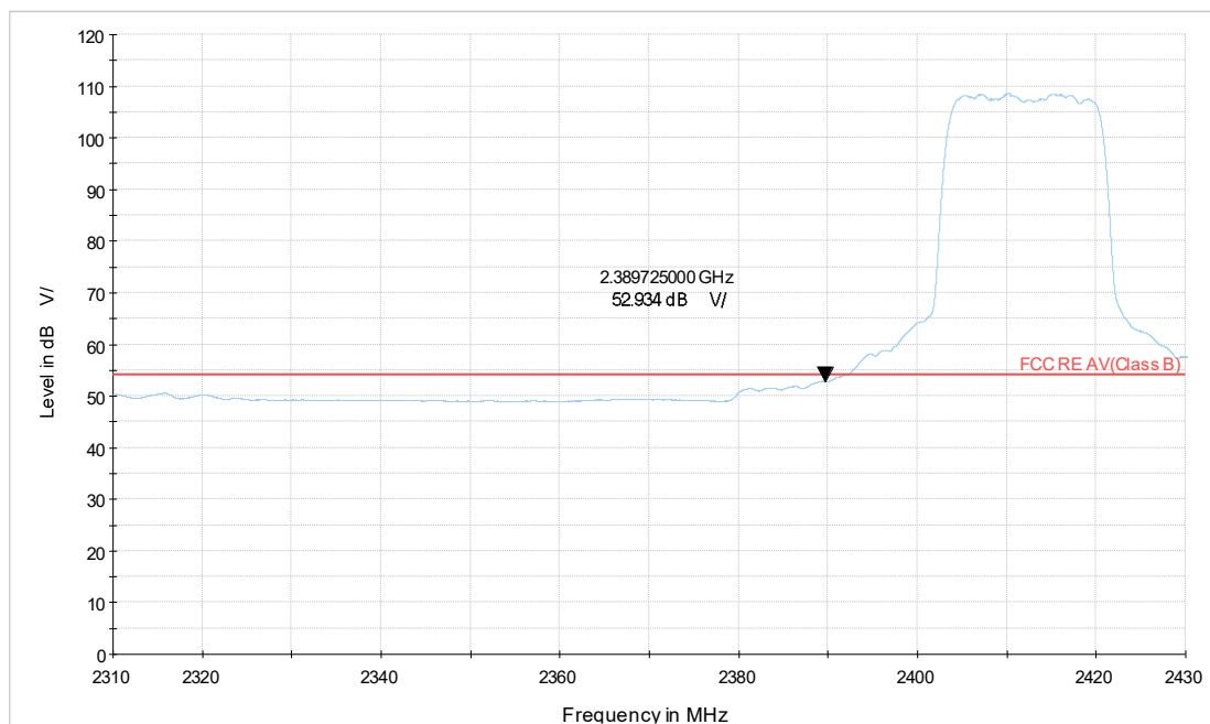
WiFi-2.4Gg_CH1_2.31-2.43GHz_AV
