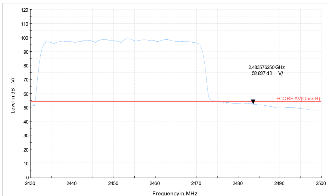
WiFi-2.4Gax40_CH9_2.43-2.5GHz_AV
