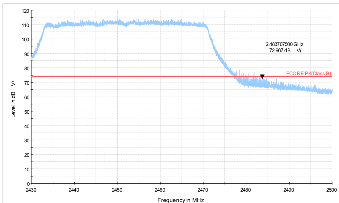
WiFi-2.4Gax40_CH9_2.43-2.5GHz_PK
