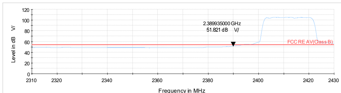
WiFi-2.4Gax20_CH1_2.31-2.43GHz_AV
