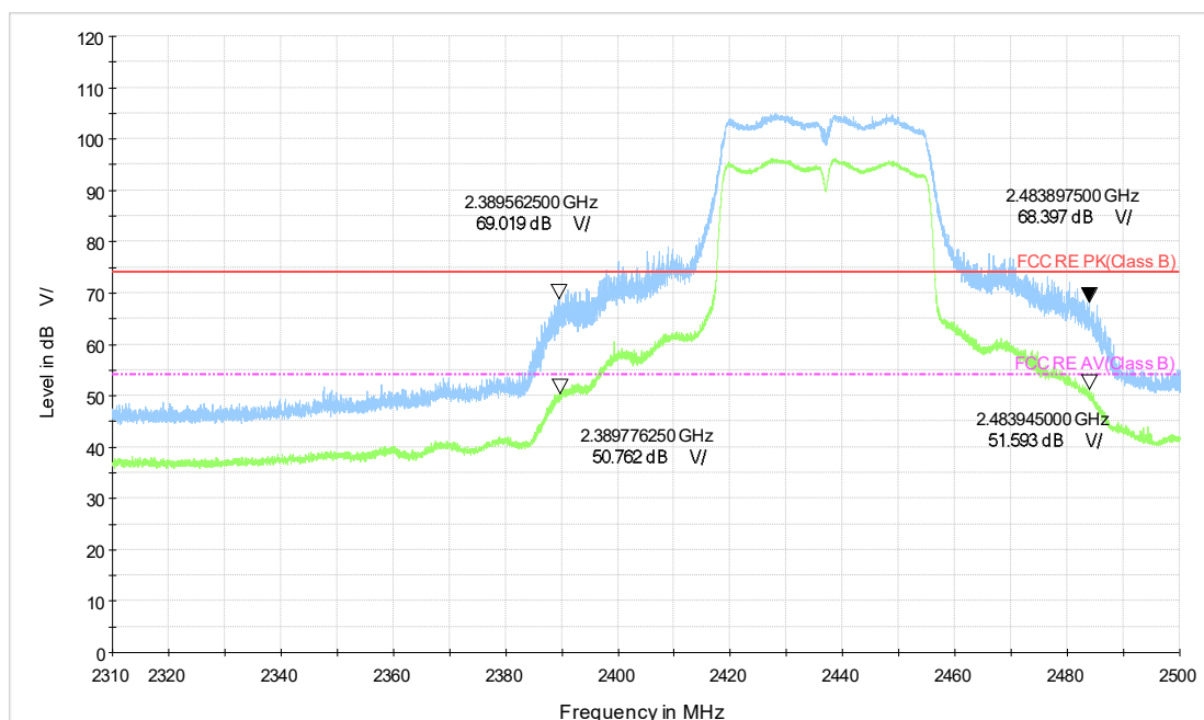
WiFi-2.4GBX54_n40_CH6_2.31-2.5GHz_PK+AV
