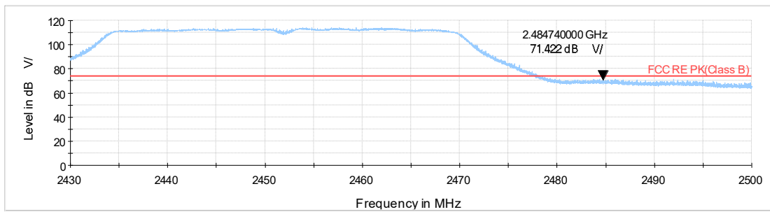
WiFi-2.4Gn40_CH9_2.43-2.5GHz_PK
