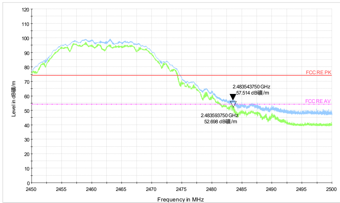
WiFi-2.4GBX54_b_CH11_2.45-2.5GHz_PK+AV
