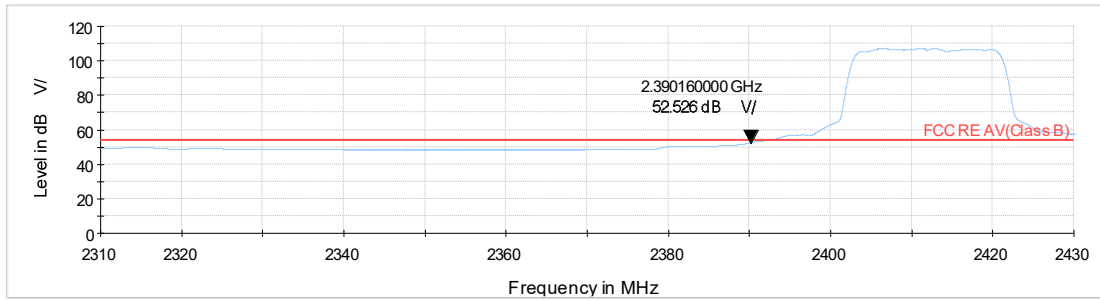
WiFi-2.4Gn20_CH1_2.31-2.43GHz_AV
