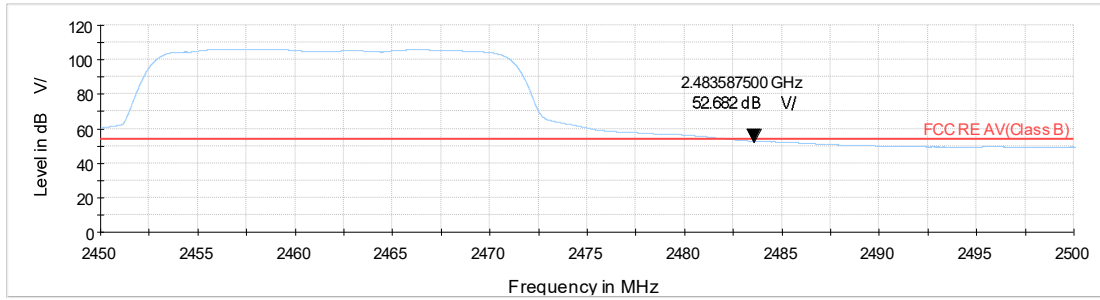
WiFi-2.4Gn20_CH11_2.45-2.5GHz_AV
