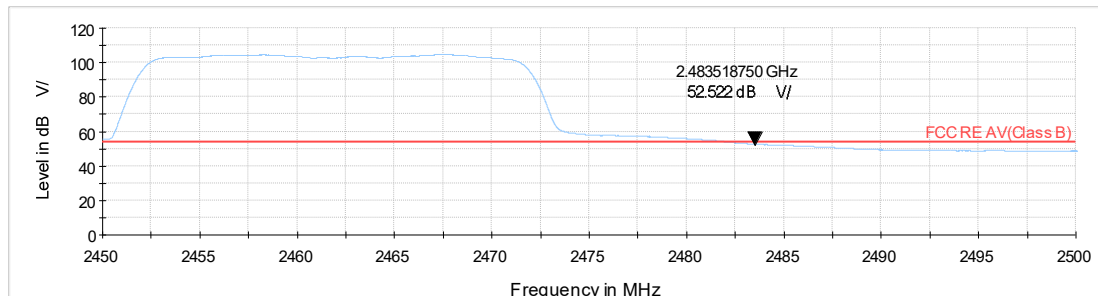
WiFi-2.4Gax20_CH11_2.45-2.5GHz_AV
