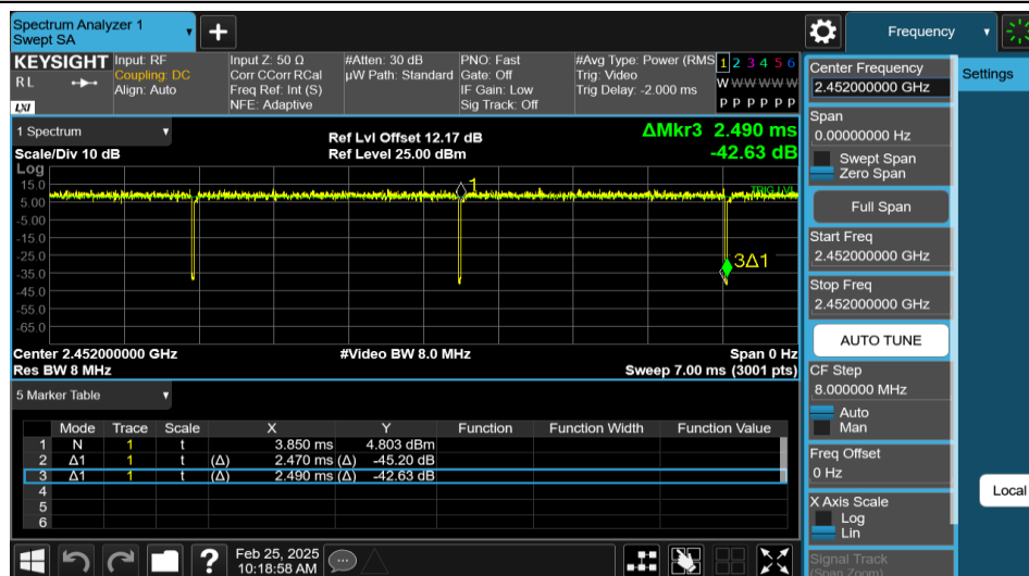
NTNV-11N40SISO-Ant1-2452
