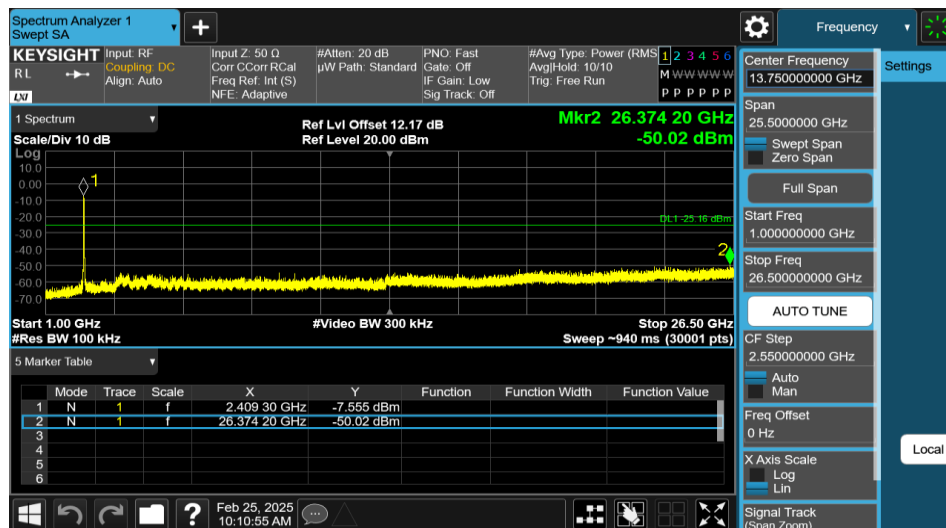
11N40SISO-Ant1-2422-1000~26500-PASS
