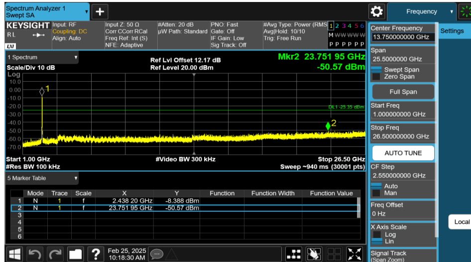
11N40SISO-Ant1-2437-1000~26500-PASS
