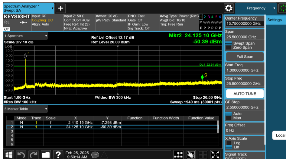
11N20SISO-Ant1-2412-1000~26500-PASS
