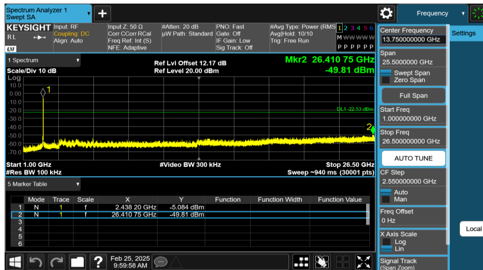
11N20SISO-Ant1-2437-1000~26500-PASS
