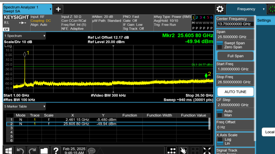
11G-Ant1-2462-1000~26500-PASS
