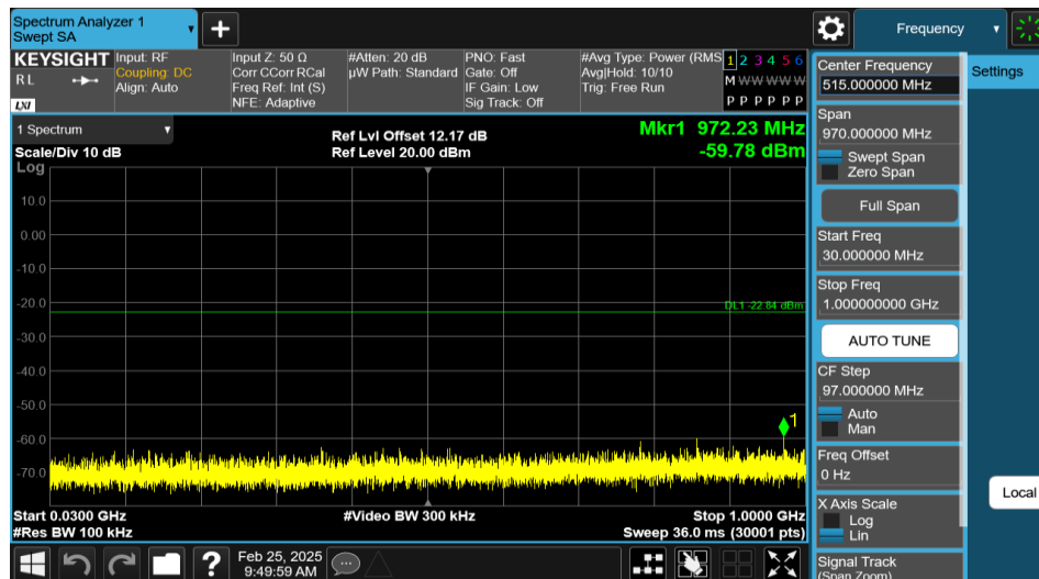
11N20SISO-Ant1-2412-30~1000-PASS
