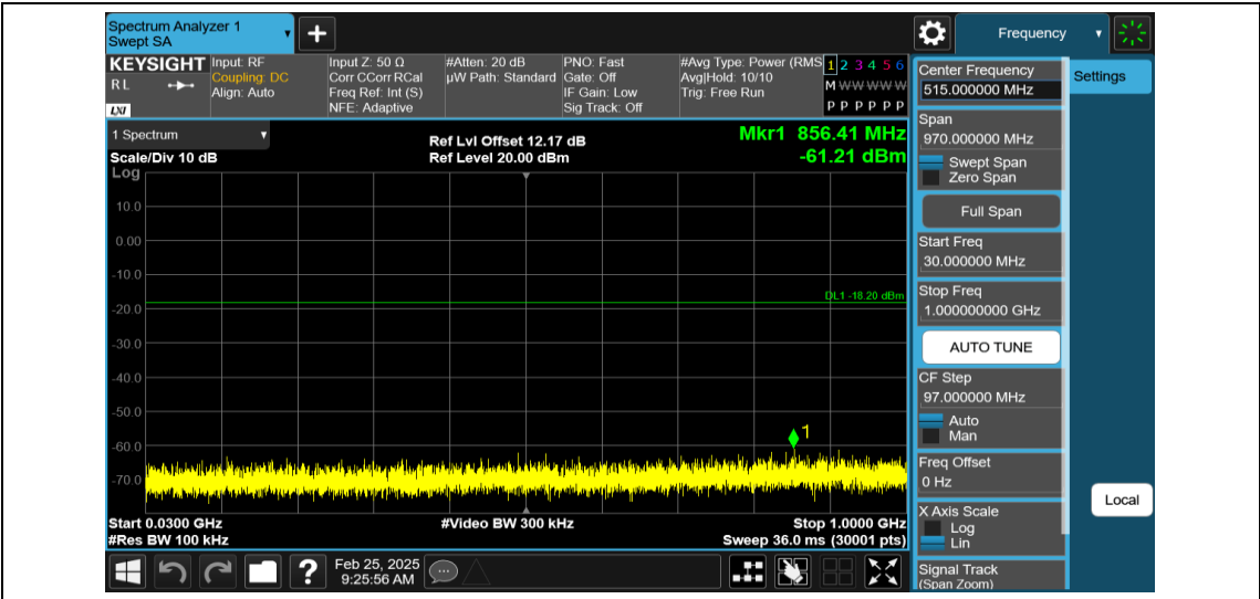
11B-Ant1-2412-30~1000-PASS
