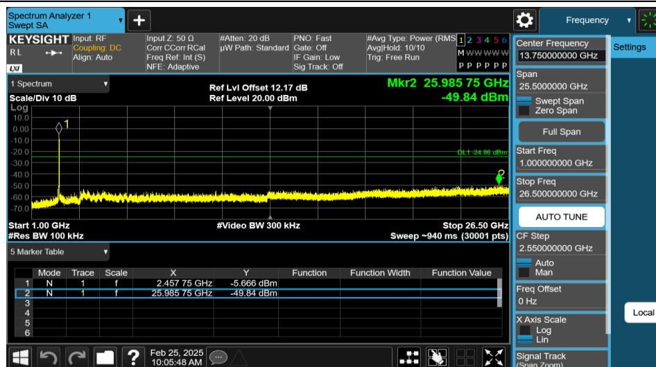
11N20SISO-Ant1-2462-1000~26500-PASS
