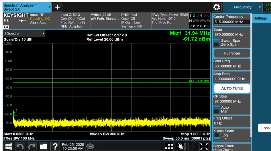
11N40SISO-Ant1-2452-30~1000-PASS
