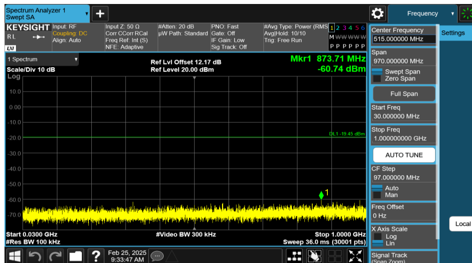
11B-Ant1-2462-30~1000-PASS
