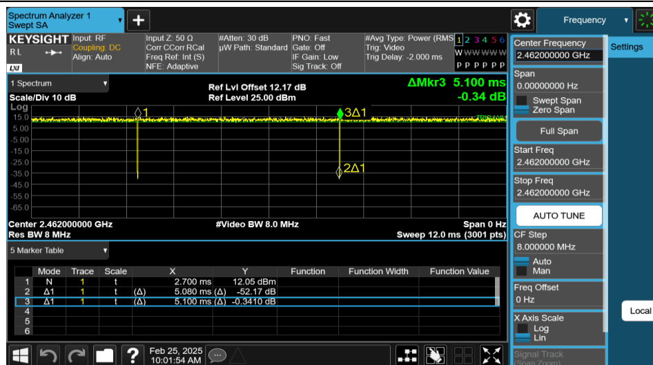
NTNV-11N20SISO-Ant1-2462
