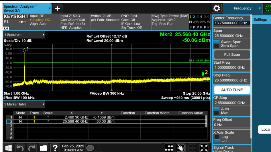
11B-Ant1-2462-1000~26500-PASS
