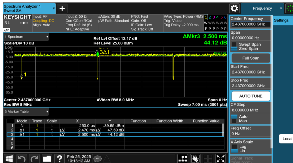
NTNV-11N40SISO-Ant1-2437
