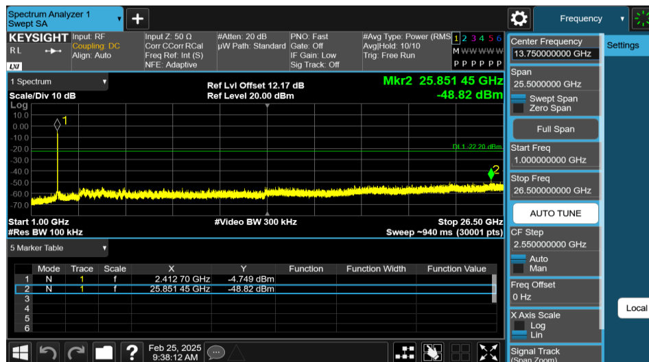
11G-Ant1-2412-1000~26500-PASS
