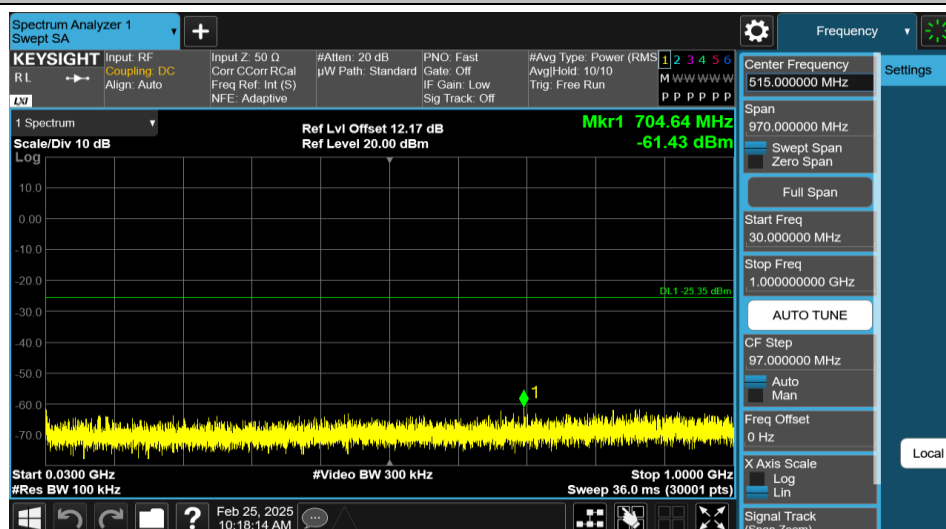
11N40SISO-Ant1-2437-30~1000-PASS
