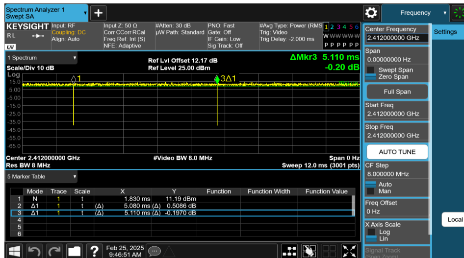
NTNV-11N20SISO-Ant1-2412
