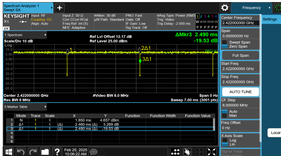
NTNV-11N40SISO-Ant1-2422
