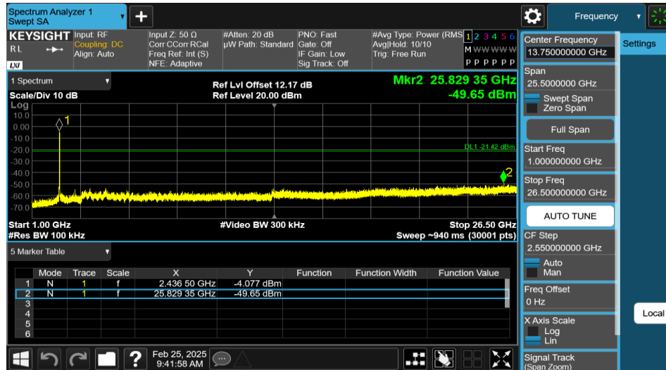
11G-Ant1-2437-1000~26500-PASS
