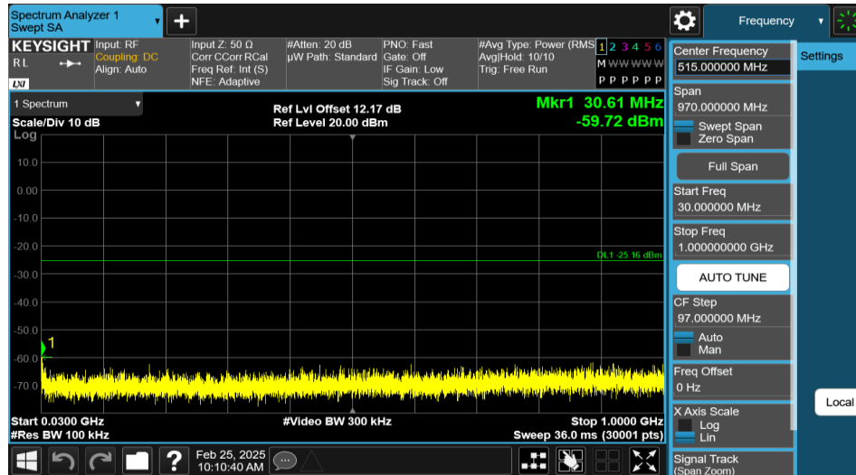
11N40SISO-Ant1-2422-30~1000-PASS
