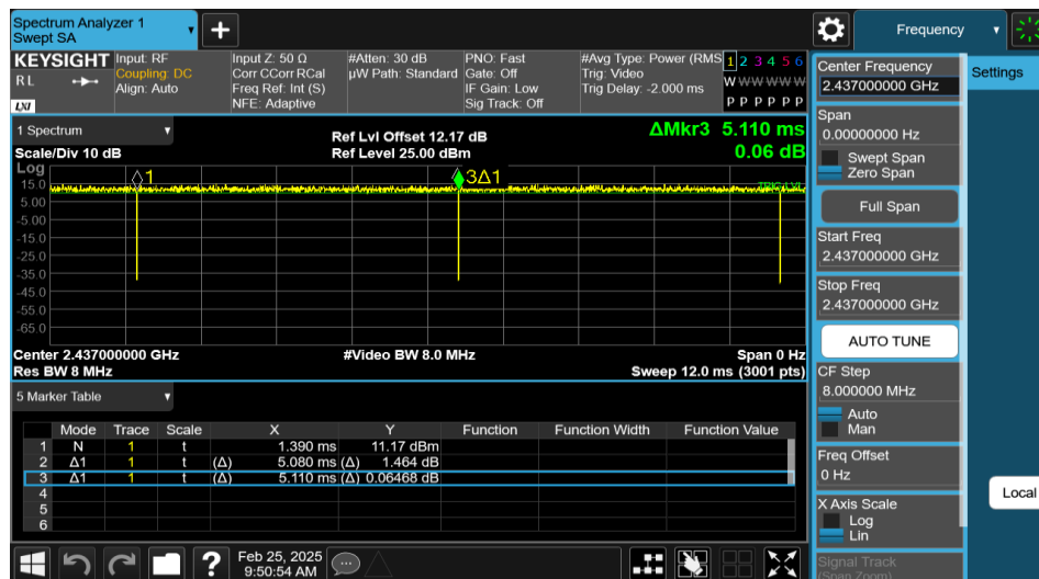
NTNV-11N20SISO-Ant1-2437
