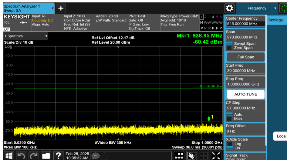
11N20SISO-Ant1-2462-30~1000-PASS
