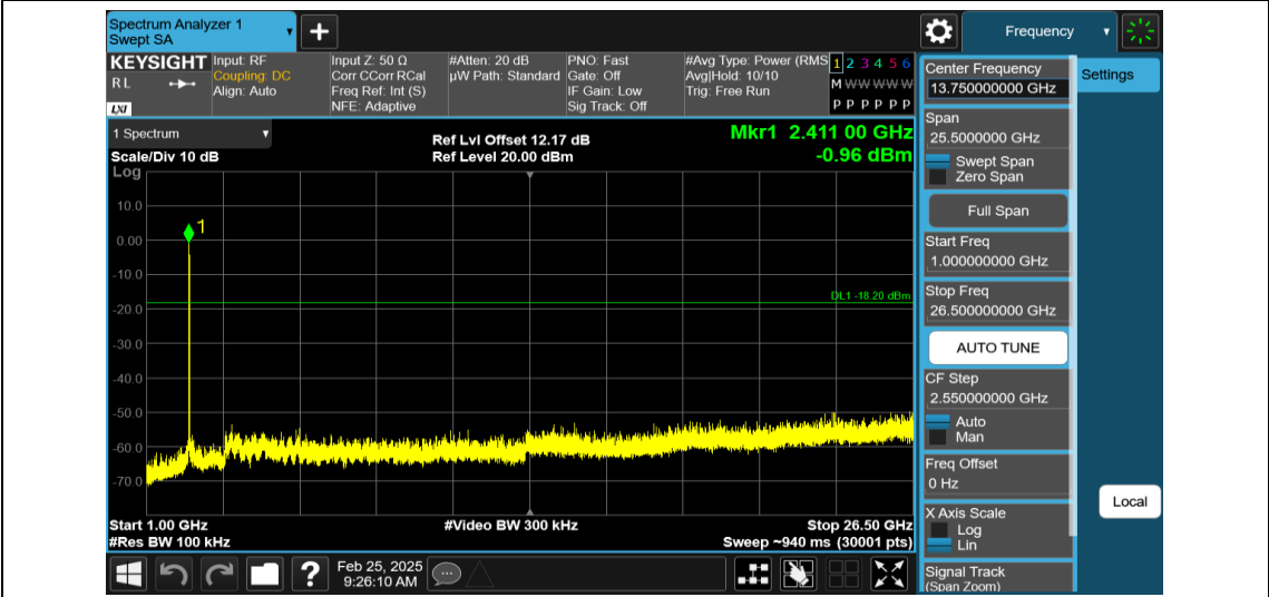
11B-Ant1-2412-1000~26500-PASS
